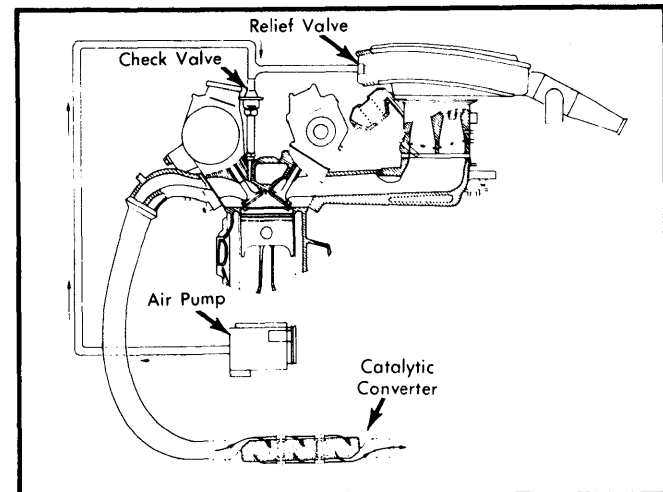
Fig. 2 Fiat Air Injection System (Brava and Spider 2000 Models)
