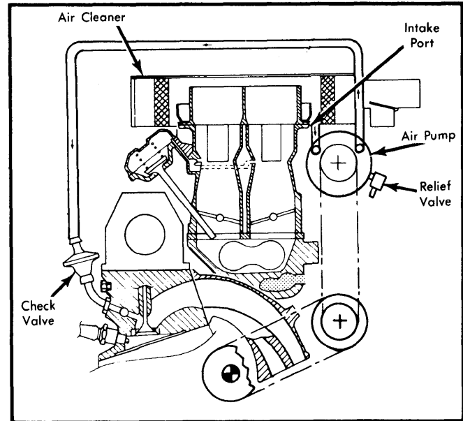
Fig. 1 Fiat Air Injection System (Strada and X1/9 Models)
