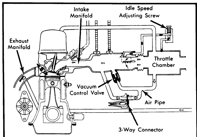
Fig. 1 200SX Intake Manifold Vacuum Control System
