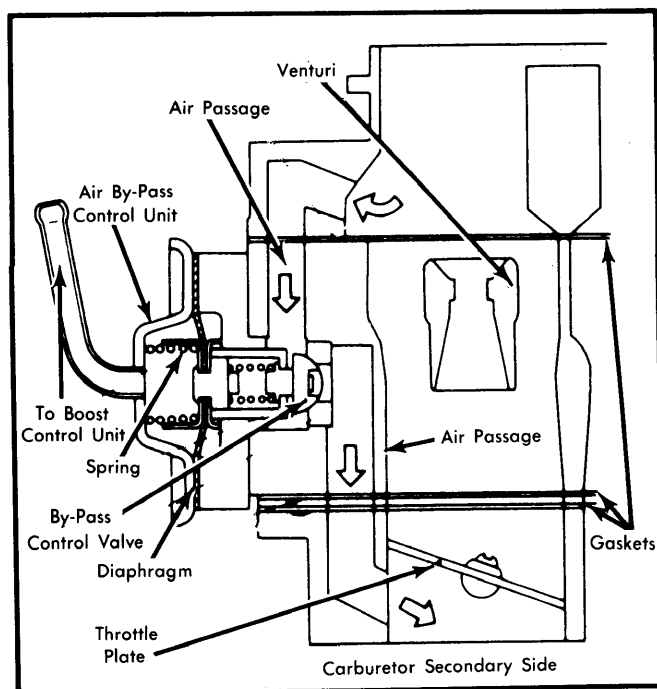
Fig. 3 Air By-Pass Control Unit Schematic
