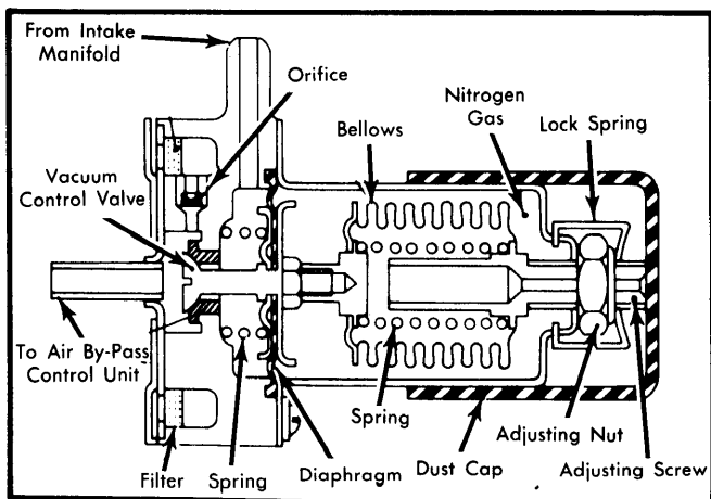
Fig. 2 510 And Pickup Boost Control Unit Schematic
