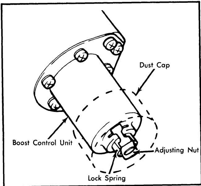
Fig. 4 Adjusting Boost Control Unit Operating Pressure
