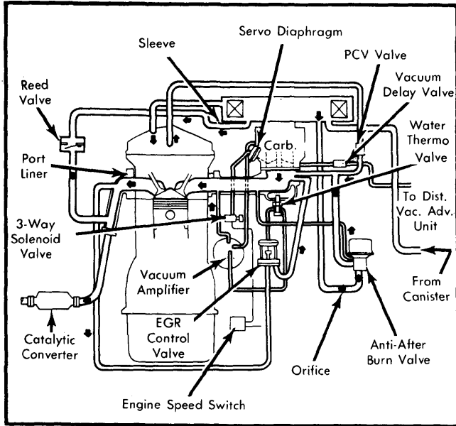
Fig. 1 2.0L; All Trans.; Federal Vacuum Diagram
