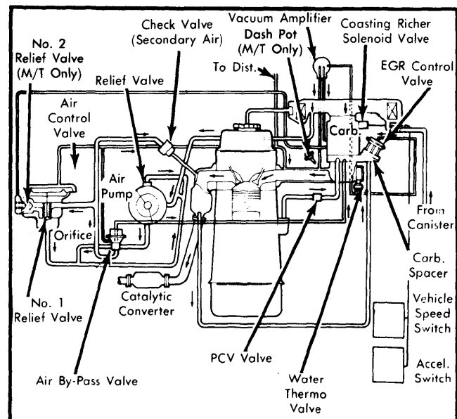
Fig. 4 2.3L; All Trans.; Calif. Vacuum Diagram
