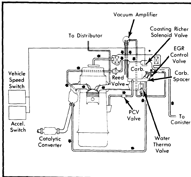
Fig. 3 2.3L; All Trans.; Federal Vacuum Diagram
