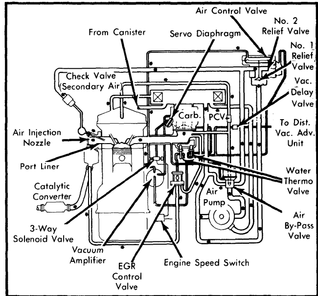
Fig. 2 2.0L; All Trans.; Calif. Vacuum Diagram
