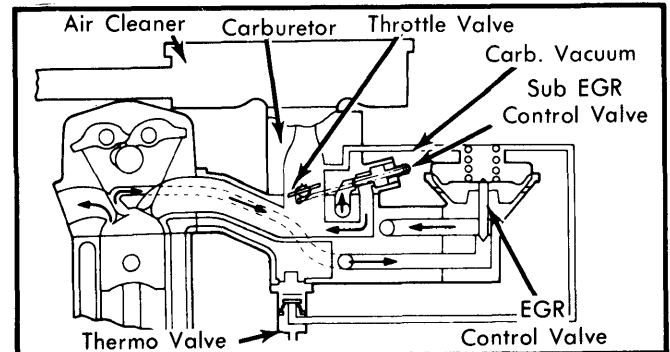
Fig. 1 Sectional View of EGR System (Federal Models)
