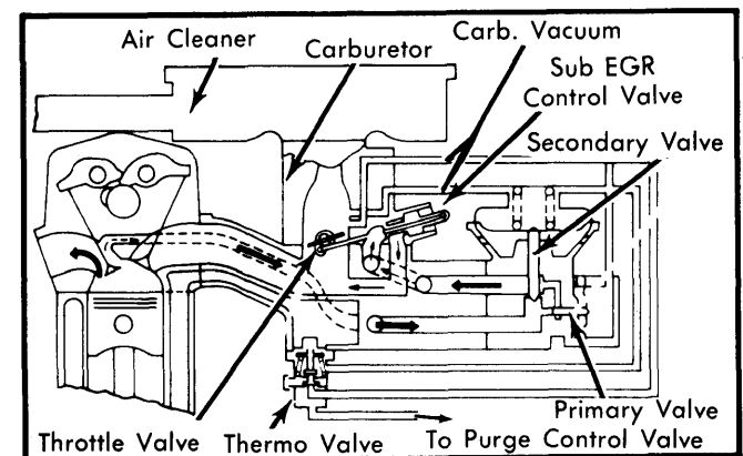
Fig. 2 Sectional View of EGR System (California Models)
