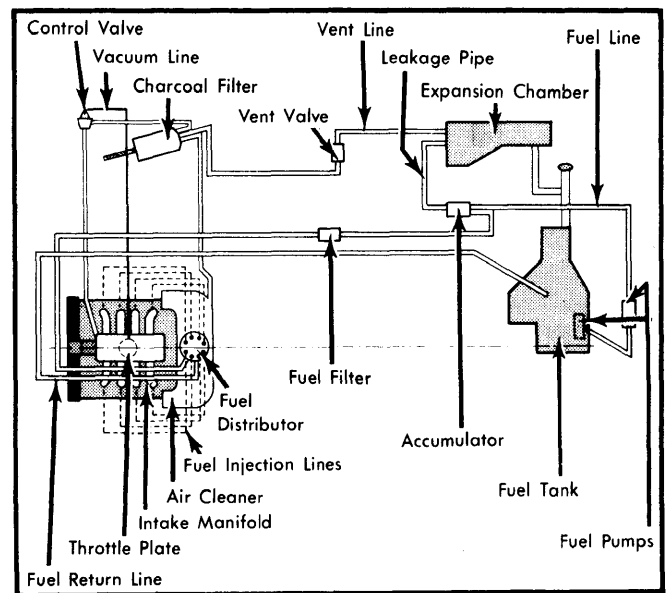
Fig. 2 Porsche 928 Fuel Evaporation System
