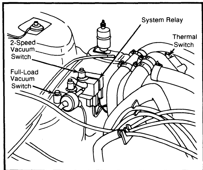
Fig. 15 Peugeot Enrichment Vacuum Switches
