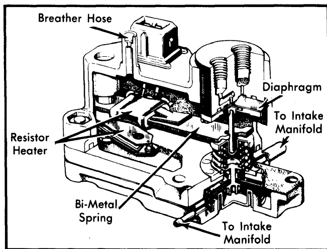
Fig. 2 Control Pressure Regulator (Pressure Compensated Model – Others Similar)
