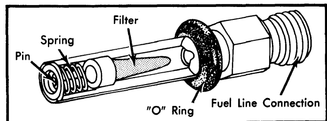
Fig. 3 Bosch CIS Lambda Injection Nozzle
