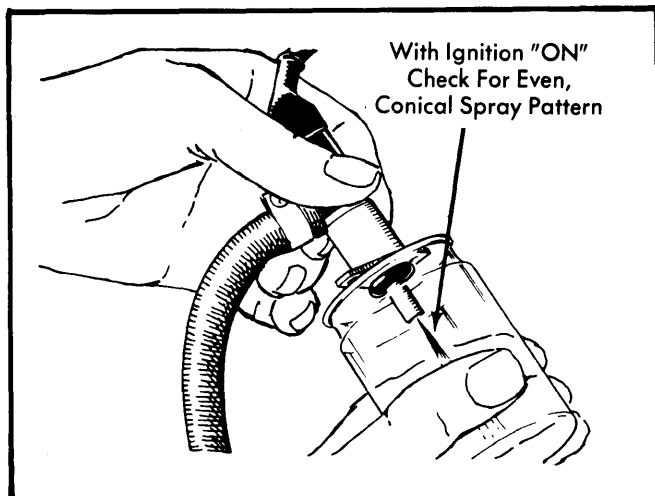
Fig. 11 Testing Cold Start Injector Valve
