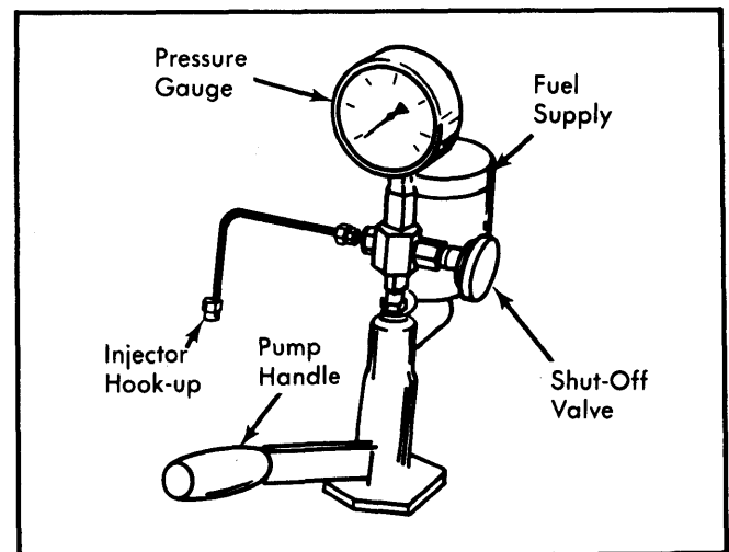
Fig. 12 Fuel Injector Tester
