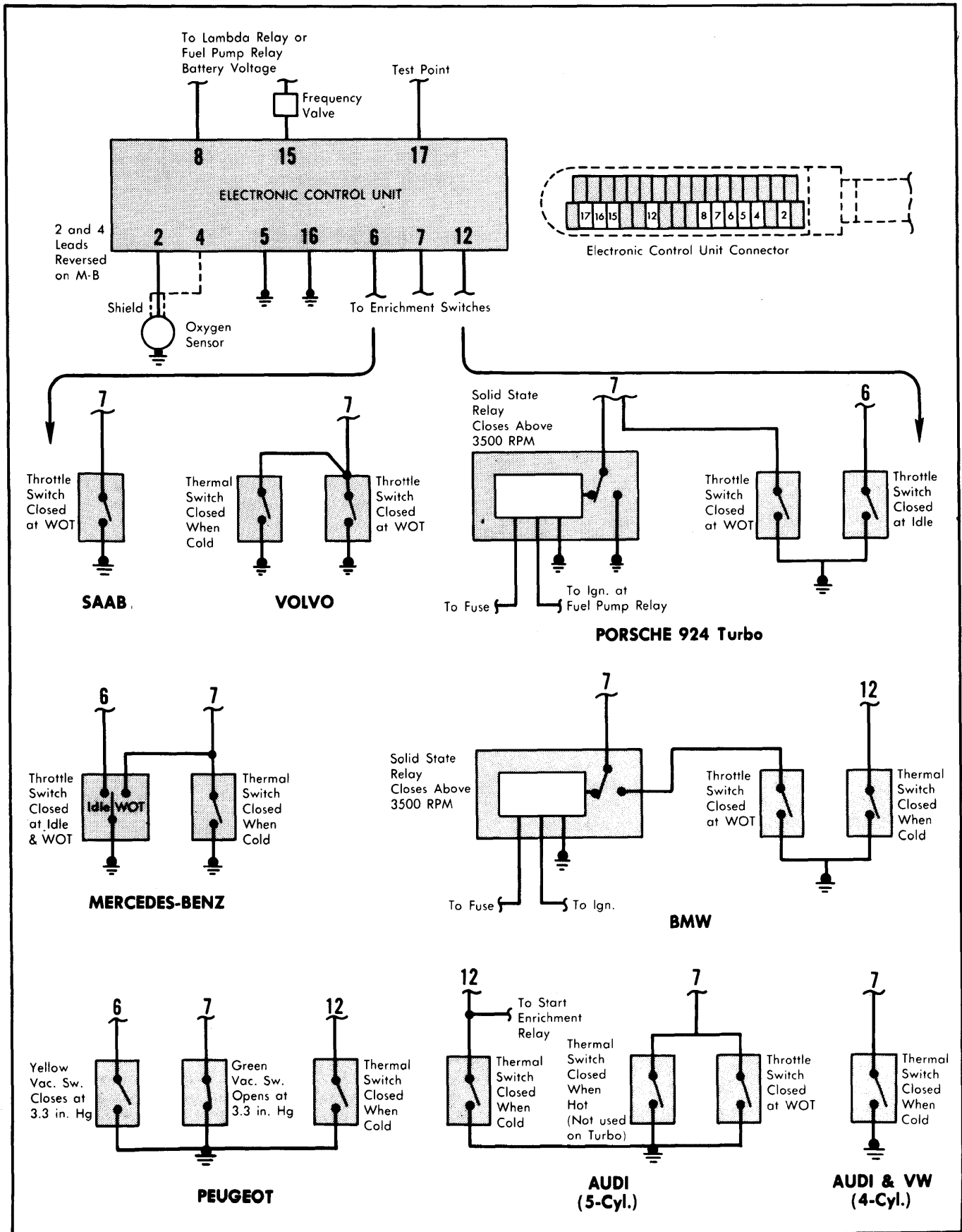
Fig. 14 Bosch CIS Lambda Electronic Control Unit Wiring Diagram Copyright (c) 2001 Mitchell Repair Information Company
