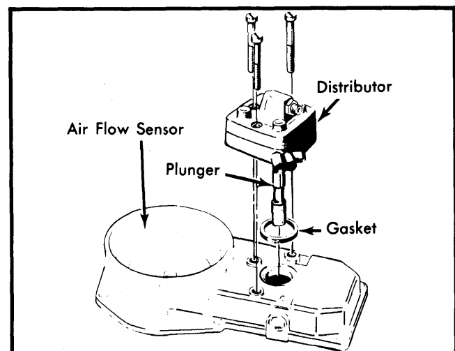
Fig. 8 Checking Fuel Distributor Plunger
