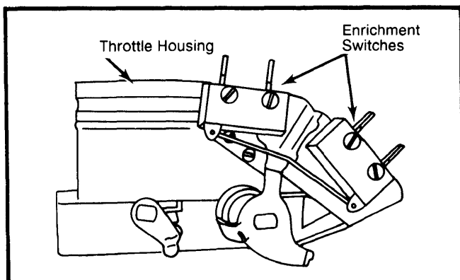
Fig. 16 Throttle Enrichment Switches (Porsche 924 Turbo Shown)
