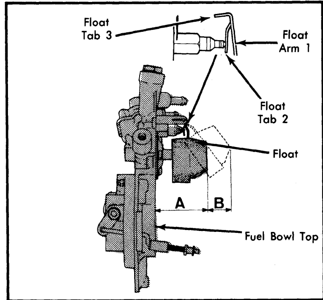
Fig. 1 Float Level and Drop (Travel) Adjustment (California Models)
