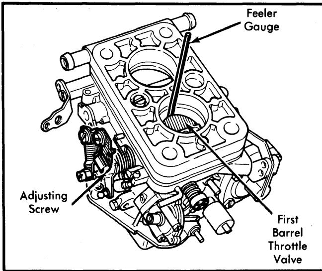
Fig. 3 Initial Throttle Valve Opening Adjustment (California Model Shown)
