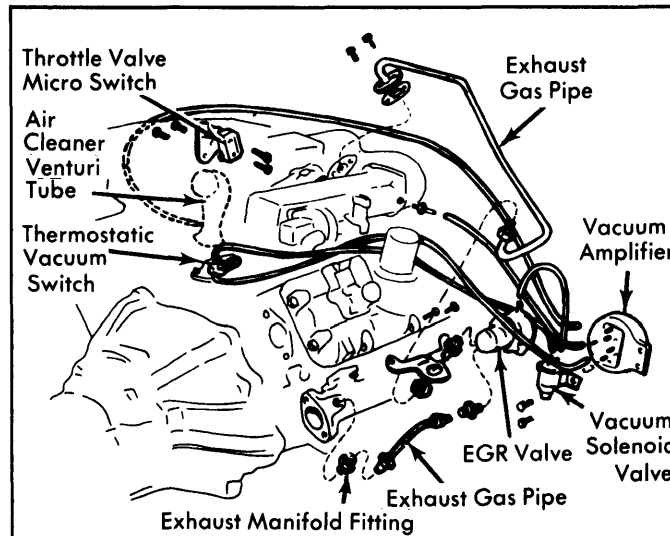
Fig. 6: 1976-78 260 Series Exhaust Gas Recirculation System
