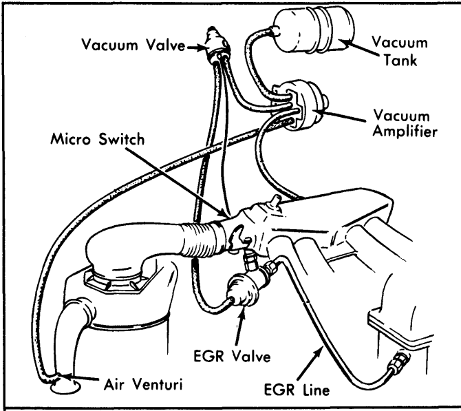
Fig. 4: 1974-75 240 Series Exhaust Gas Recirculation System
