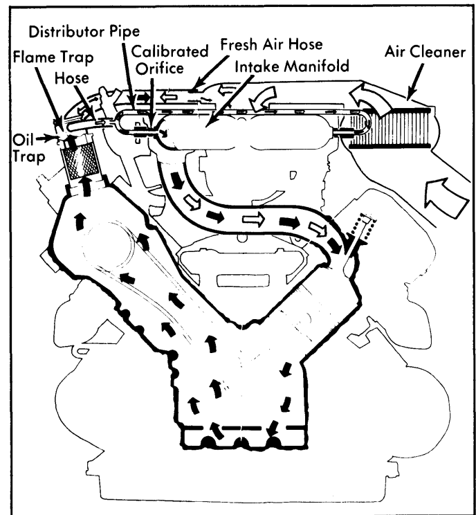
Fig. 8: 1976-78 260 Series Positive Crankcase Ventilation System
