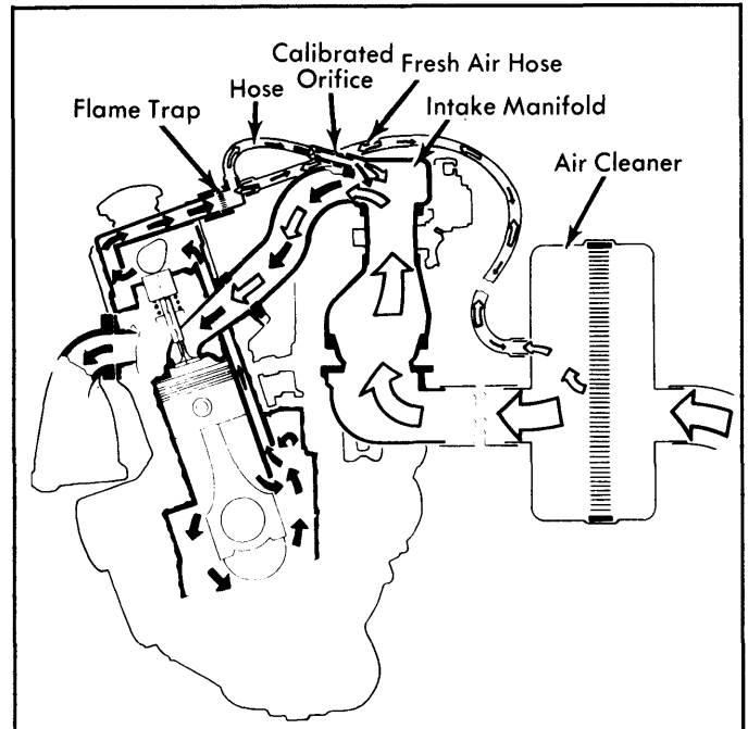
Fig. 7: 1976-78 240 Series Positive Crankcase Ventilation System
