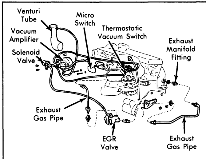
Fig. 5: 1976-78 240 Series Exhaust Gas Recirculation System
