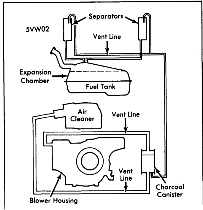
Fig. 12: 1975-76 Type 2 Fuel Evaporation System
