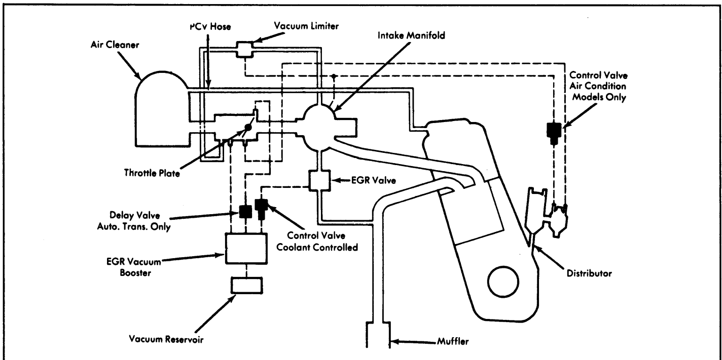
Fig. 19: 1977-78 Dasher Exhaust Emission System
