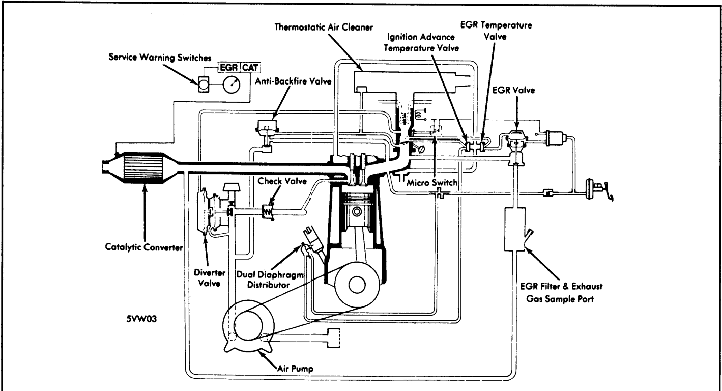
Fig. 7: 1975 Dasher, Rabbit & Scirocco Exhaust Emission System
