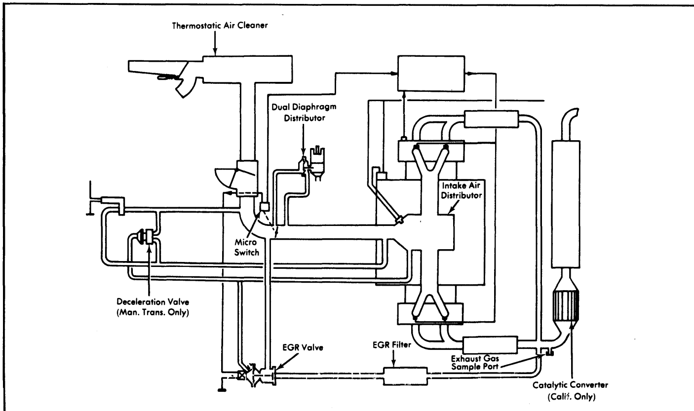
Fig. 8: 1975-76 Type 1 & Thing Exhaust Emission System
