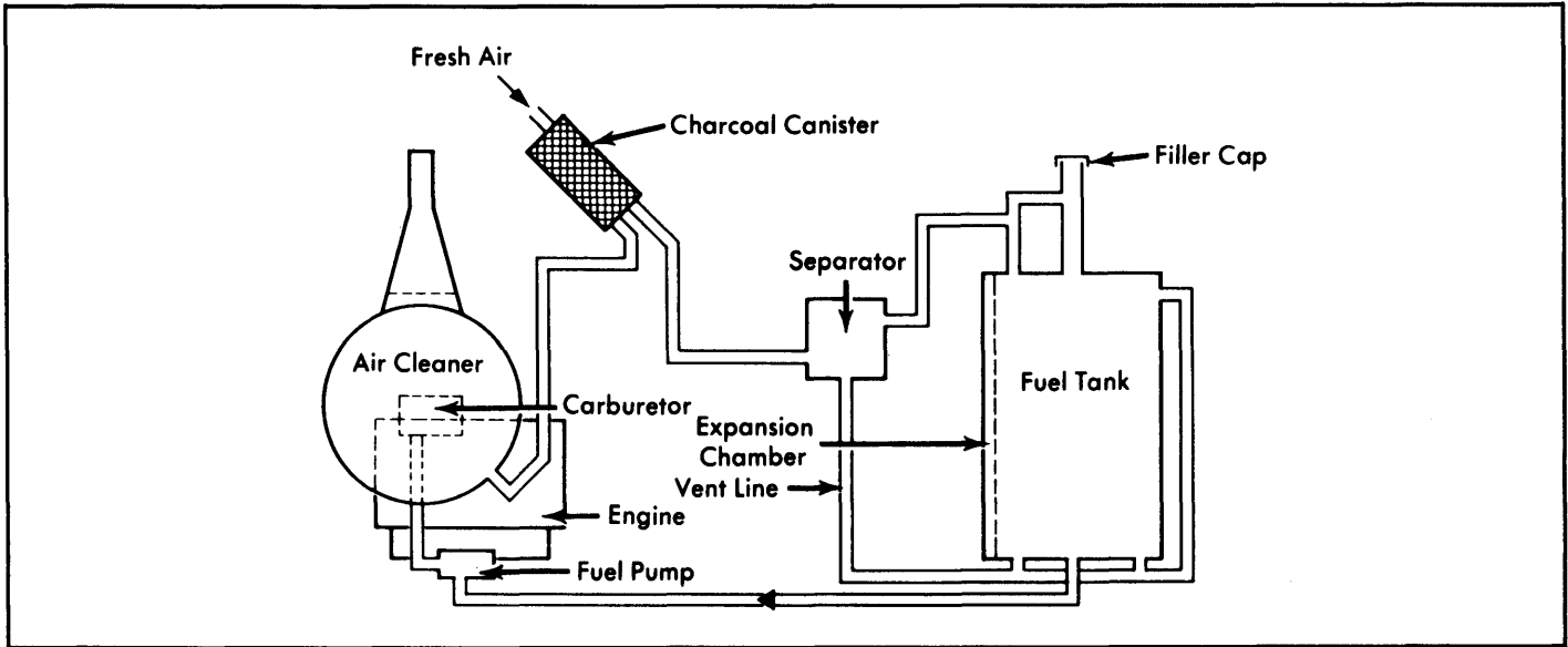
Fig. 10: 1975-76 Rabbit & Scirocco Fuel Evaporation System
