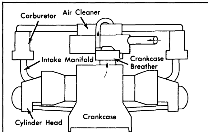
Fig. 3: 1974 Type 2 Positive Crankcase Ventilation System
