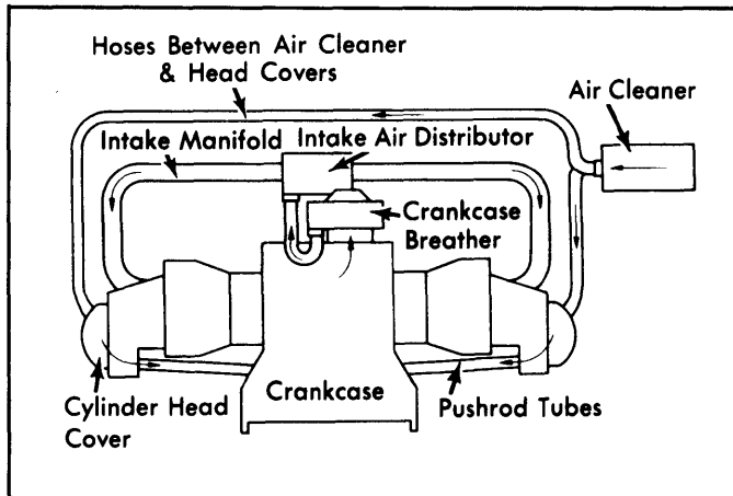
Fig. 2: 1974 Positive Crankcase Ventilation System (Fuel Injected)
