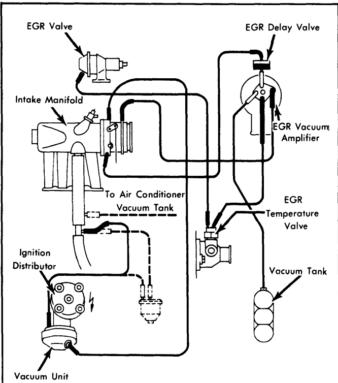
Fig. 28: 1979 Dasher Exhaust Emission System (Federal & California Auto. Trans.)
