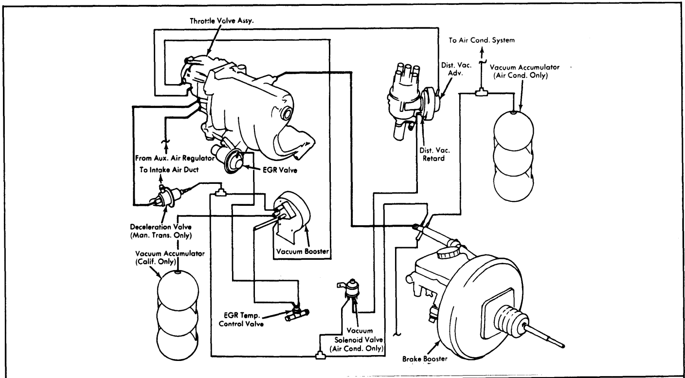
Fig. 14: 1976 Dasher Exhaust Emission System
