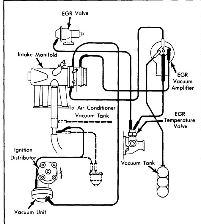
Fig. 30: 1979 Dasher Exhaust Emission System (California Man. Trans.)
