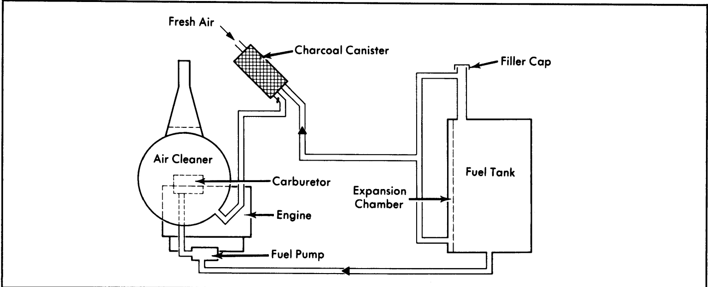
Fig. 6: 1974-75 Dasher Fuel Evaporation System
