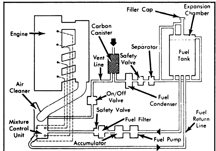
Fig. 25: 1978 Rabbit & Scirocco Fuel Evaporation System
