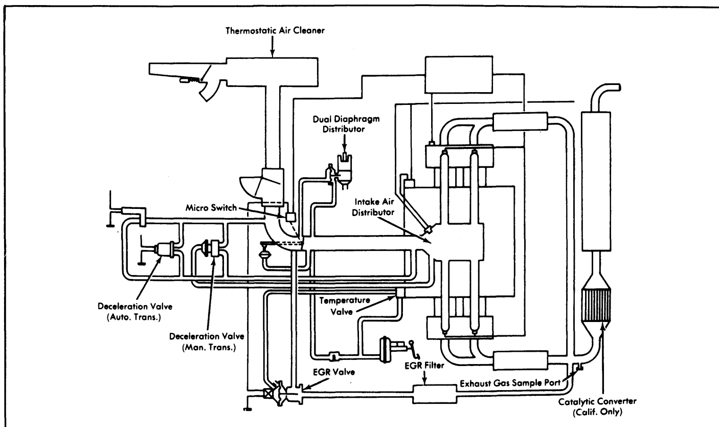
Fig. 9: 1975-76 Type 2 Exhaust Emission System
