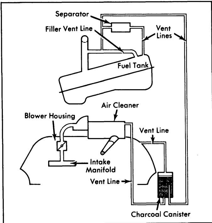
Fig. 11: 1975-76 Type 1 Fuel Evaporation System
