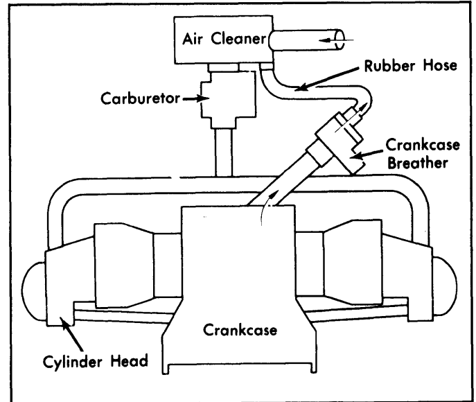
Fig. 4: 1974 Type 1, 4 & Thing Positive Crankcase Ventilation System
