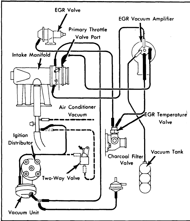
Fig. 27: 1979 Rabbit & Scirocco Exhaust Emission System (California Man. Trans.)
