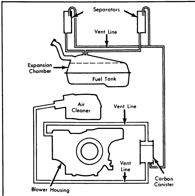
Fig. 23: 1978 Type 2 Fuel Evaporation System
