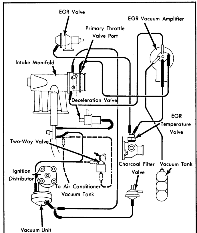
Fig. 26: 1979 Rabbit & Scirocco Exhaust Emission System (Federal Man. Trans.)
