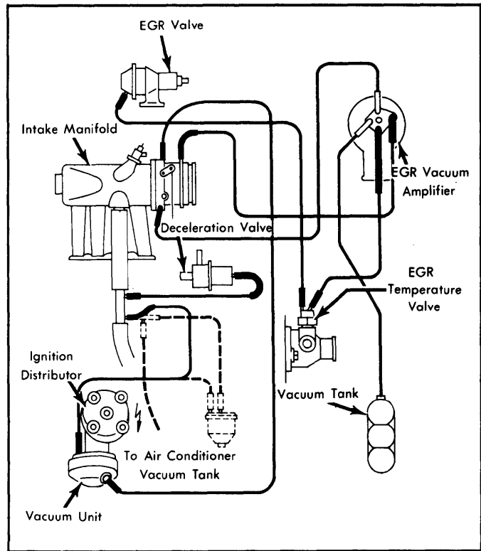
Fig. 29: 1979 Dasher Exhaust Emission System (All Except California Man. Trans.)
