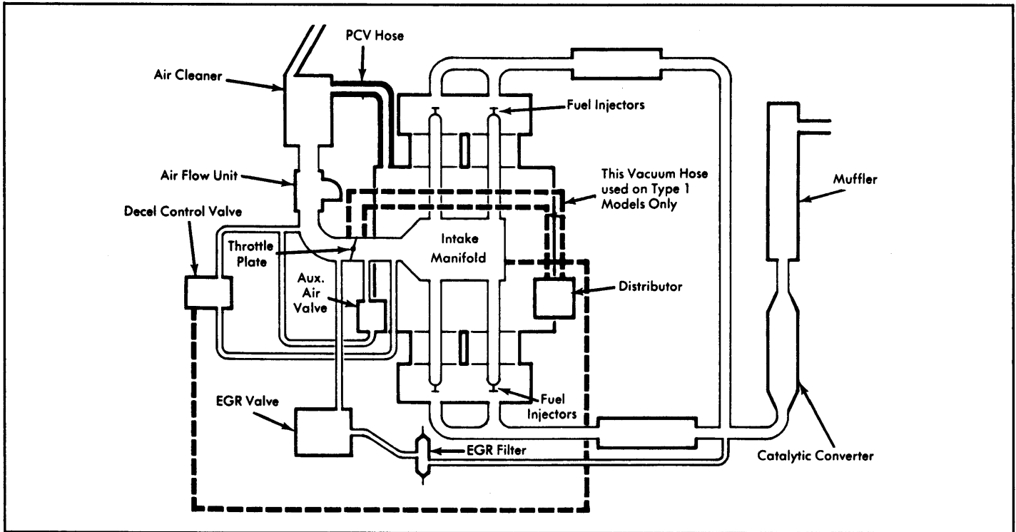
Fig. 18: 1977-78 Type 1 & 2 Exhaust Emission System
