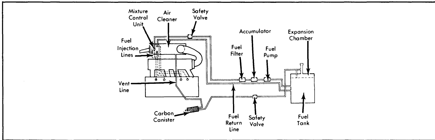
Fig. 17: 1976-78 Dasher Fuel Evaporation System
