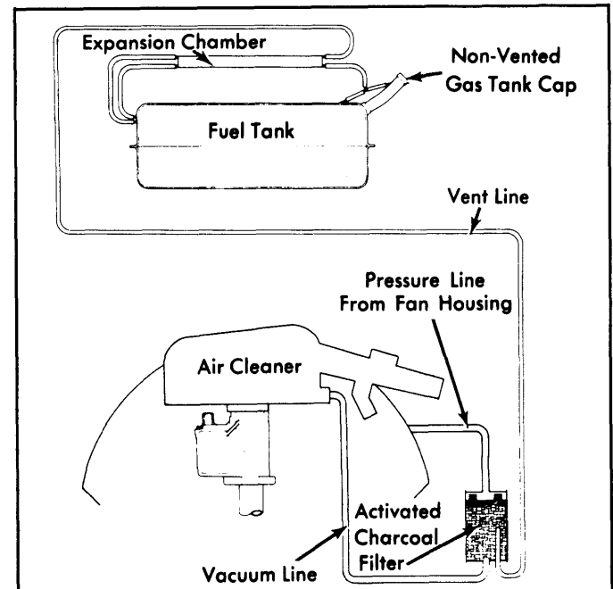
Fig. 5: 1974-75 Fuel Evaporation System (Except Dasher)
