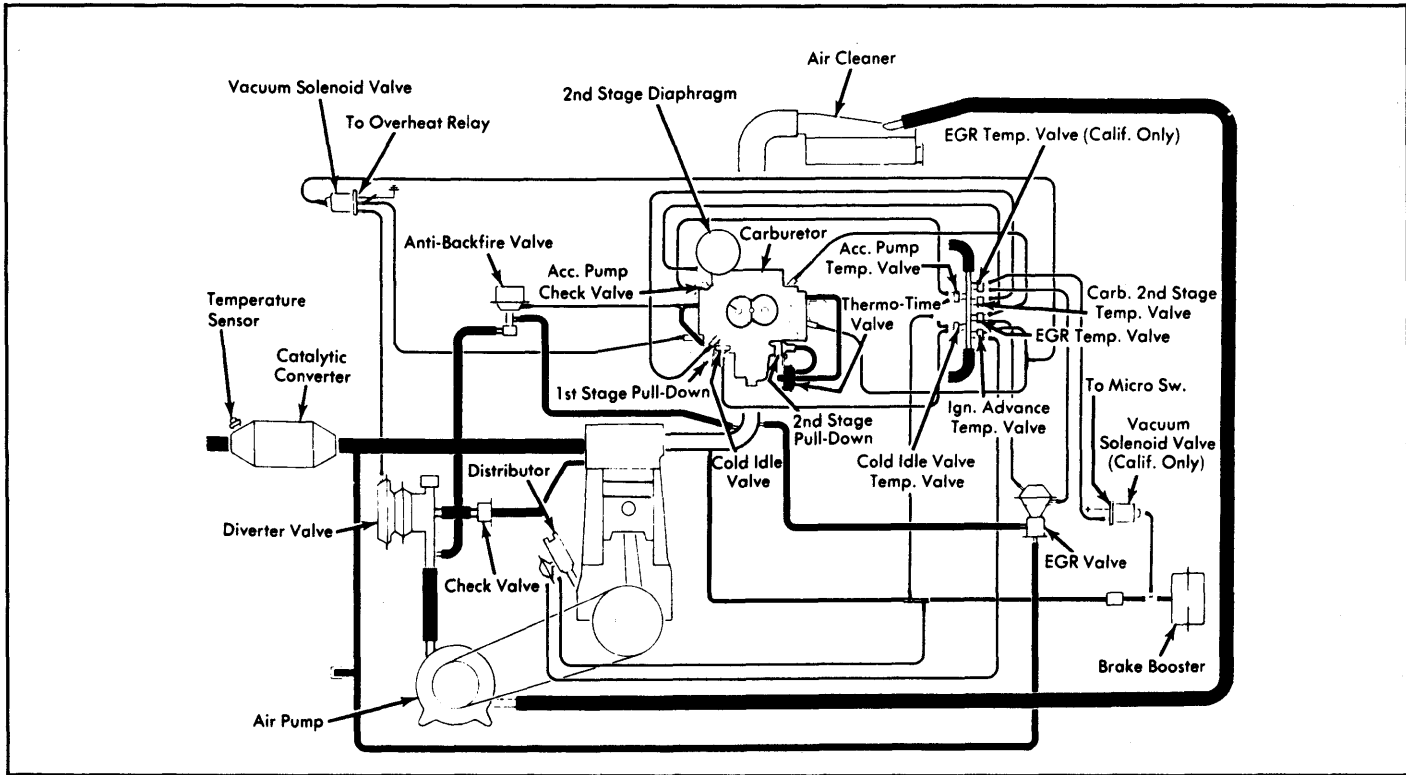
Fig. 16: 1976 Rabbit & Scirocco Exhaust Emission System
