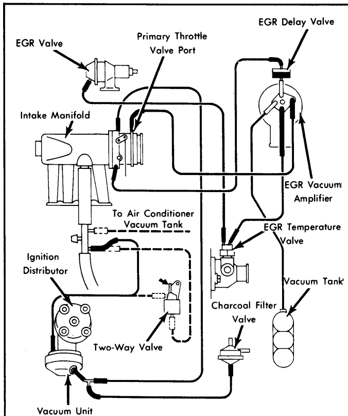
Fig. 24: 1979 Rabbit & Scirocco Exhaust Emission System (Federal & California Auto. Trans.)
