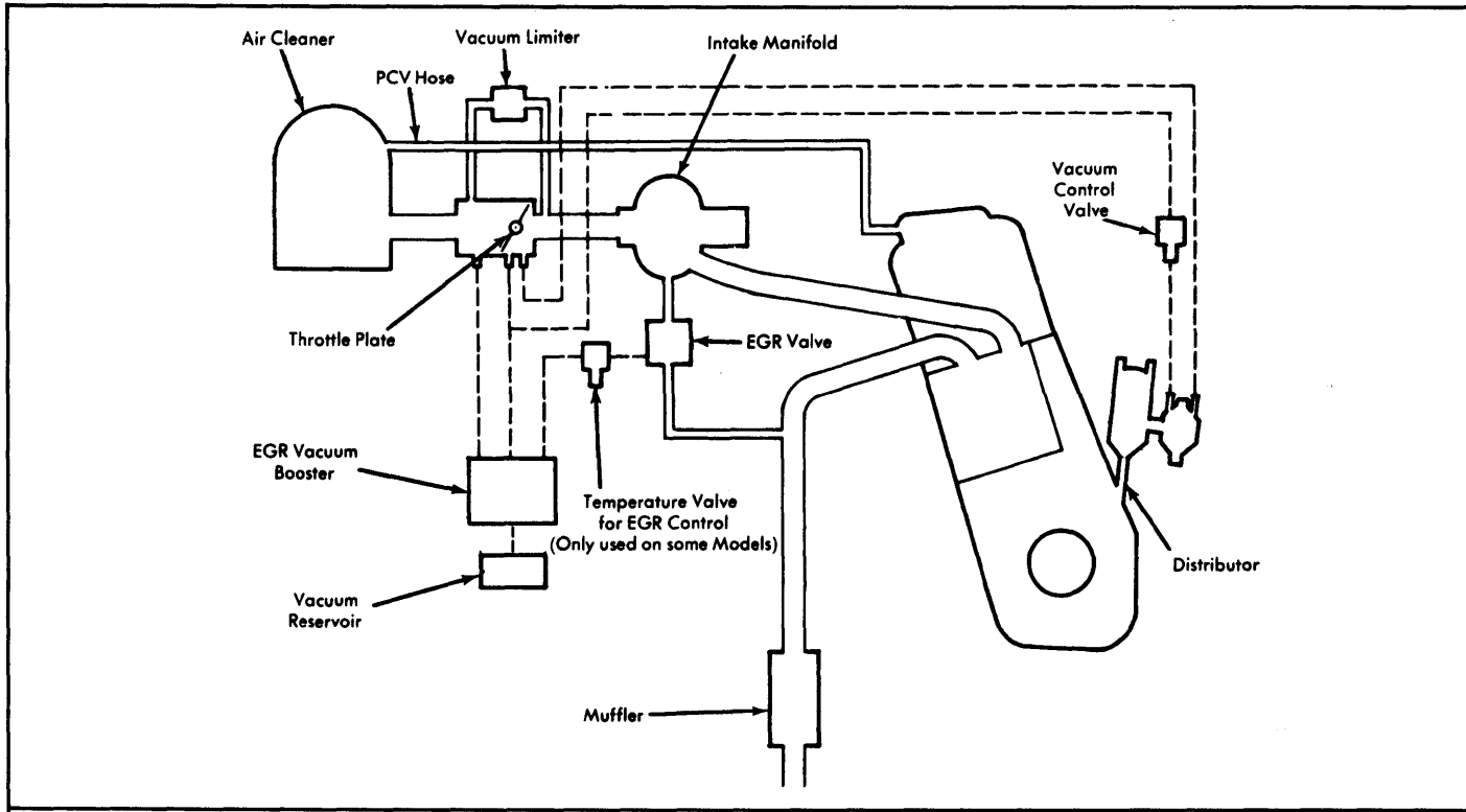
Fig. 20: 1977-78 Rabbit & Scirocco Exhaust Emission System
