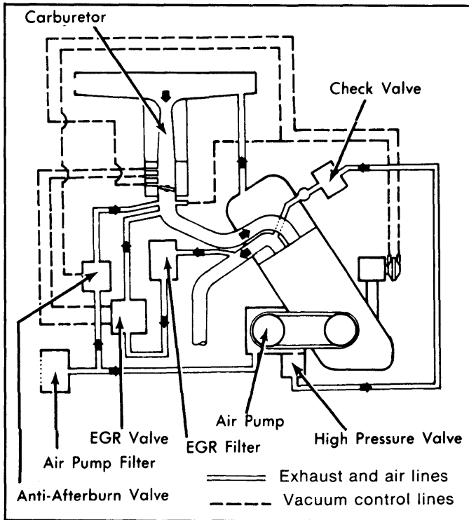
Fig. 1: 1974 Dasher Exhaust Emission System
