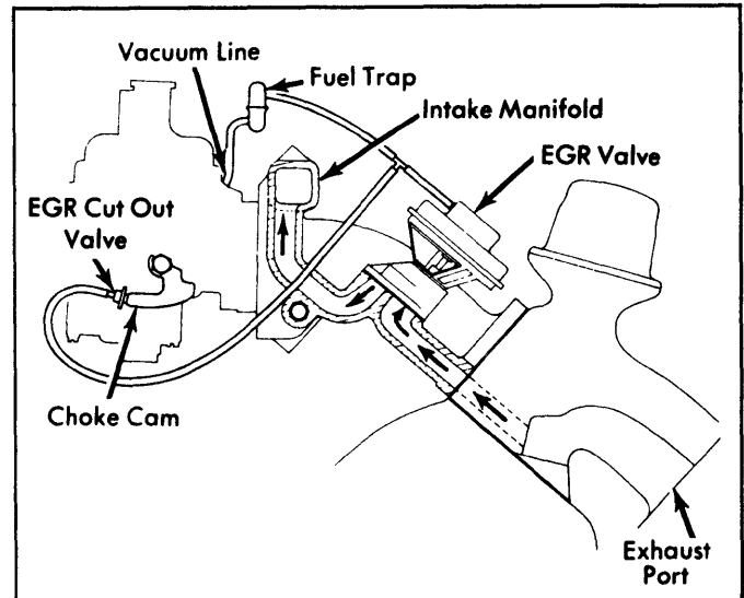
Fig. 9: 1977 TR7 Exhaust Gas Recirculation System
