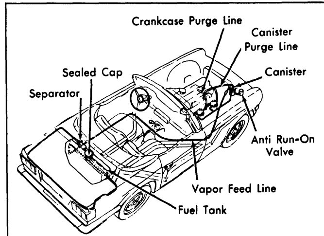
Fig. 7: 1975-78 TR6 Fuel Evaporation System
