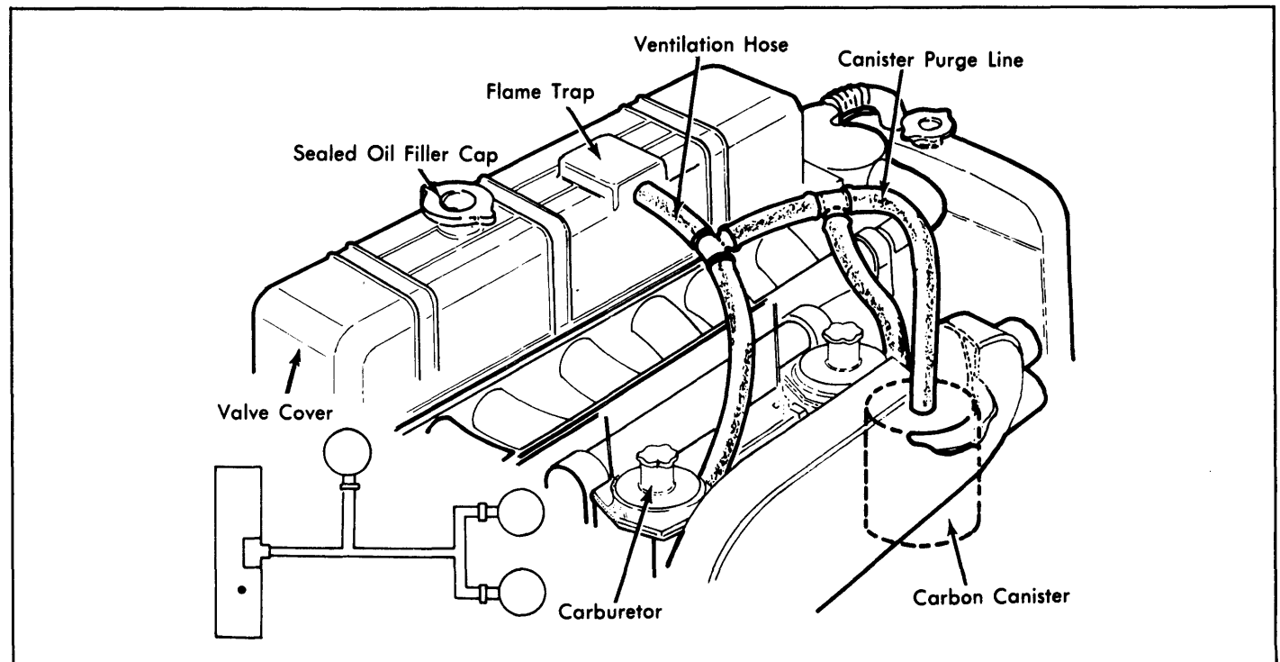
Fig. 3: 1974-78 Positive Crankcase Ventilation System (Typical)
