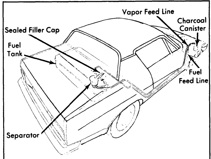
Fig. 8: 1975-78 TR7 Fuel Evaporation System
