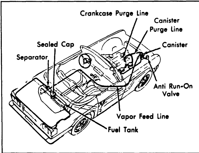
Fig. 5: 1974 TR6 Fuel Evaporation System
