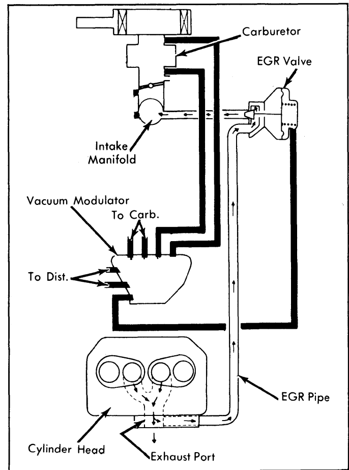
Fig. 22: 1978 Exhaust Gas Recirculation System
