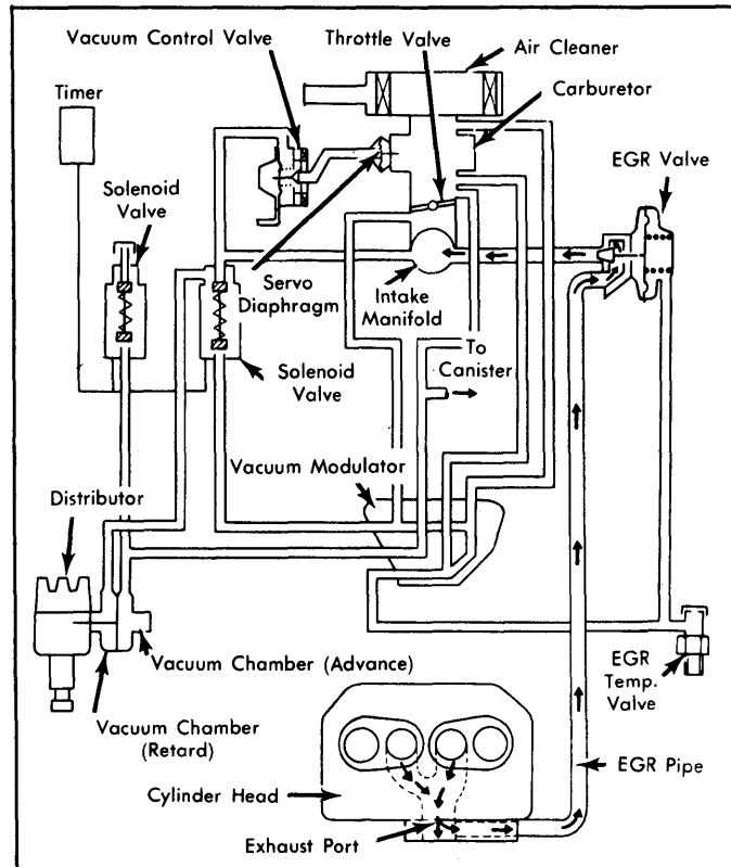
Fig. 24: 1979 Exhaust Emission System (California With Man. Trans., Except 4WD)
