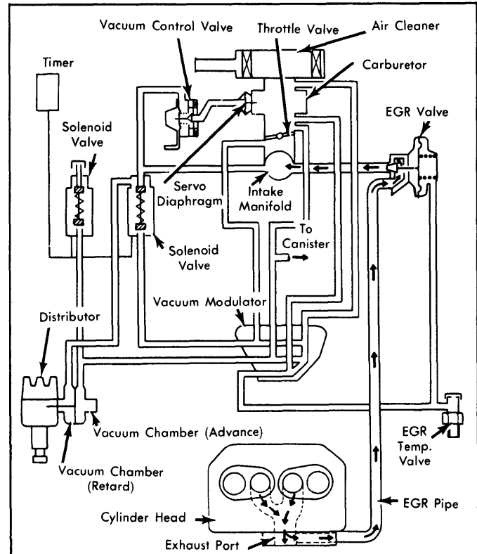
Fig. 26: 1979 Exhaust Emission System (California 4WD)
