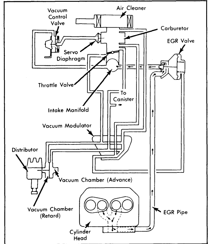
Fig. 21: 1977-79 Exhaust Emission System (Federal 4WD)
