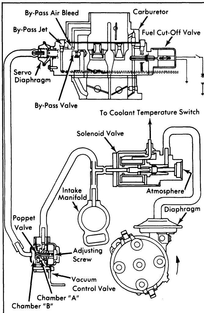
Fig. 6: 1975 Exhaust Emission System (Federal Auto. Trans. & California Man. Trans.)
