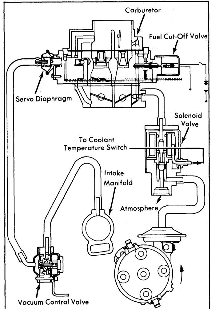
Fig. 7: 1975 Exhaust Emission System (Federal Man. Trans.)
