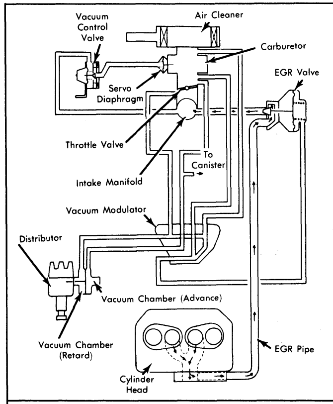
Fig. 20: 1977-79 Exhaust Emission System (Federal With Man. Trans., Except 4WD)
