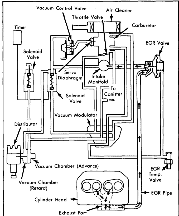
Fig. 25: 1979 Exhaust Emission System (California With Auto. Trans., Except 4WD)
