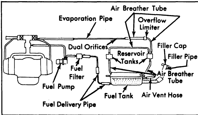
Fig. 5: 1974-76 Fuel Evaporation System (Station Wagon)
