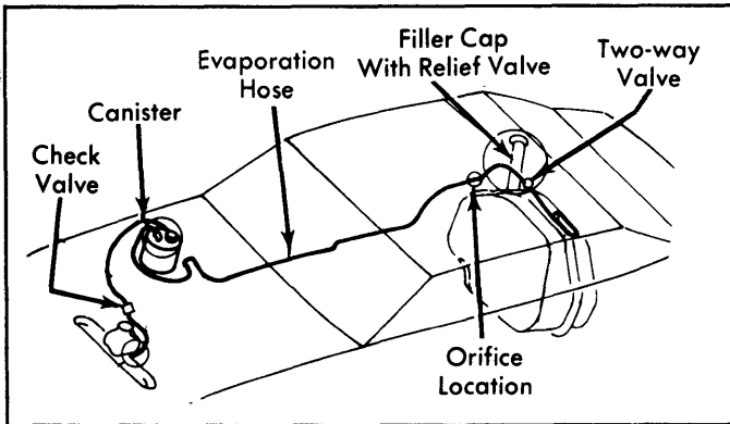
Fig. 18: 1977-78 Fuel Evaporation System (Sedan, Coupe & Hardtop)
