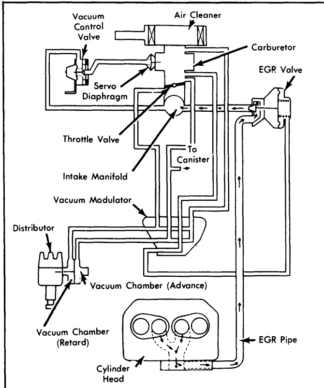
Fig. 23: 1979 Exhaust Emission System (Federal With Auto. Trans., Except 4WD)
