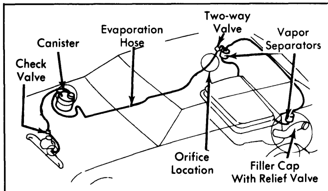
Fig. 19: 1977-78 Fuel Evaporation System (Station Wagon & 4WD)
