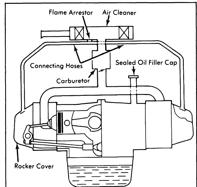
Fig. 8: 1975-78 Positive Crankcase Ventilation System
