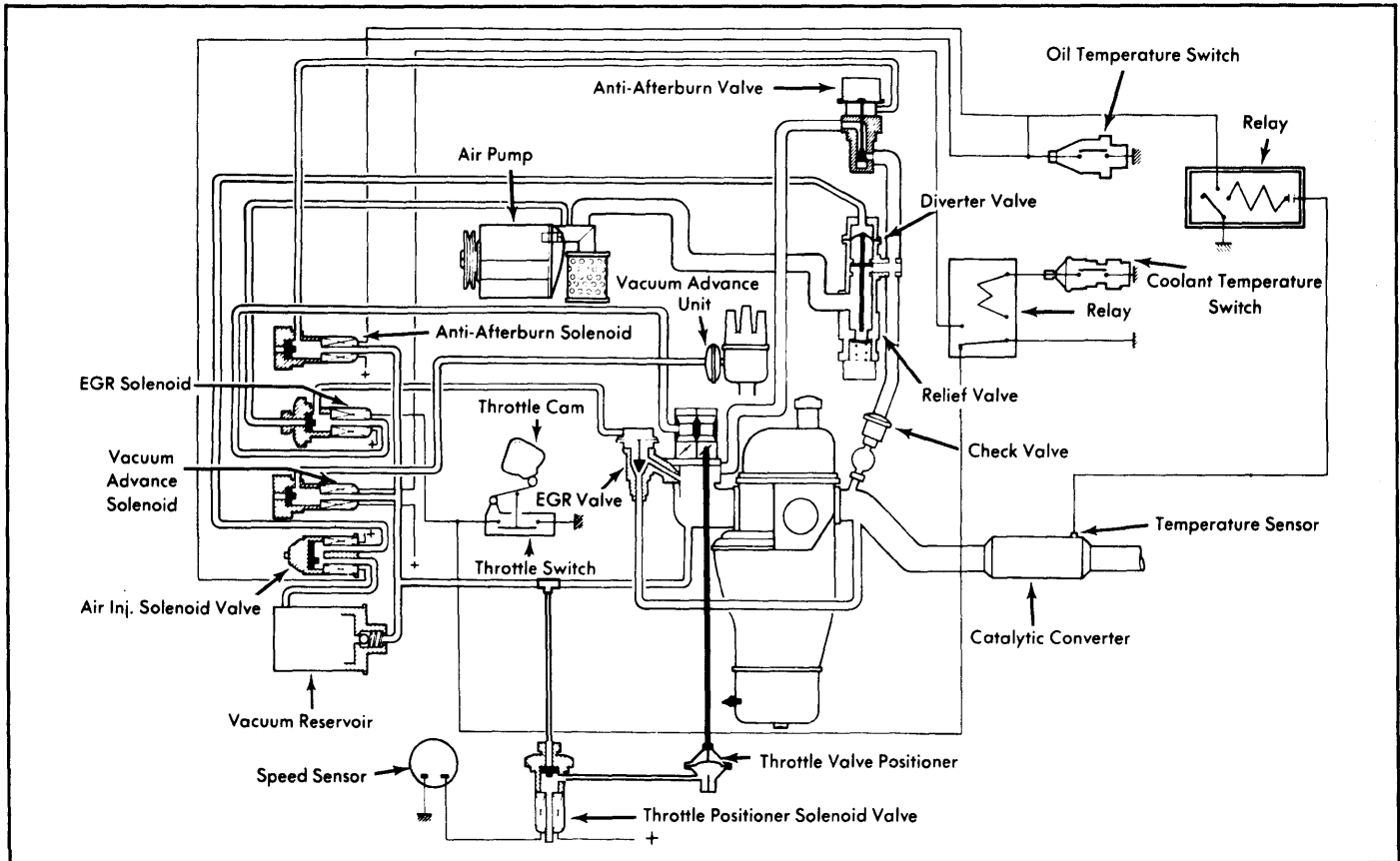
Fig. 8: 1976 Exhaust Emission System (Carburetor Models Except R-5)
