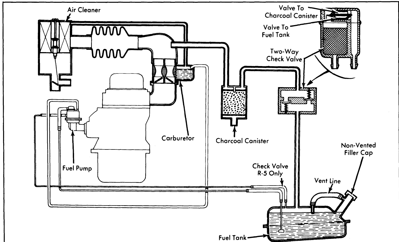
Fig. 9: 1976-78 R-5 Fuel Evaporation System (Typical)
