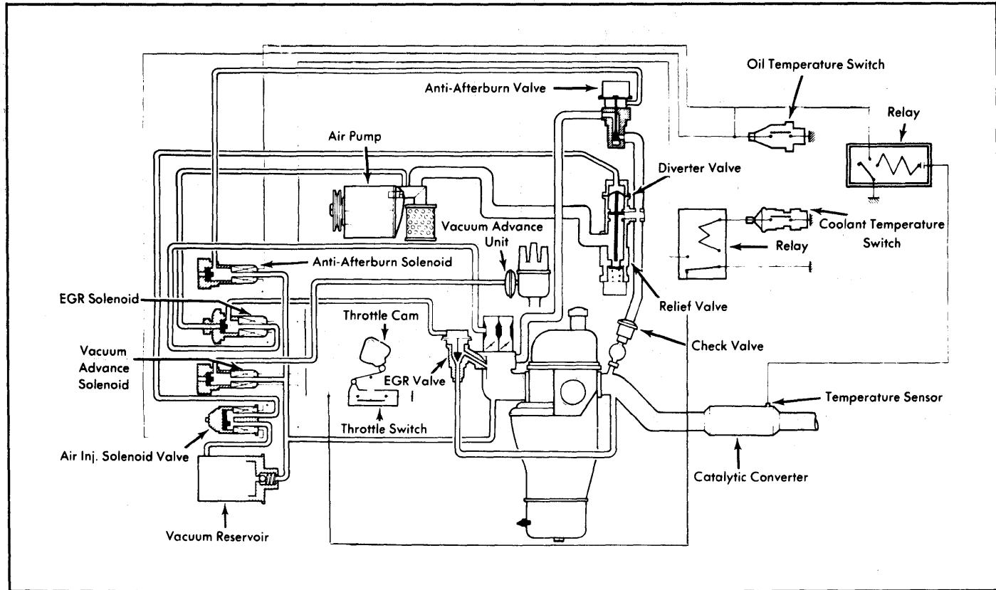
Fig. 2: 1975 Exhaust Emission System (Carbureted Models)
