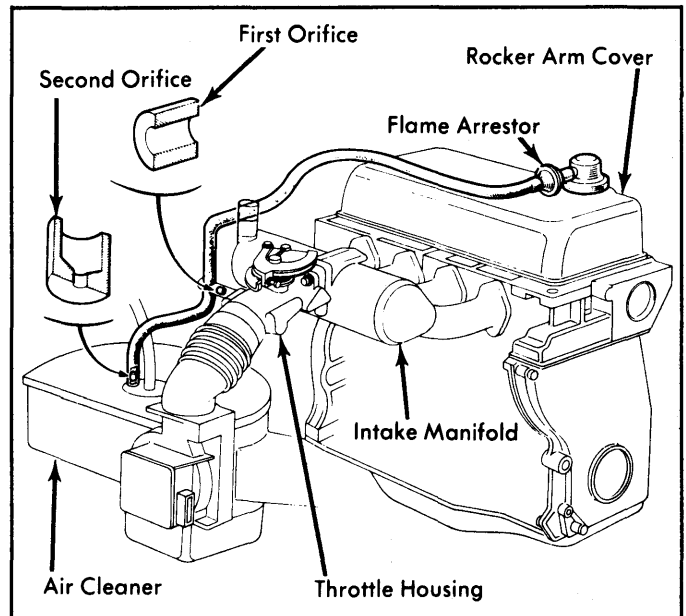
Fig. 5: 1975-76 Positive Crankcase Ventilation System (Fuel Injected Models)
