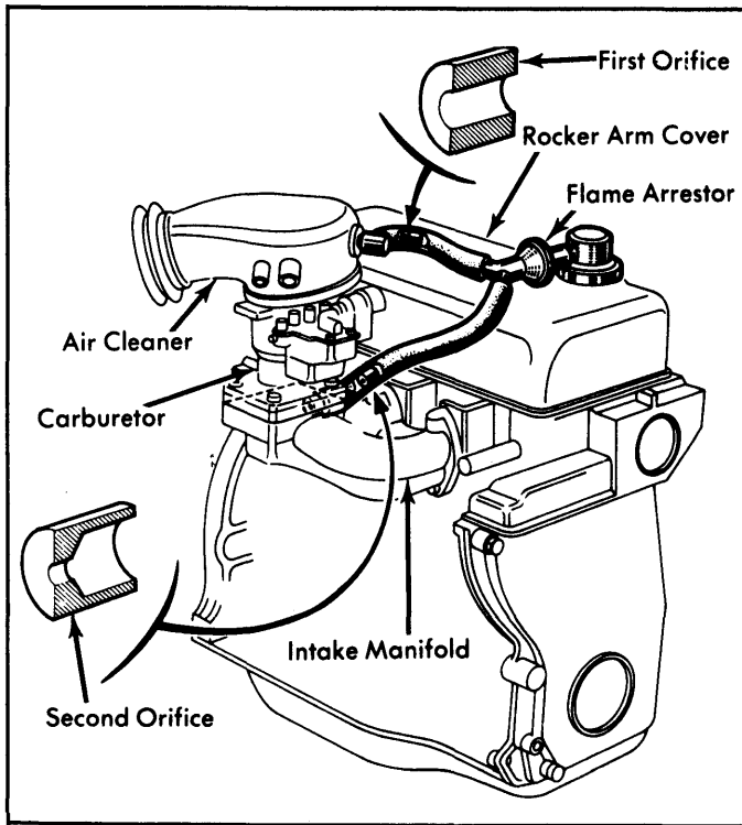
Fig. 4: 1975-76 Positive Crankcase Ventilation System (Carbureted Models Except R-5)
