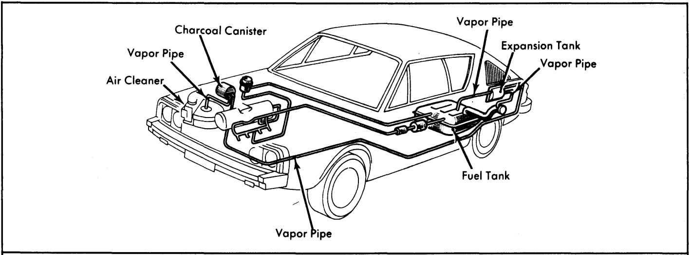
Fig. 3: 1975 Fuel Evaporation System
