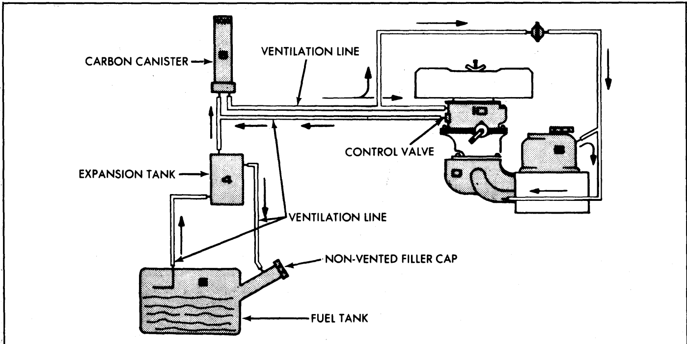
Fig. 1: 1974 Fuel Evaporation System
