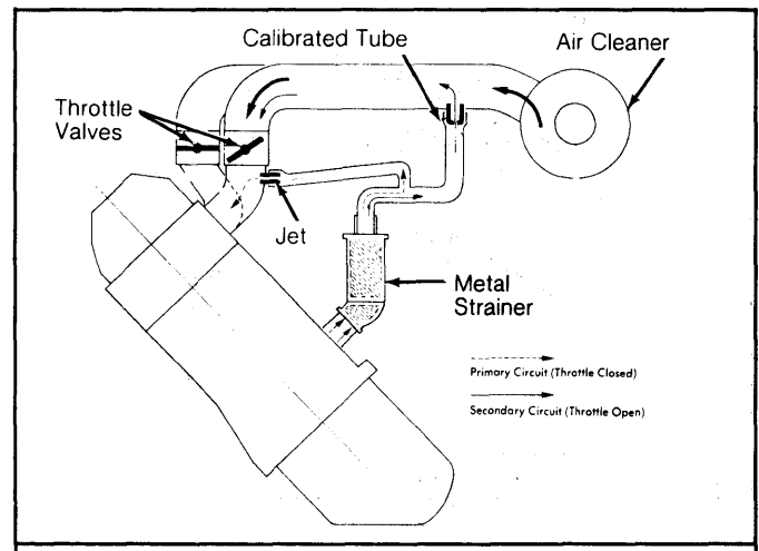
Fig. 4: 1977-78 Positive Crankcase Ventilation System
