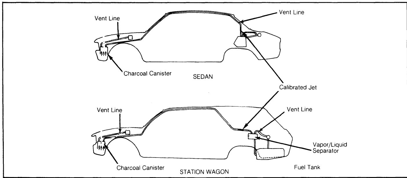
Fig. 3: 1977-78 505 Fuel Evaporation System
