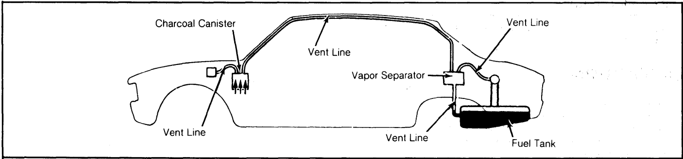
Fig. 1: 1974-75 Fuel Evaporation System
