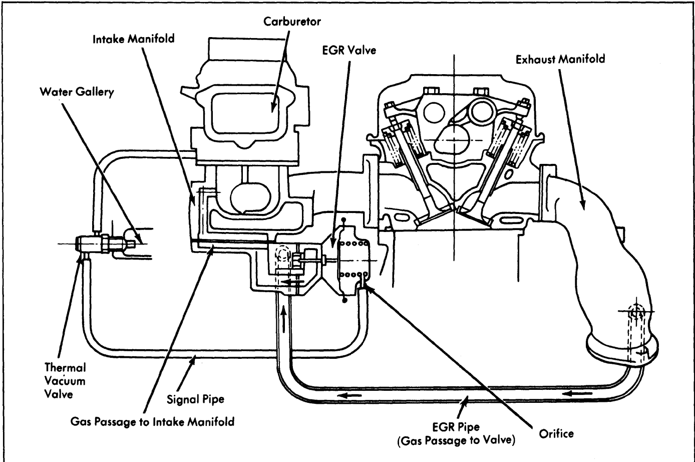
Fig. 3: 1976-77 Exhaust Gas Recirculation System
