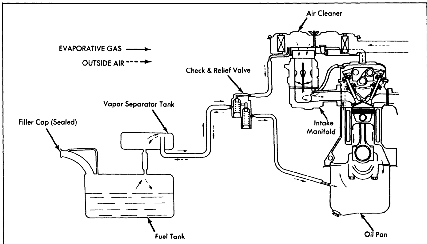
Fig. 4: 1976-78 Fuel Evaporation System
