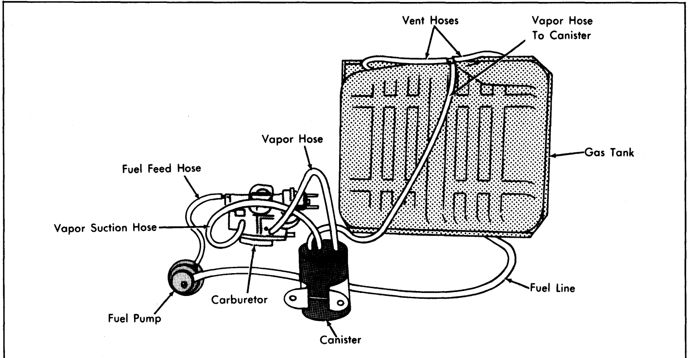
Fig. 1: 1974 Fuel Evaporation System
