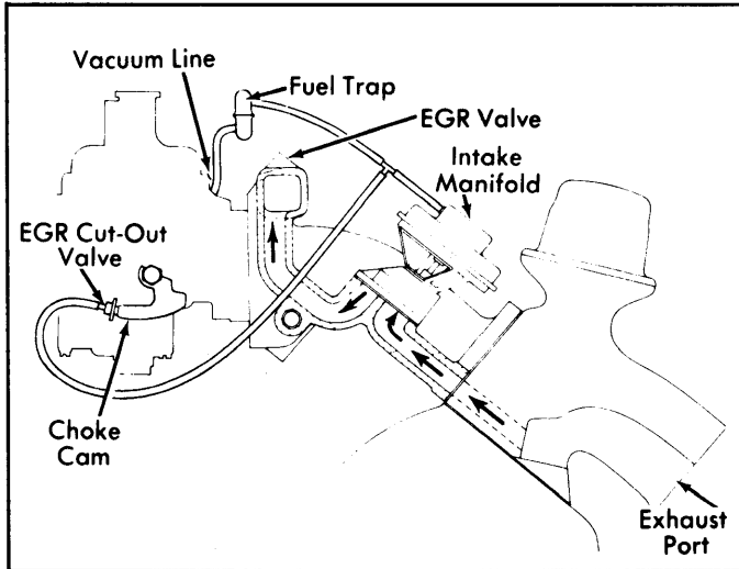
Fig. 4: 1975 Midget Exhaust Gas Recirculation System
