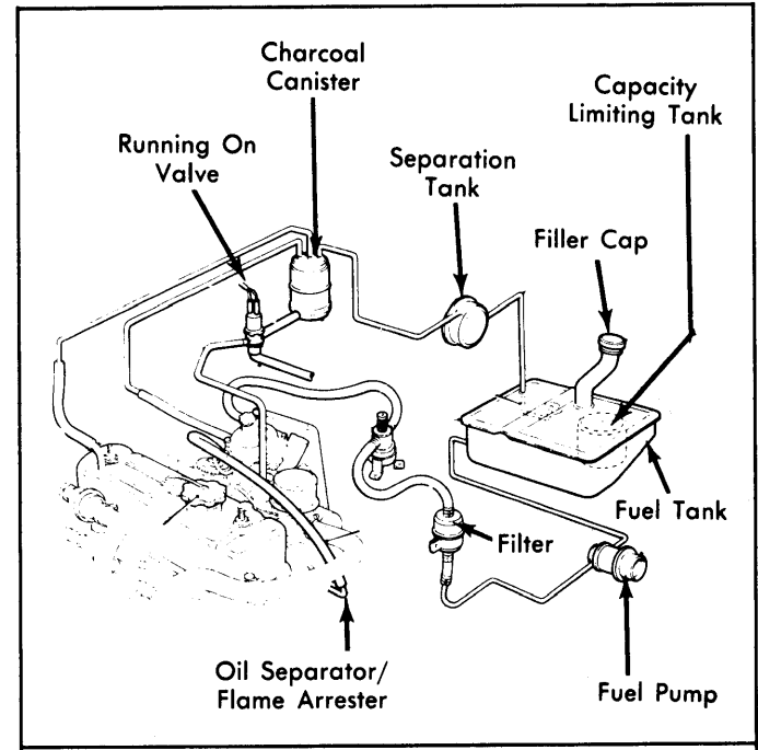
Fig. 8: 1977-78 MGB Fuel Evaporation System
