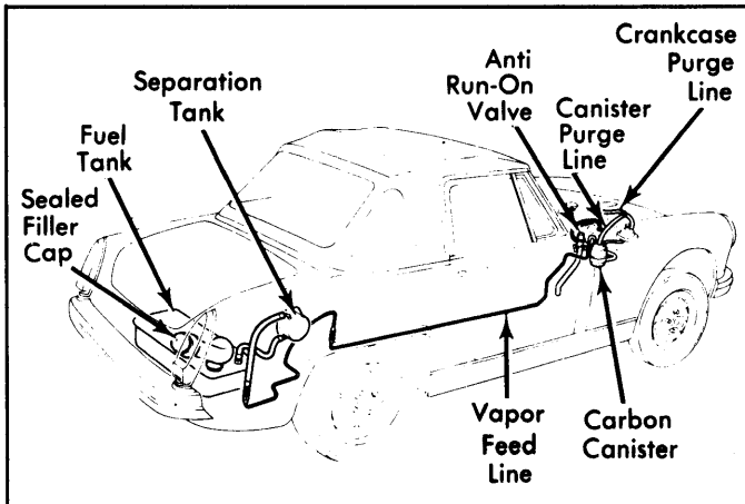
Fig. 5: 1975-76 Midget Fuel Evaporation System (MGB Similar)
