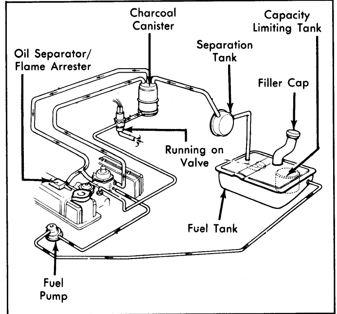
Fig. 7: 1977-78 Midget Fuel Evaporation System
