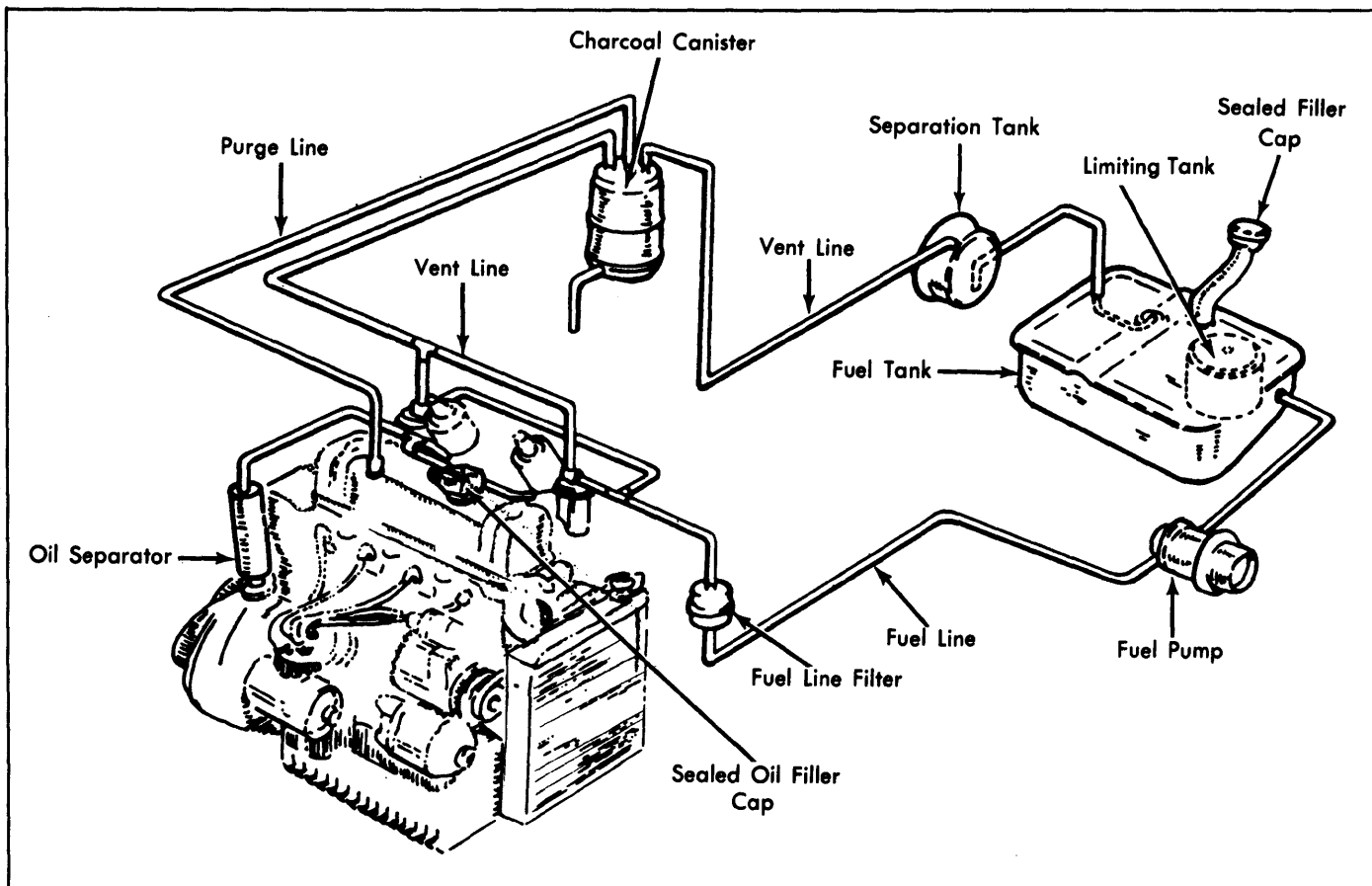
Fig. 1: 1974 Fuel Evaporation System
