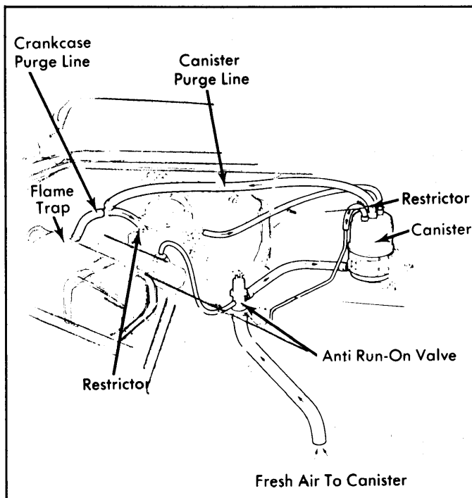
Fig. 6: 1975-76 Positive Crankcase Ventilation System
