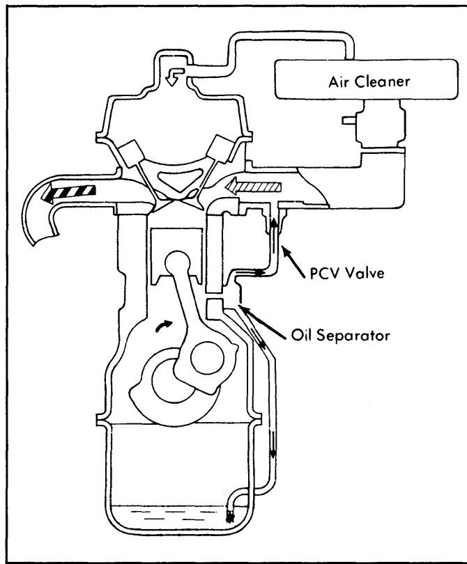
Fig. 8: 1974 808 Positive Crankcase Ventilation System
