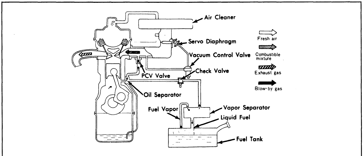
Fig. 2: 1974 808 Fuel Evaporation System (California & Federal Man. Trans.)
