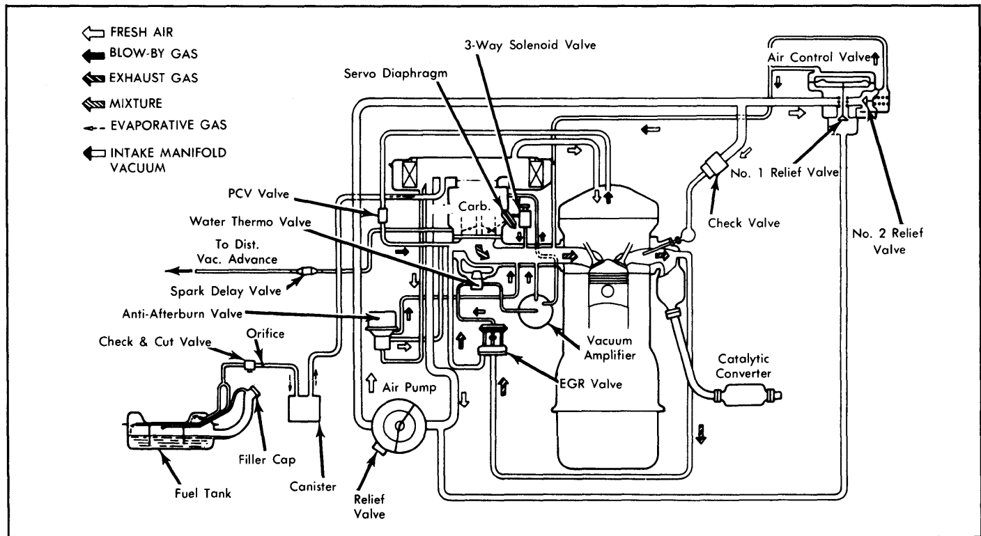
Fig. 24: 1979 GLC Exhaust Emission System (California Auto. Trans.)
