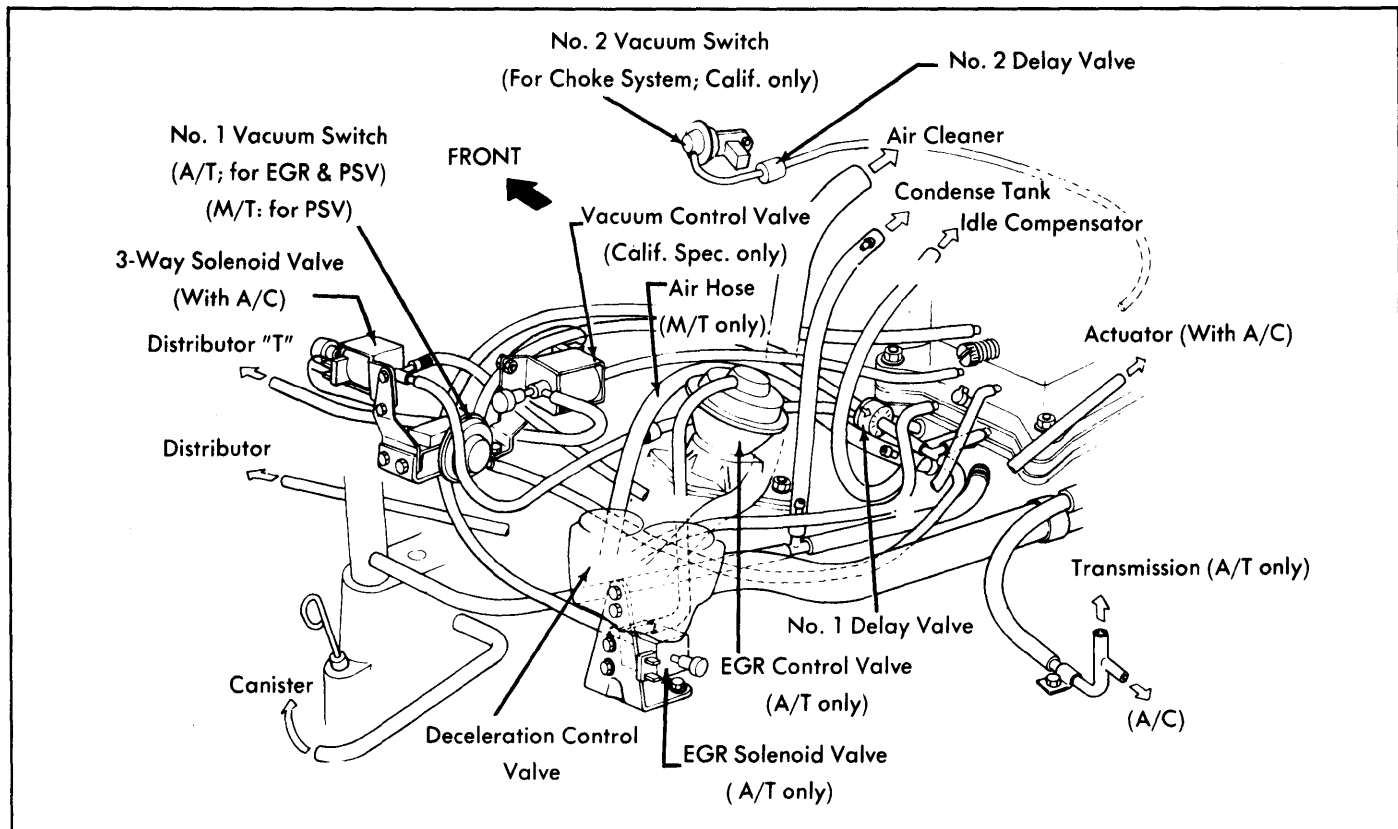
Fig. 16: 1977 RX4 & Cosmo Exhaust Emission System (California & Federal Auto. Trans.)
