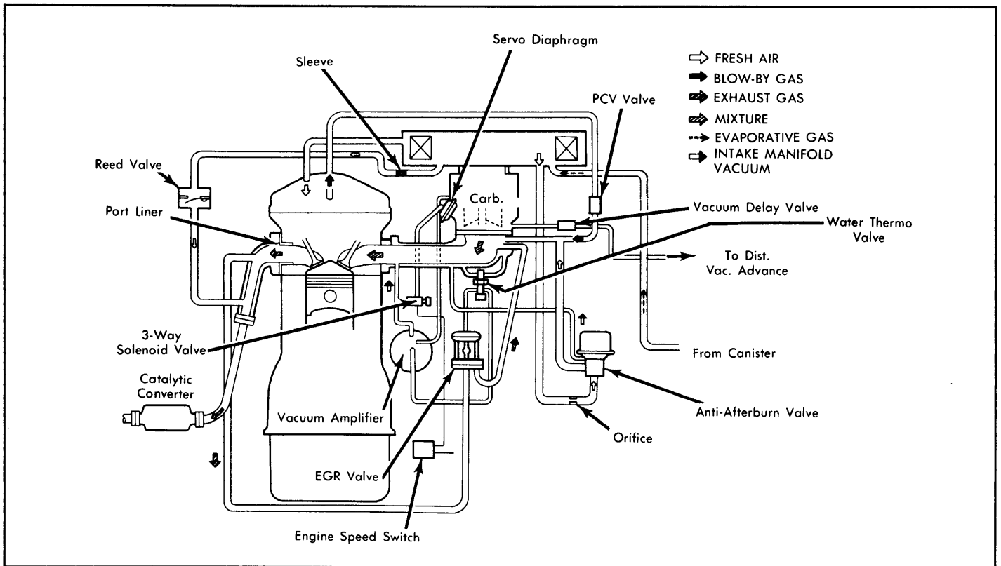
Fig. 22: 1979 B2000 Exhaust Emission System (Federal)
