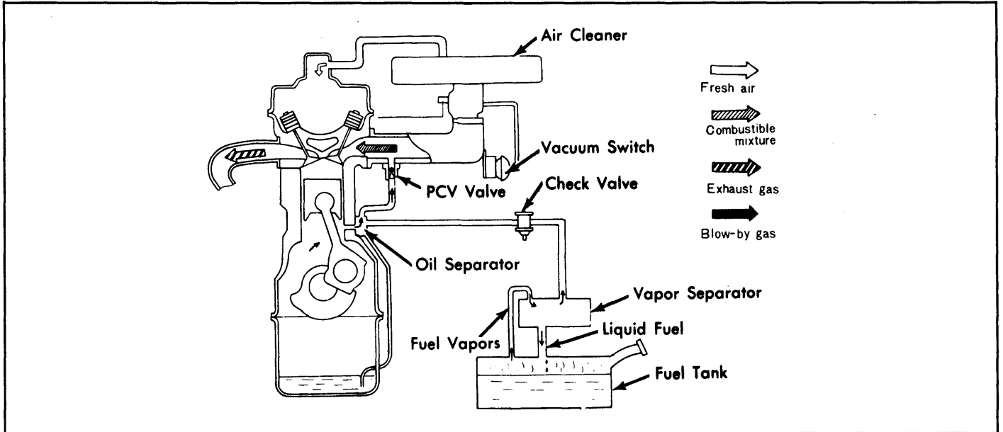
Fig. 1: 1974 808 Fuel Evaporation System (California Auto. Trans.)
