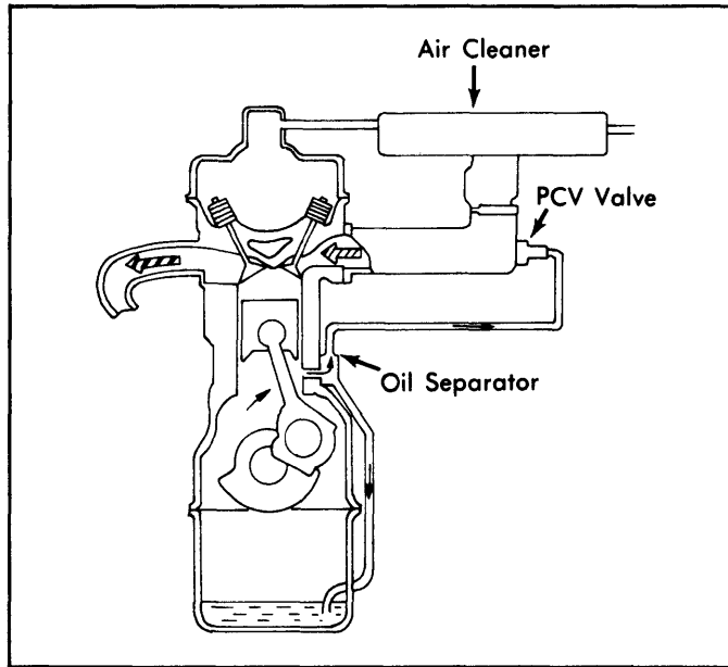
Fig. 9: 1974 B1600 Positive Crankcase Ventilation System
