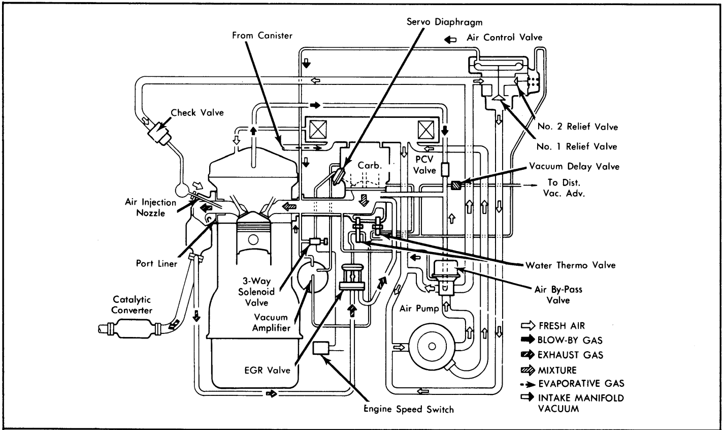
Fig. 21: 1979 B2000 Exhaust Emission System (California)
