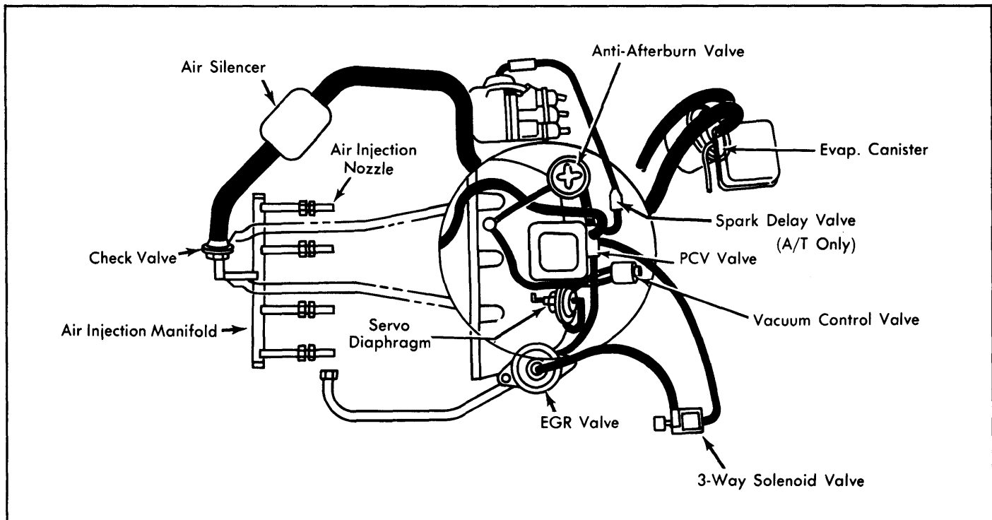
Fig. 20: 1978 GLC Exhaust Emission System (Federal)
