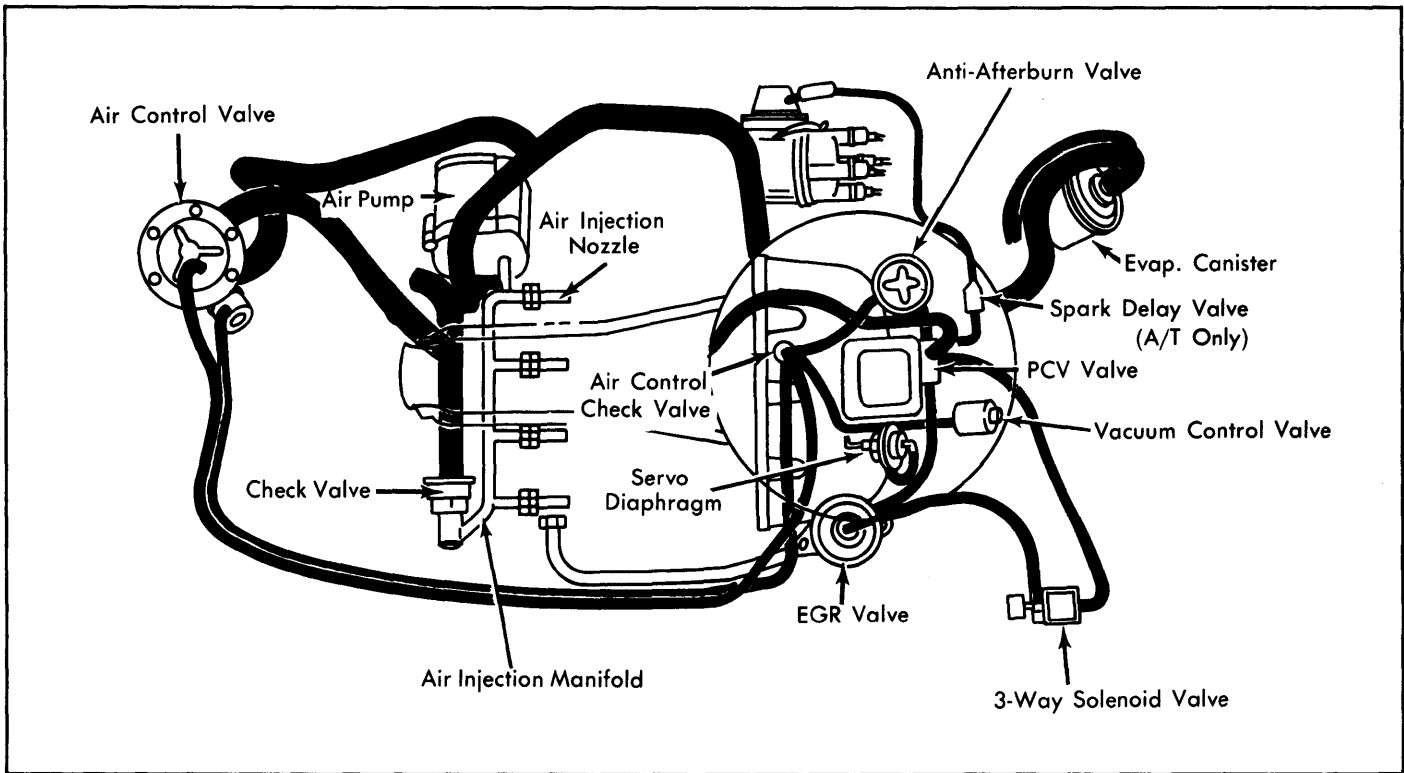
Fig. 19: 1978 GLC Exhaust Emission System (California)
