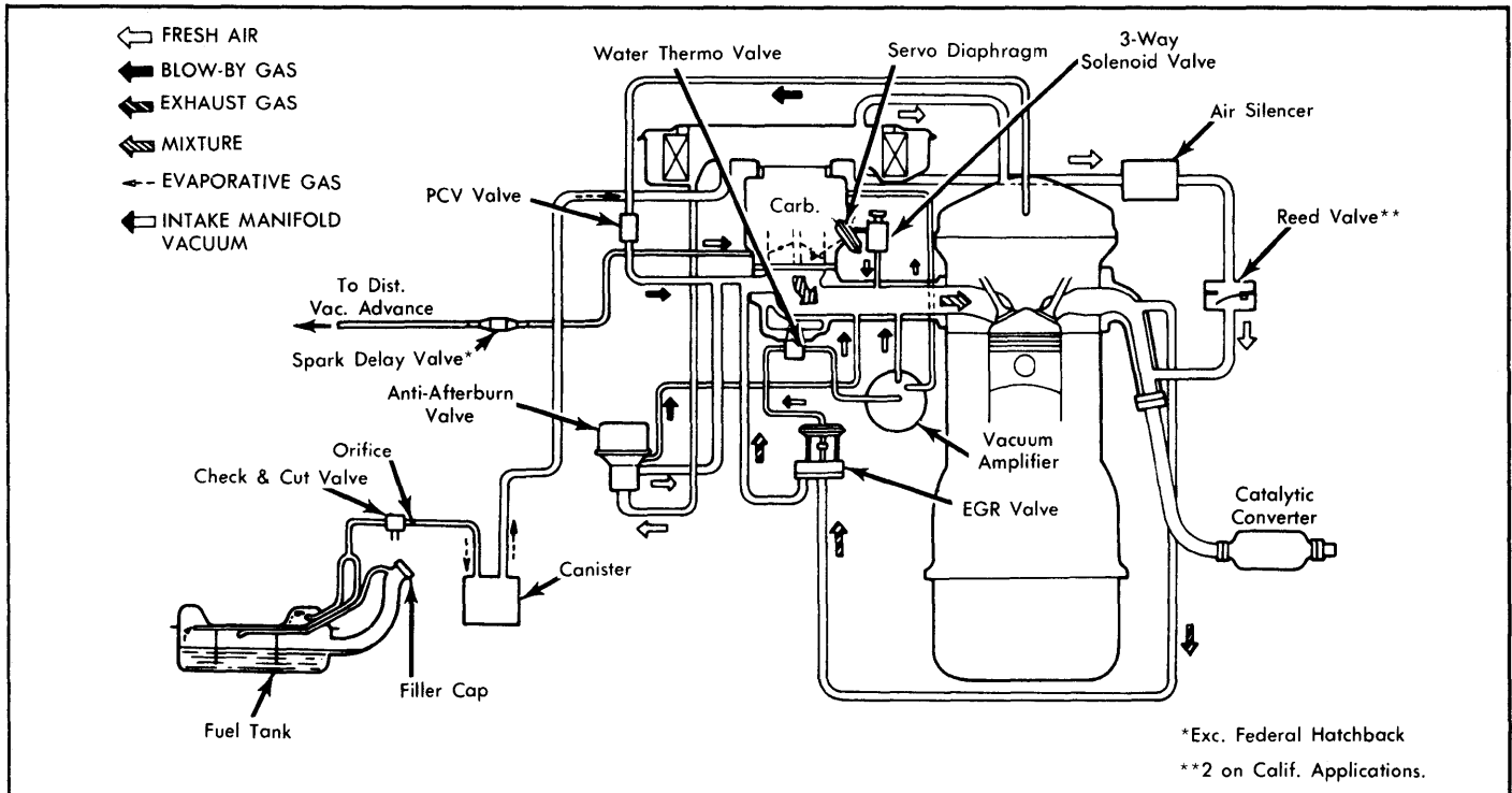
Fig. 23: 1979 GLC Exhaust Emission System (All Except California With Auto. Trans.)
