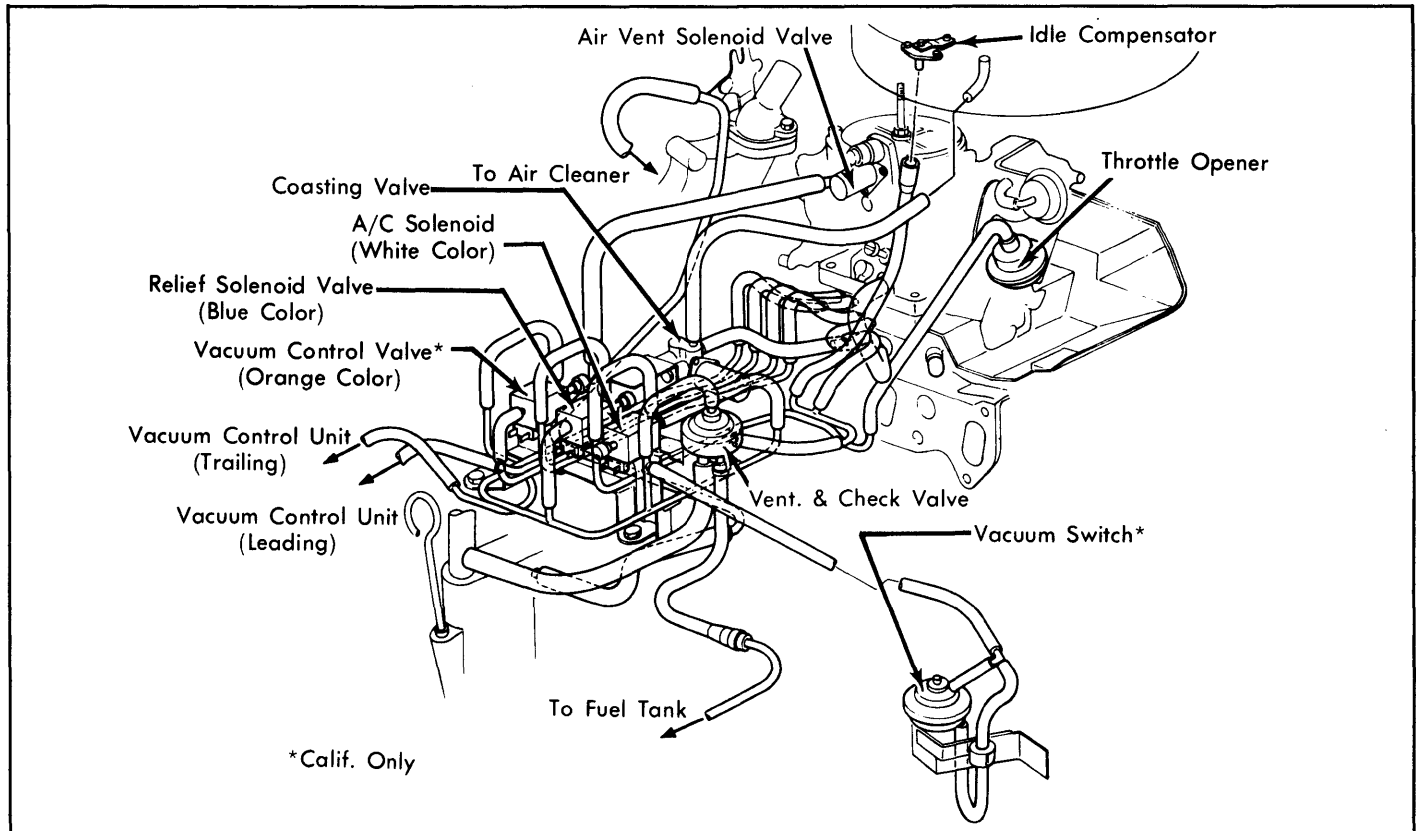
Fig. 26: 1979 RX7 Exhaust Emission System (Man. Trans.)
