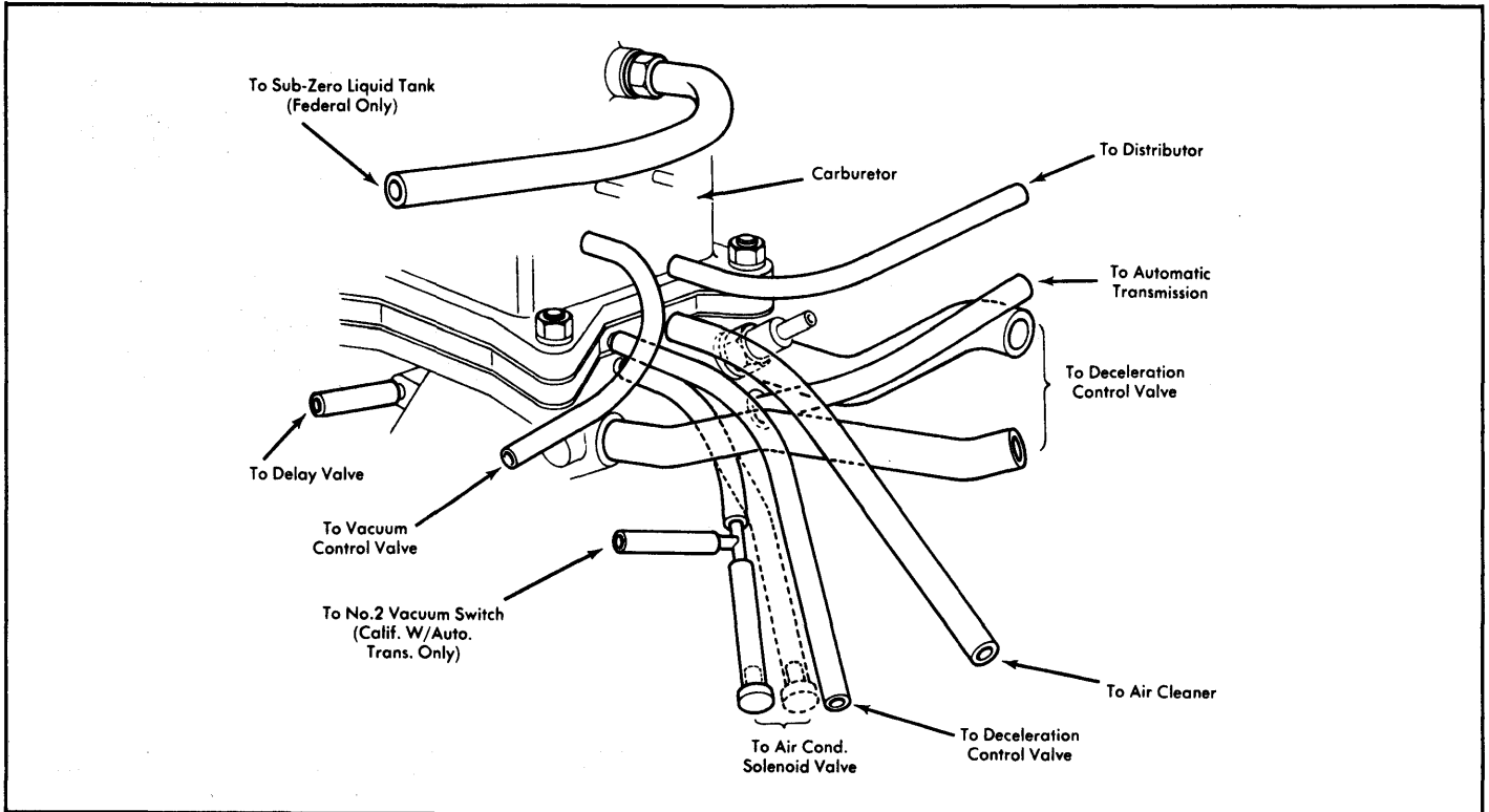
Fig. 13: 1976 RX4 & Cosmo Exhaust Emission System
