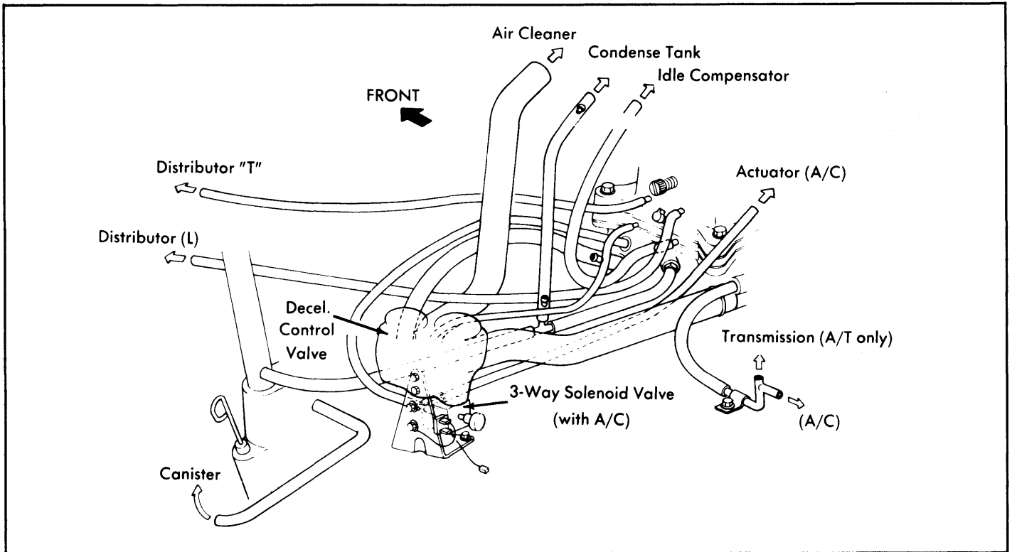
Fig. 17: 1977 RX4 & Cosmo Exhaust Emission System (Federal Man. Trans.)
