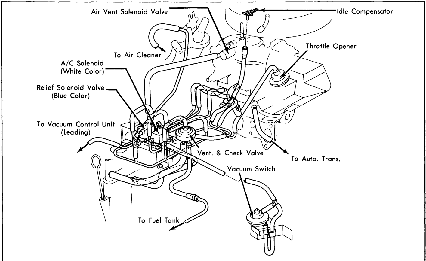
Fig. 25: 1979 RX7 Exhaust Emission System (Auto. Trans.)
