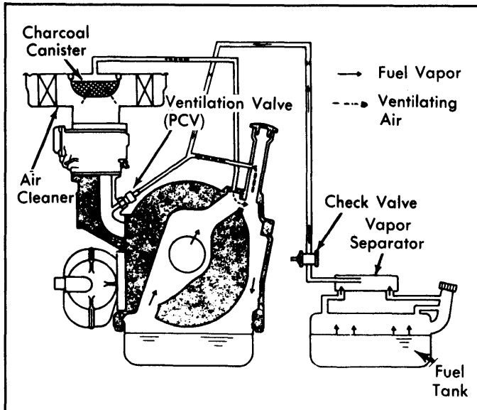
Fig. 6: 1974-78 Fuel Evaporation System (Rotary)
