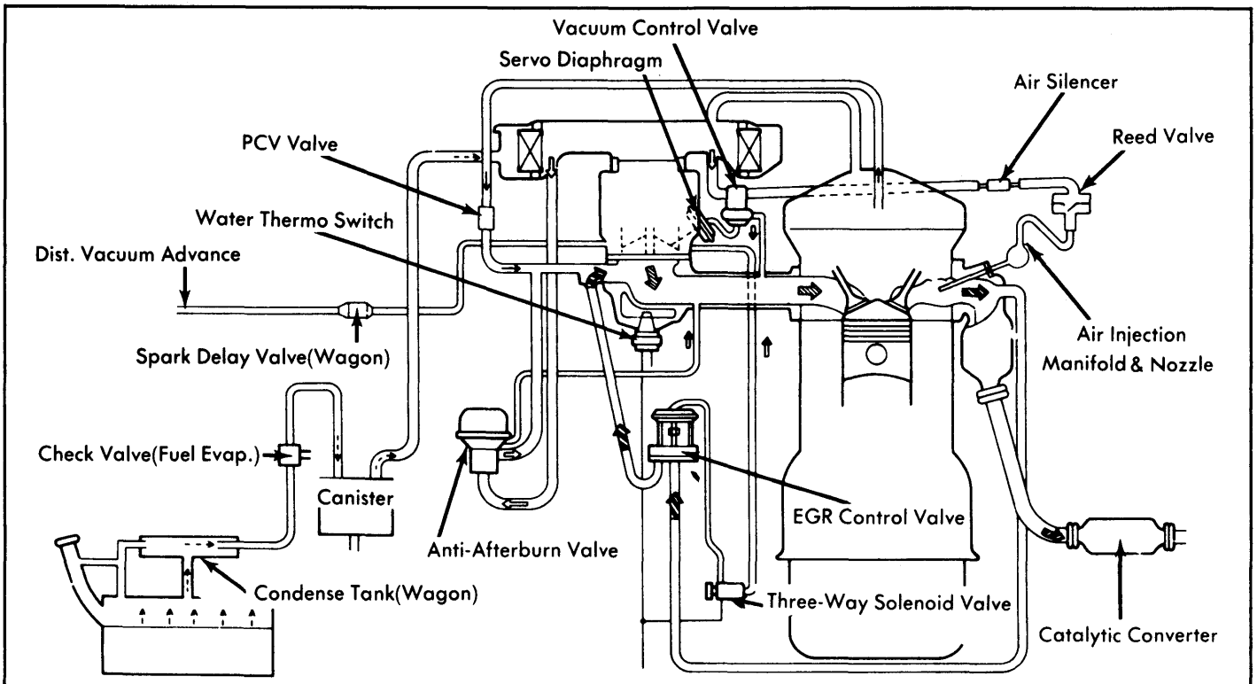
Fig. 14: 1977 808 (1300) Exhaust Emission System (Federal)
