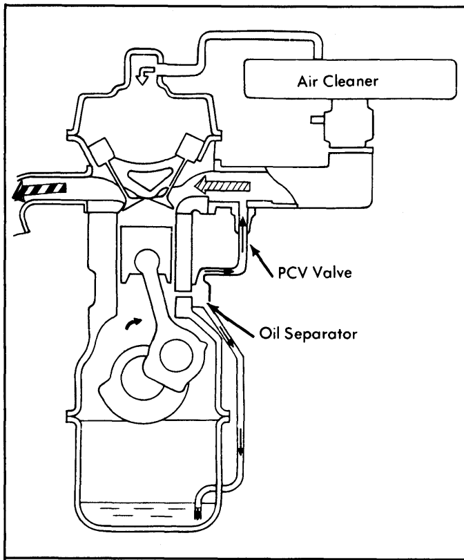
Fig. 7: 1974 808 & 1800 Positive Crankcase Ventilation System
