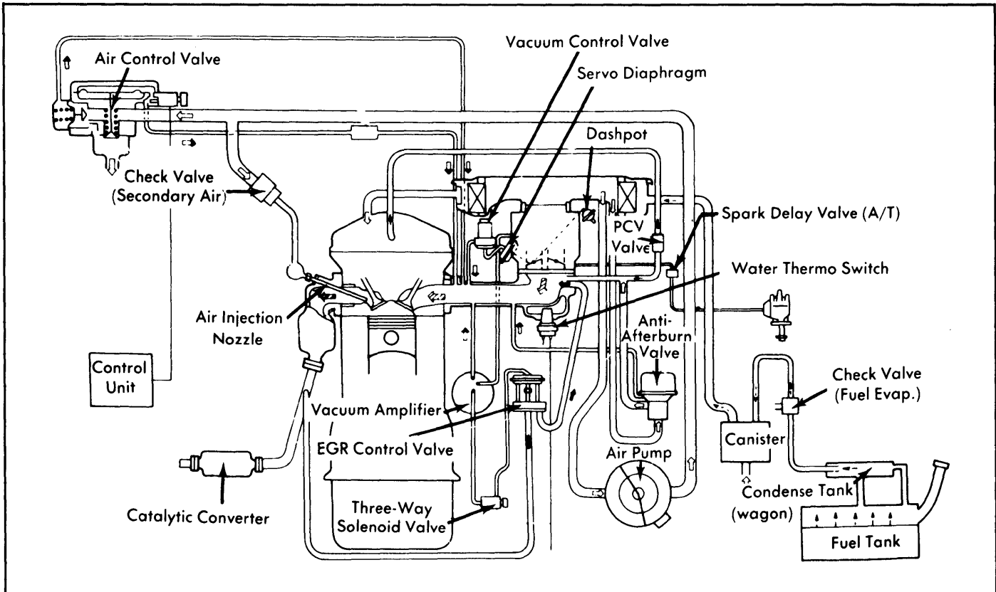
Fig. 15: 1977 808 (1600) Exhaust Emission System (California)
