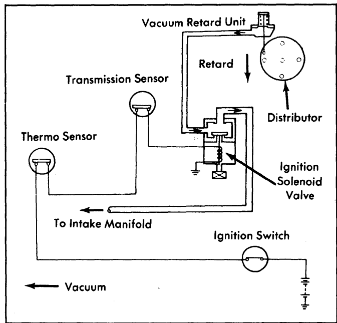
Fig. 13: 1977 Ignition Timing Control System (Man. Trans. Except CVCC)
