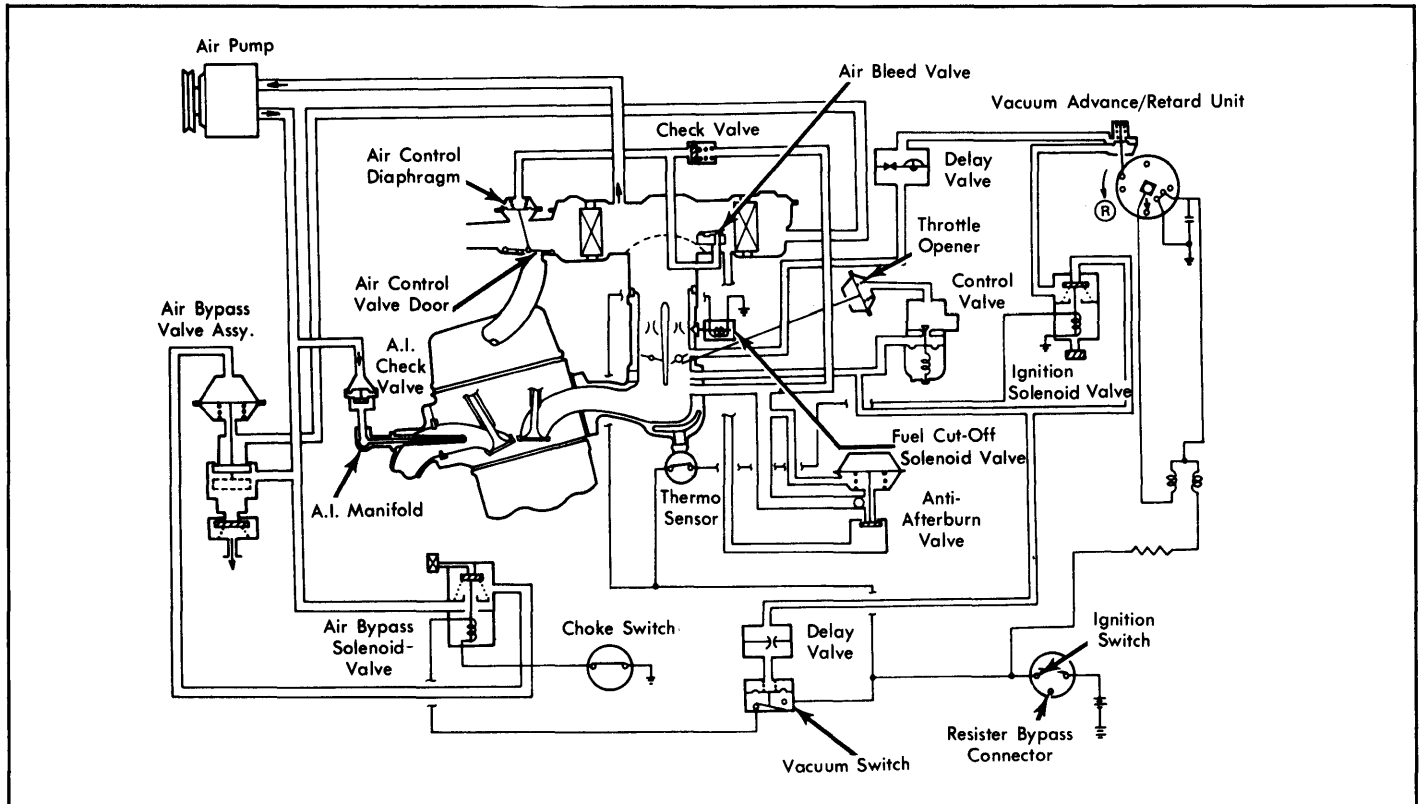
Fig. 25: 1979 Civic 1200 Exhaust Emission System (Man. Trans.)
