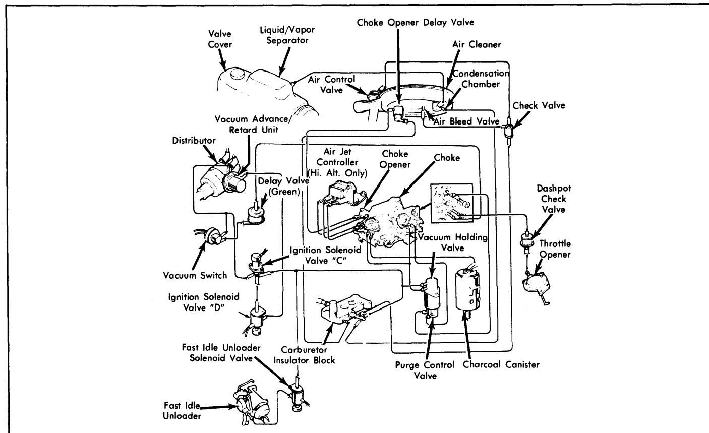
Fig. 24: 1979 Accord & Prelude Exhaust Emission System (Calif. & High Altitude Auto. Trans.)
