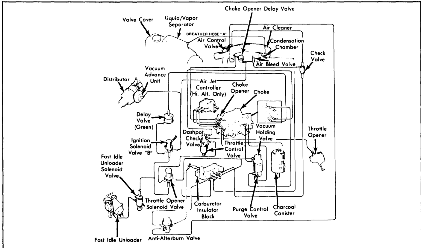
Fig. 23: 1979 Accord & Prelude Exhaust Emission System (Calif. & High Altitude Man. Trans.)
