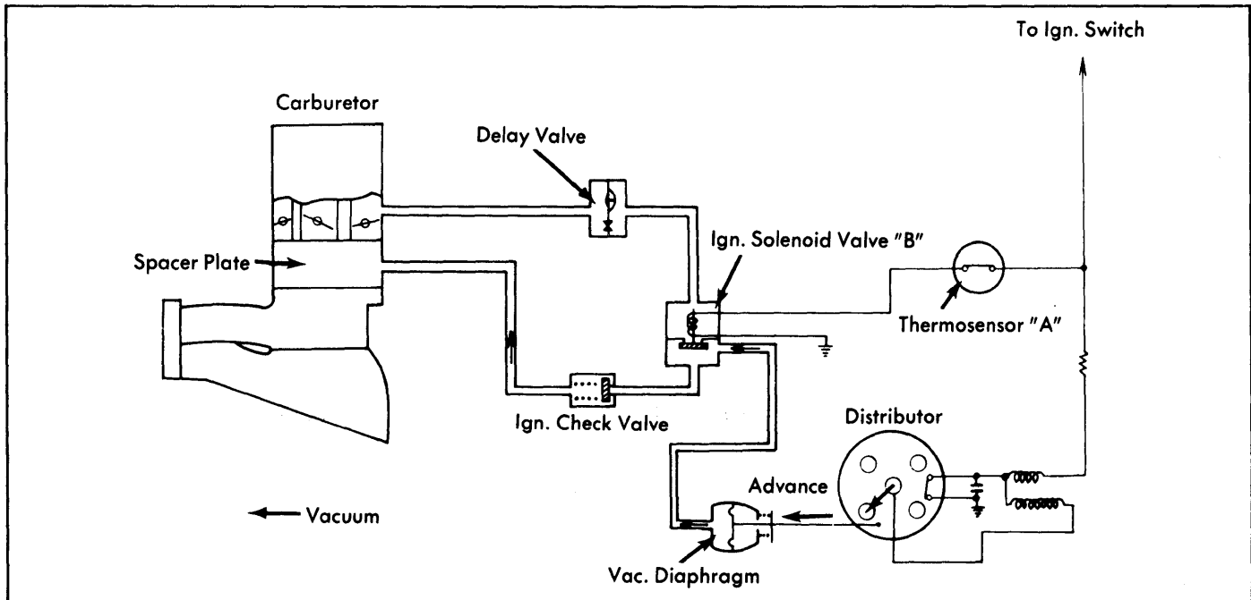
Fig. 11: 1977 Ignition Timing Control System (Federal Auto. Trans. & All Man. Trans.)
