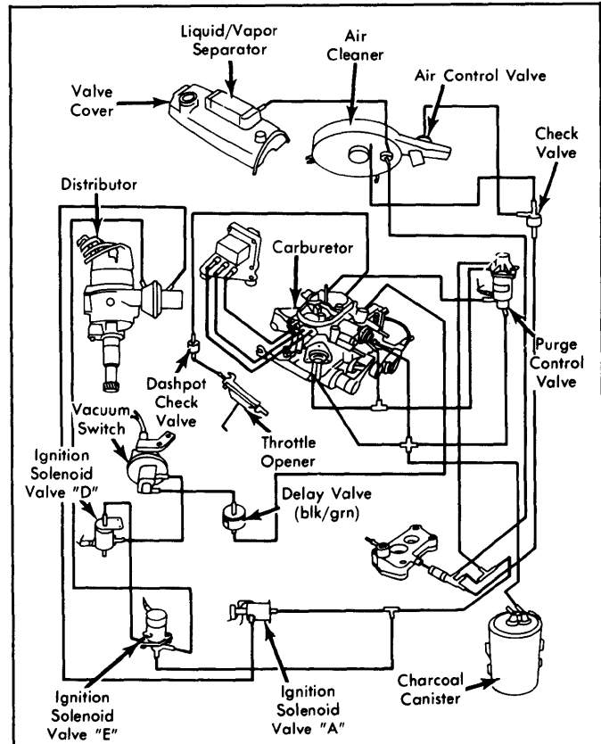
Fig. 30: 1979 Civic CVCC Station Wagon Exhaust Emission System (Calif. & High Altitude Auto. Trans.)
