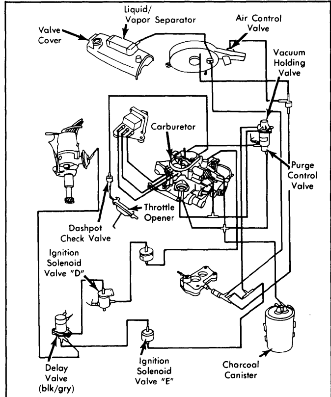
Fig. 29: 1979 Civic CVCC Exhaust Emission System (Auto. Trans. Except Calif. & High Alt. Wagon)
