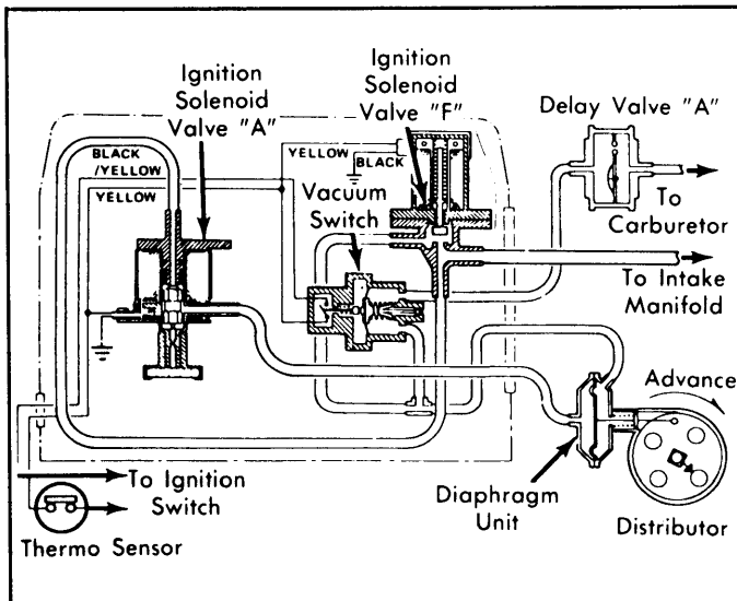
Fig. 20: 1978 Ignition Timing Control System (Calif. & High Altitude Auto. Trans. Accord)
