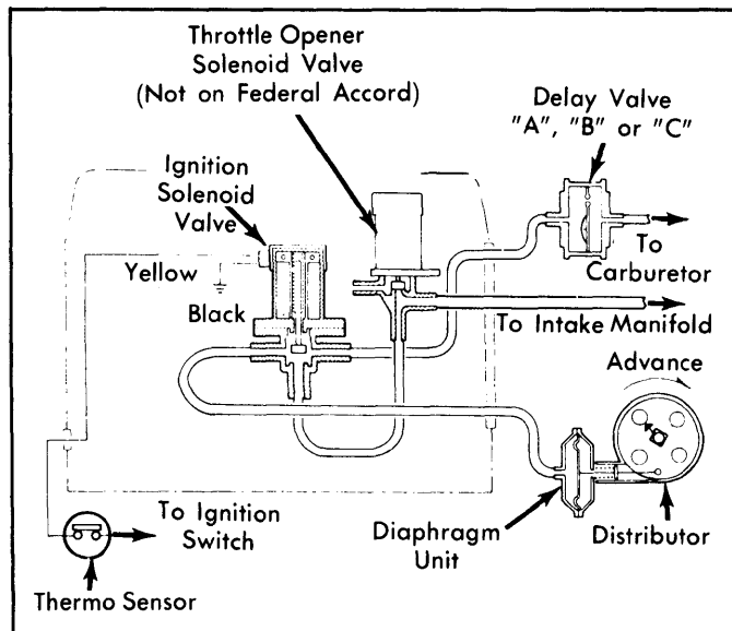
Fig. 18: 1978 Ignition Timing Control System (Federal Auto. Trans. Accord & All Man. Trans. Models)
