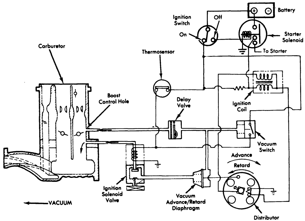
Fig. 6: 1976 Ignition Timing Control System (Auto. Trans.)
