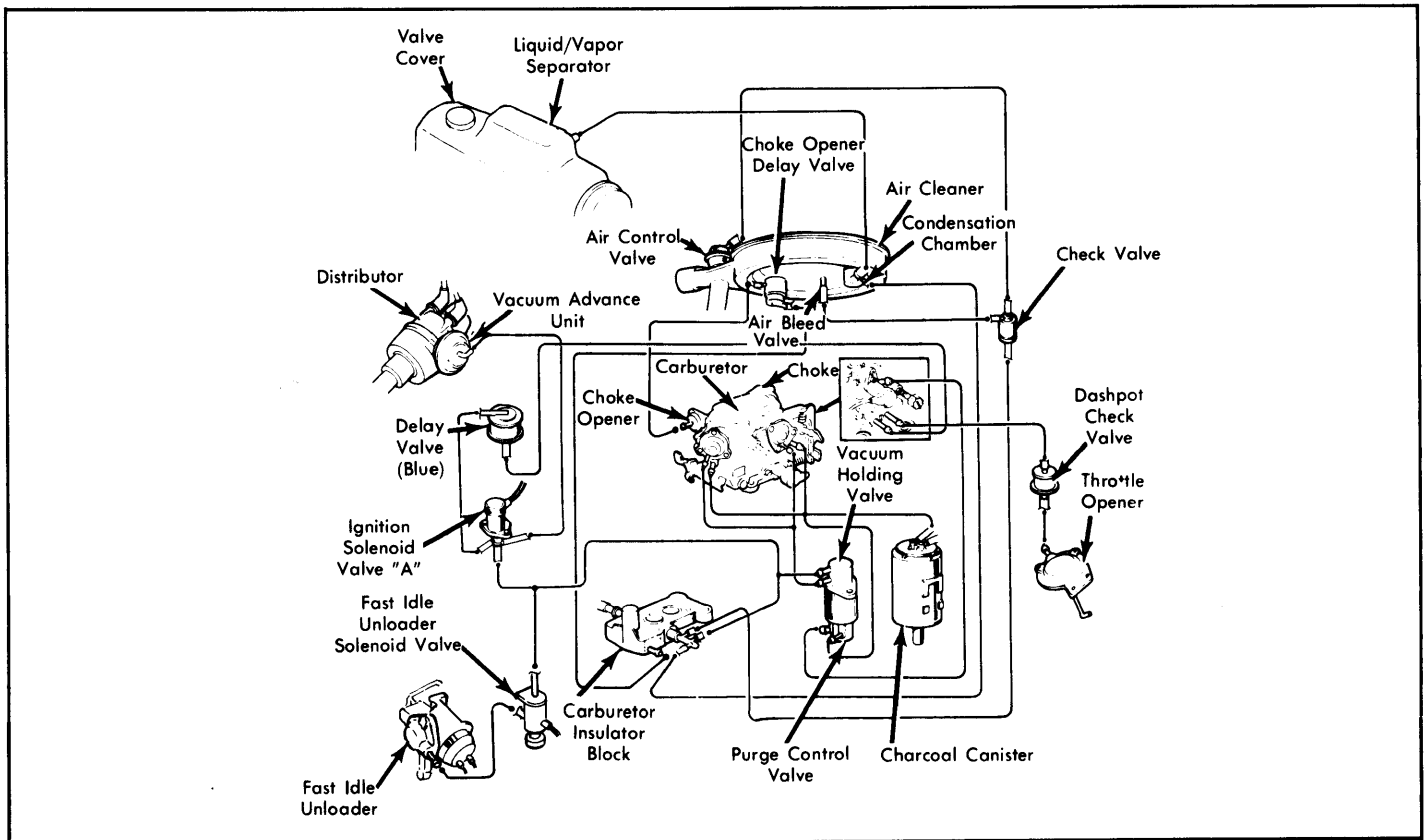
Fig. 21: 1979 Accord & Prelude Exhaust Emission System (Federal)
