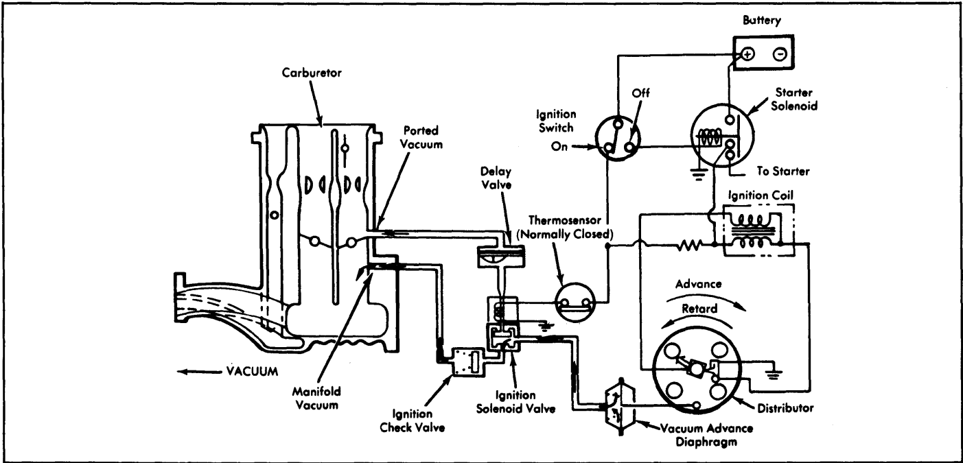
Fig. 7: 1976 Ignition Timing Control System (Man. Trans.)
