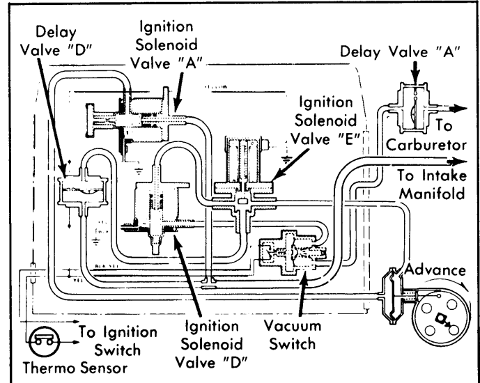
Fig. 22: 1978 Ignition Timing Control System (Calif. & High Altitude Auto. Trans. Civic Wagon)
