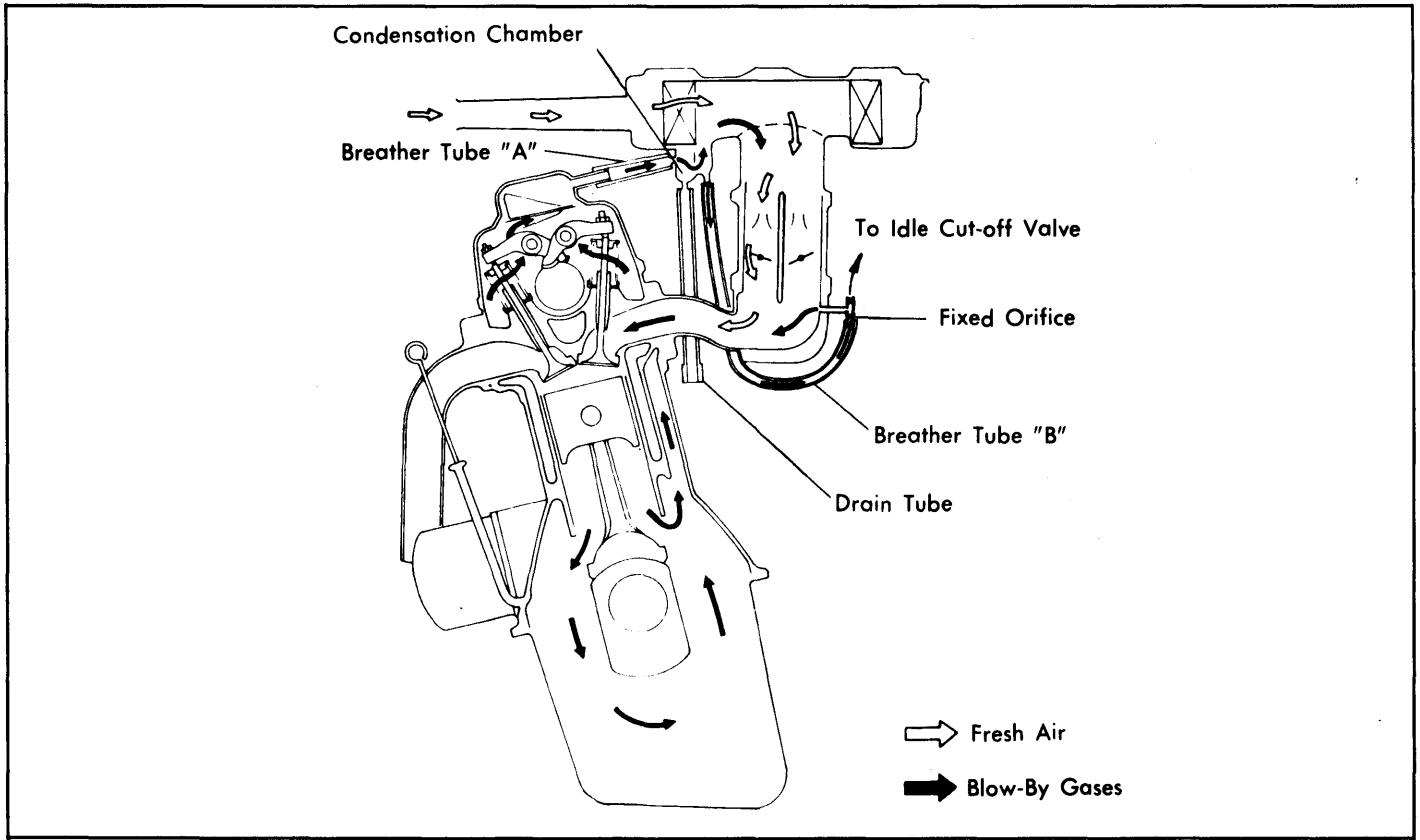
Fig. 1: 1974 Positive Crankcase Ventilation System (Typical)
