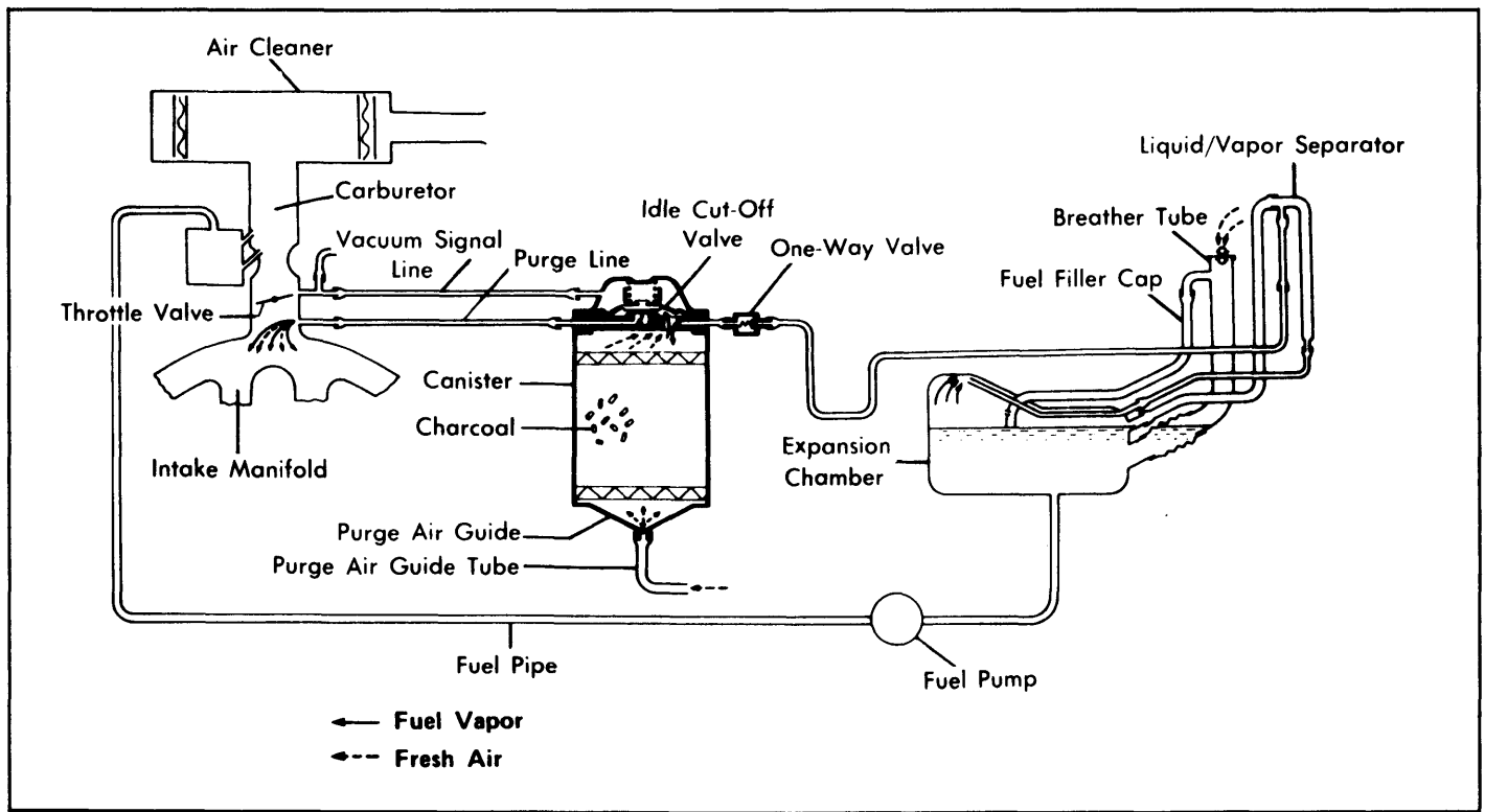
Fig. 2: 1974-76 Fuel Evaporation System
