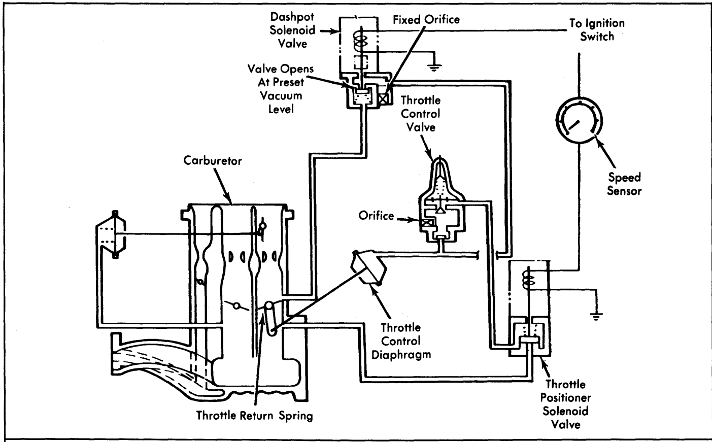
Fig. 8: 1976 Throttle Positioner System
