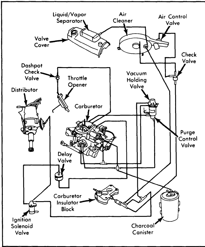
Fig. 27: 1979 Civic CVCC Exhaust Emission System (Federal Man. Trans.)
