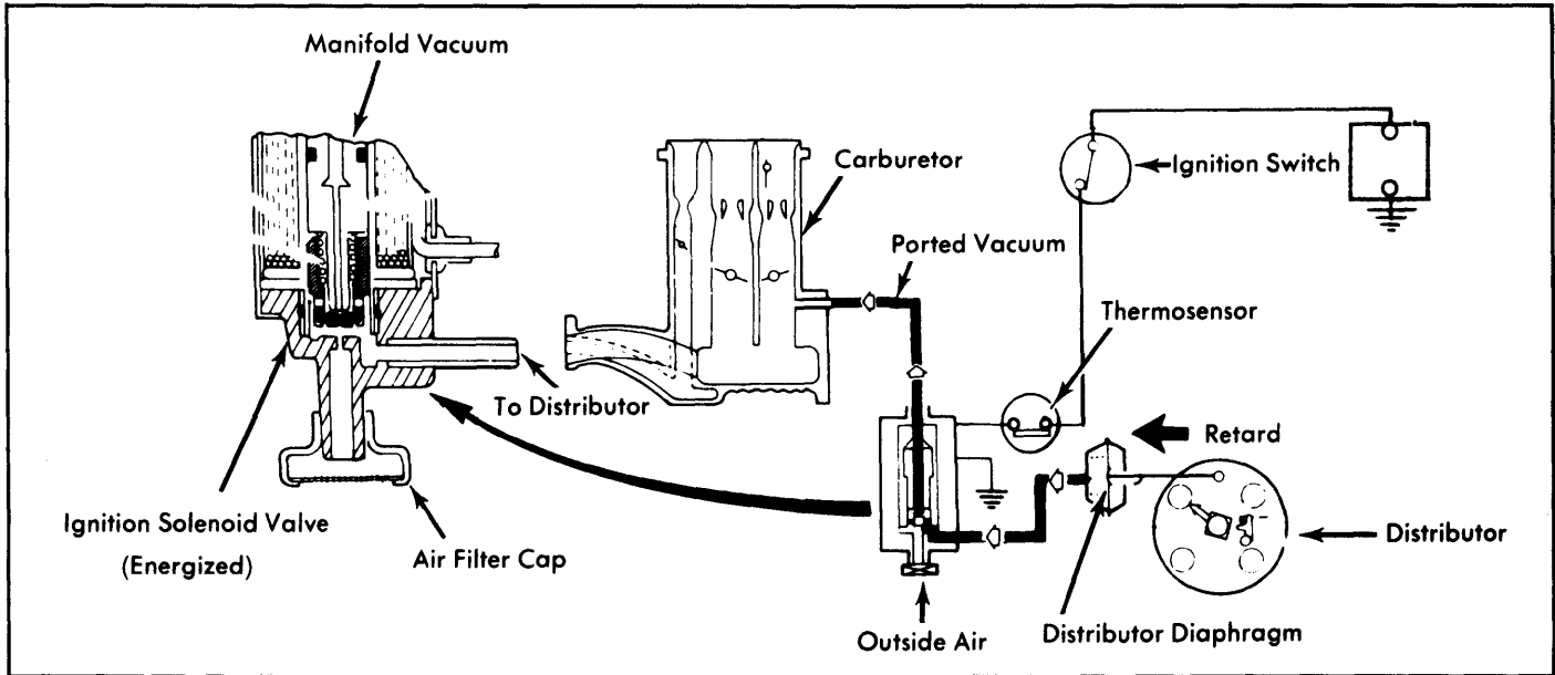
Fig. 3: 1975 Ignition Timing Control System (Auto. Trans.)
