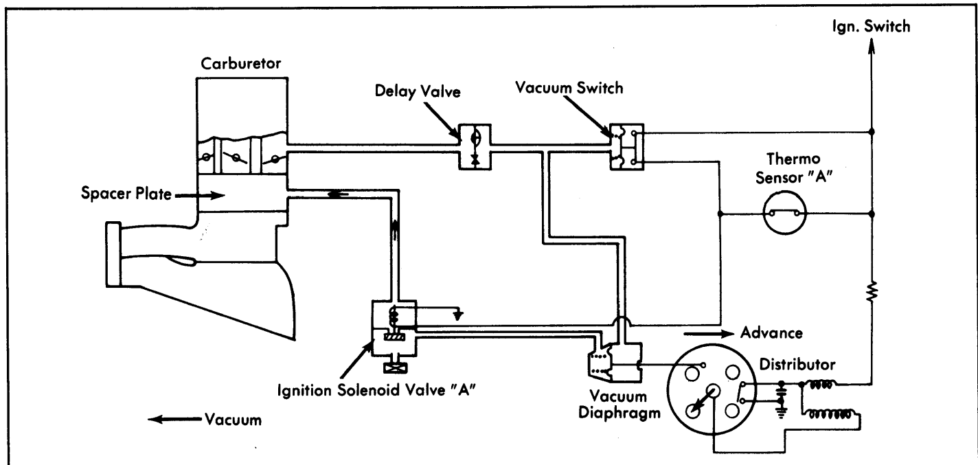
Fig. 10: 1977 Ignition Timing Control System (California & High Altitude)
