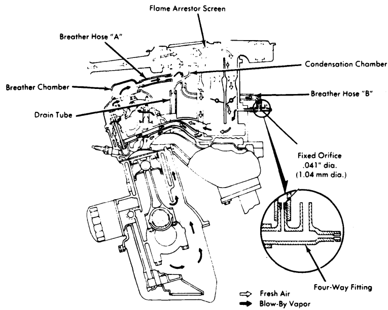
Fig. 5: 1975-76 Positive Crankcase Ventilation System (Typical)
