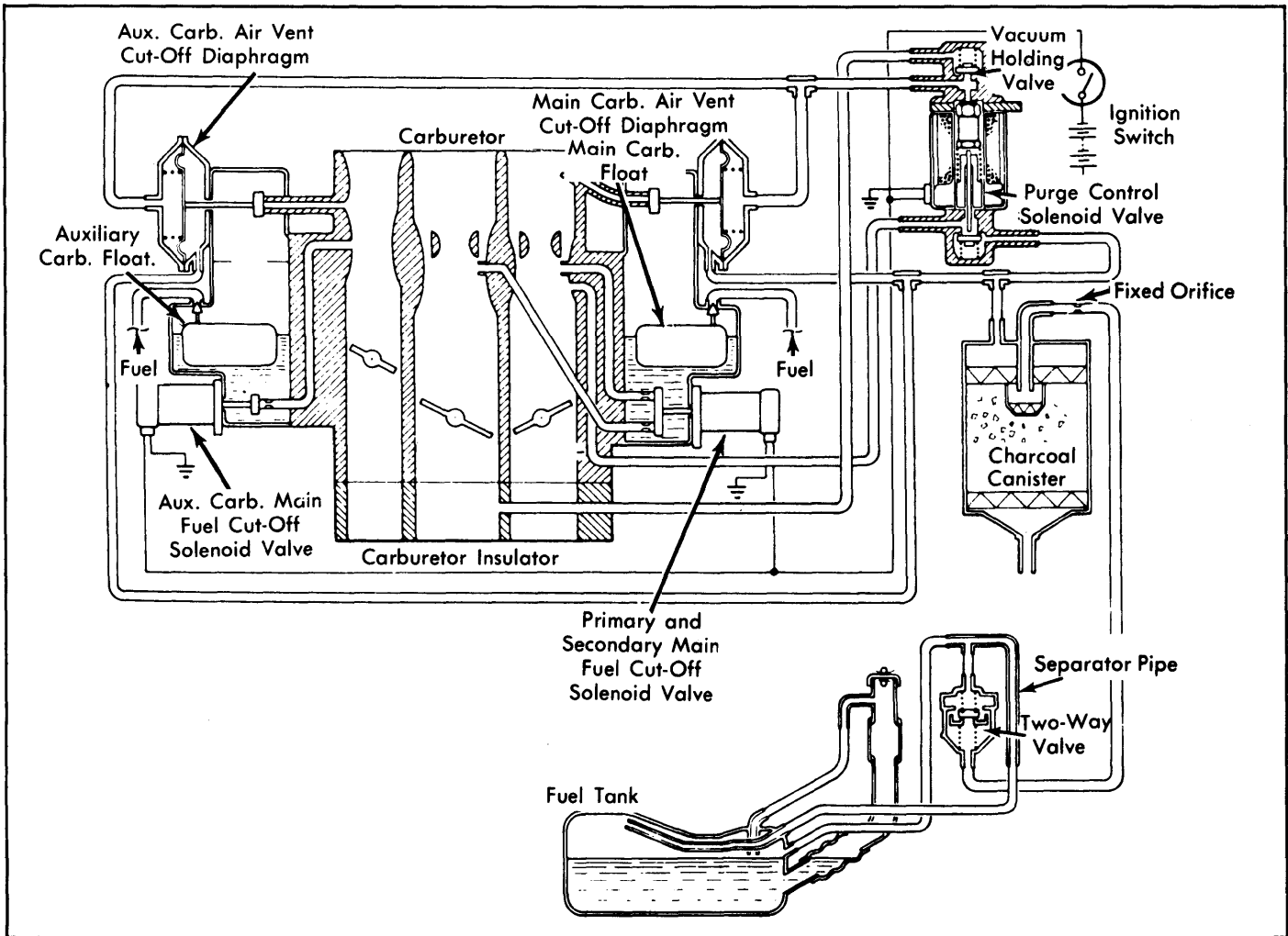
Fig. 17: 1978 Civic CVCC & Accord Fuel Evaporation System
