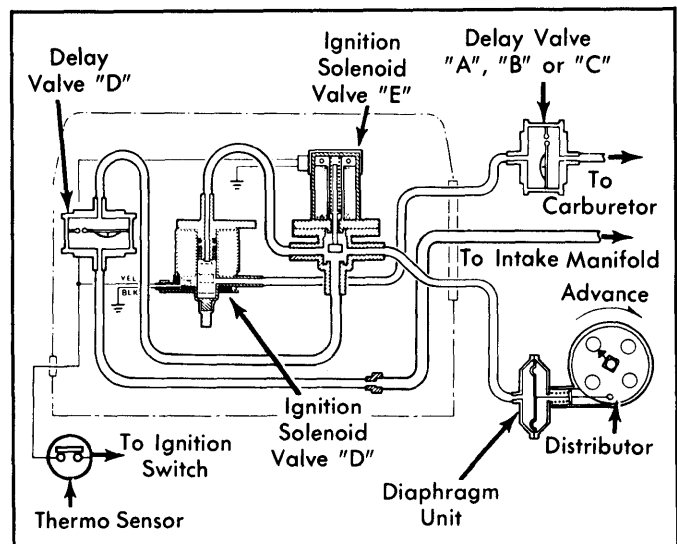
Fig. 19: 1978 Ignition Timing Control System (Federal Auto. Trans. Wagon & Auto. Trans. Civic Sedan)
