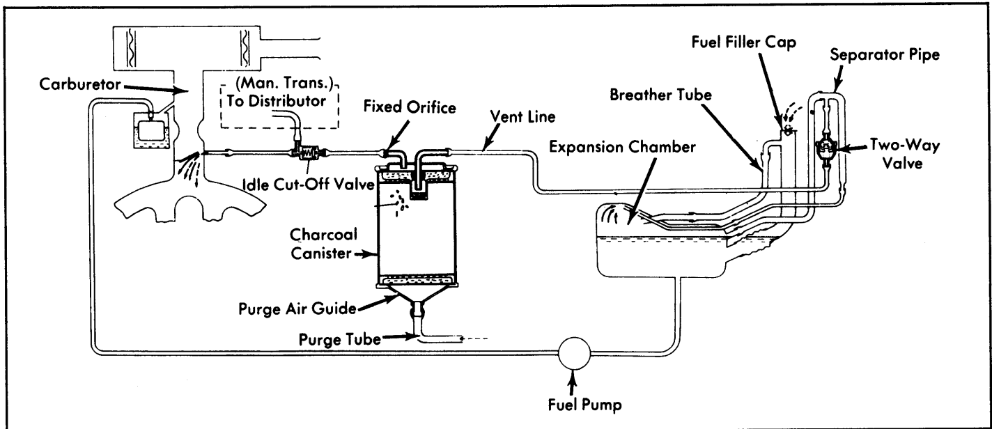
Fig. 9: 1977 Fuel Evaporation System
