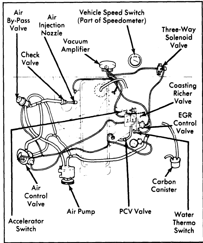
Fig. 6: 1977 2.3L Exhaust Emission System (California)
