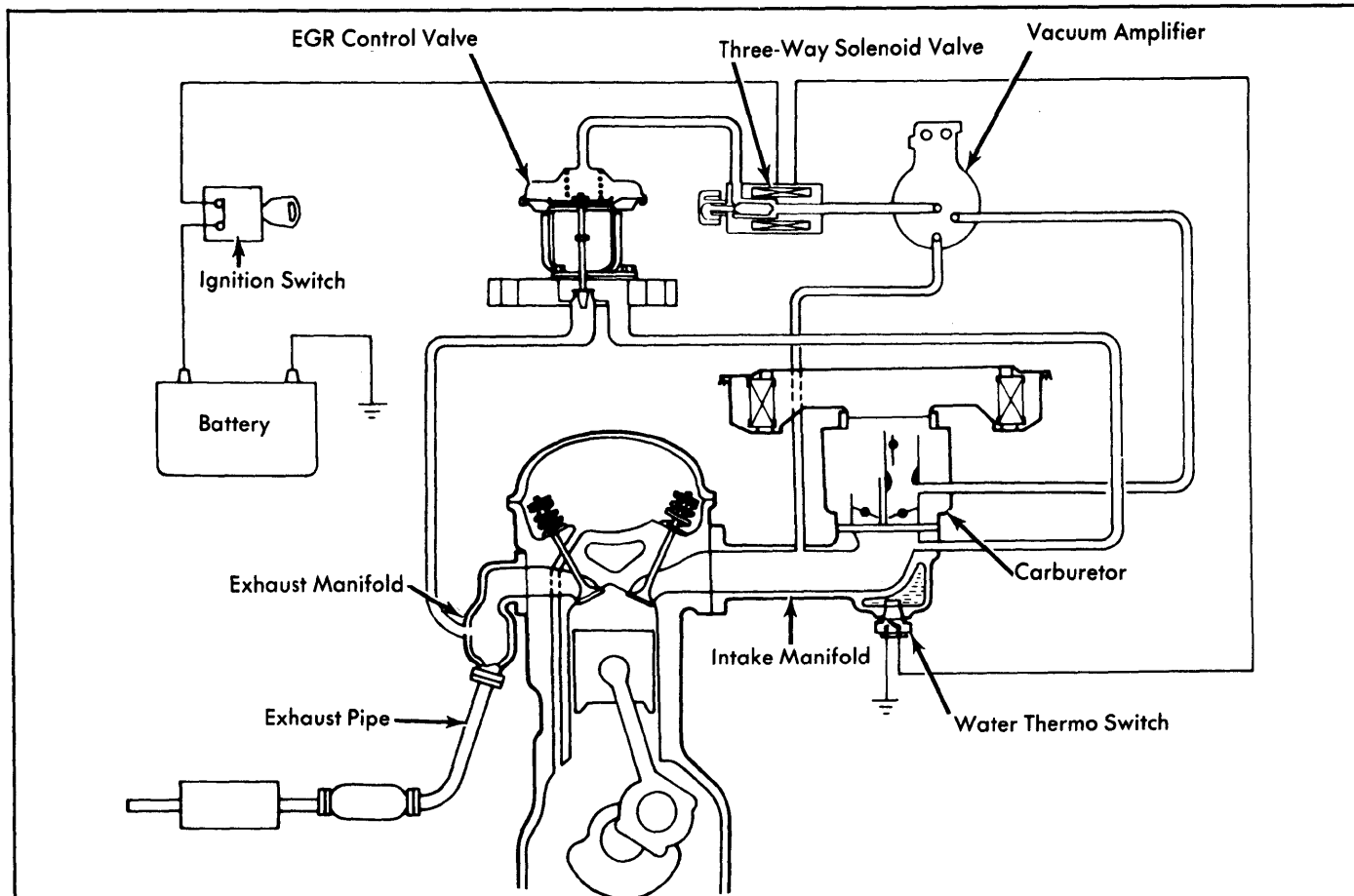
Fig. 5: 1977 Exhaust Gas Recirculation System
