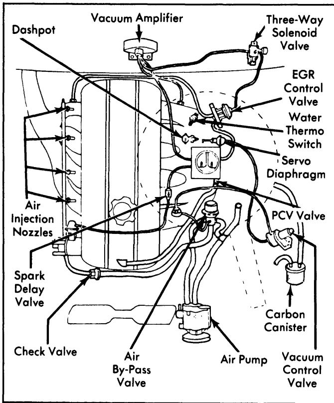
Fig. 2: 1977 1.8L Exhaust Emission System (Except California)
