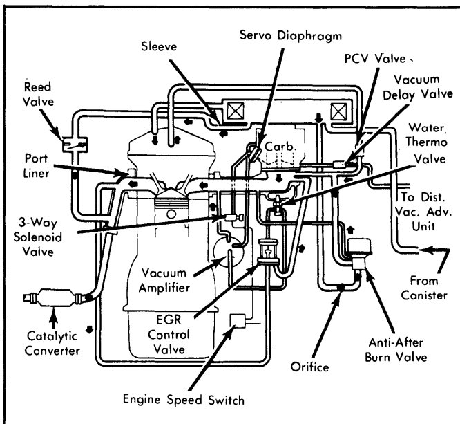
Fig. 8: 1979 2.0L Federal Exhaust Emission System
