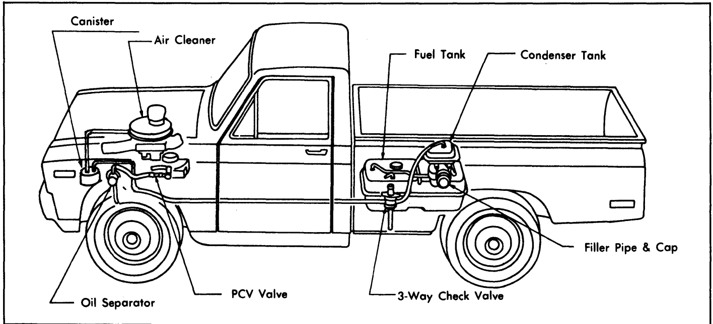
Fig. 1: 1974-76 Fuel Evaporation System
