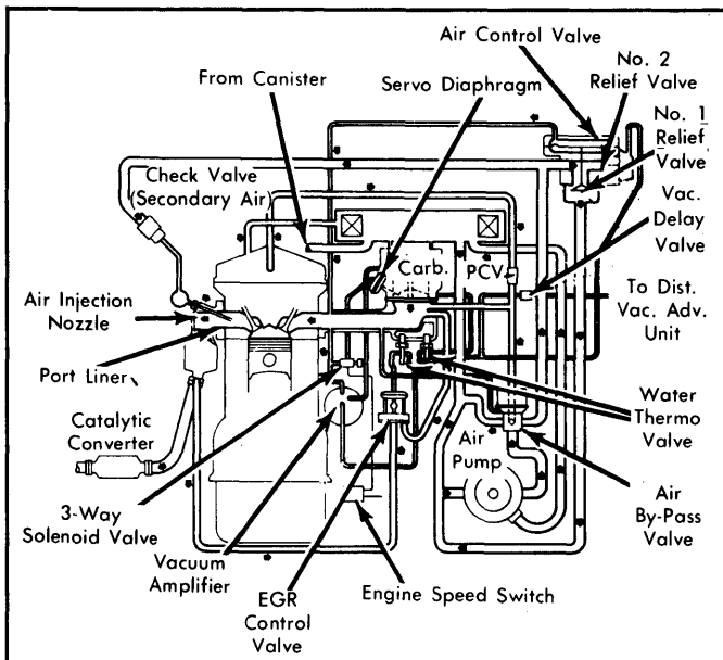
Fig. 9: 1979 2.0L California Exhaust Emission System
