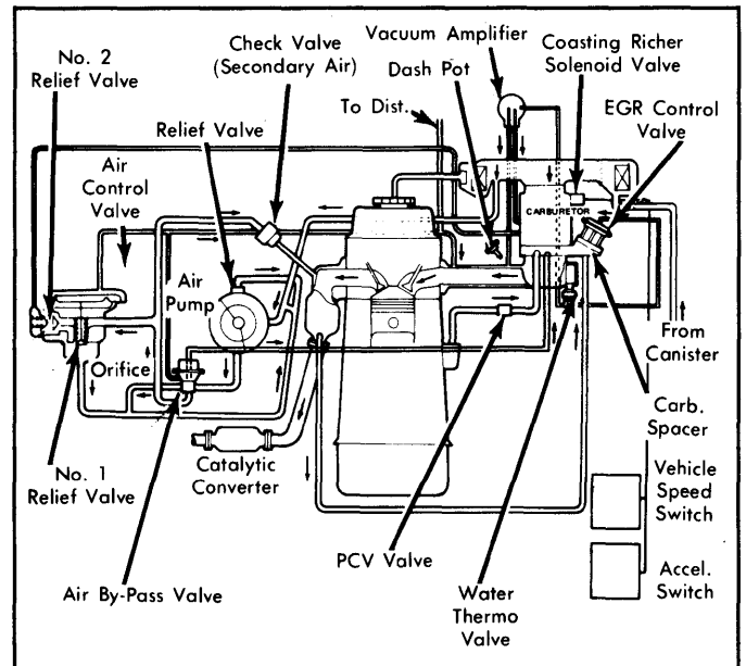
Fig. 11: 1979 2.3L California Exhaust Emission System
