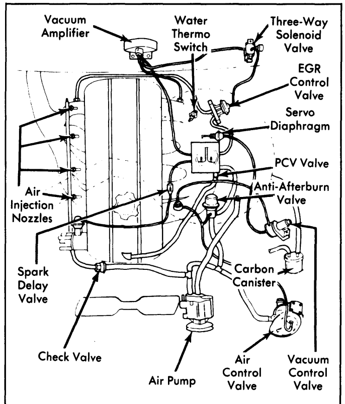
Fig. 3: 1977 1.8L Exhaust Emission System (California)
