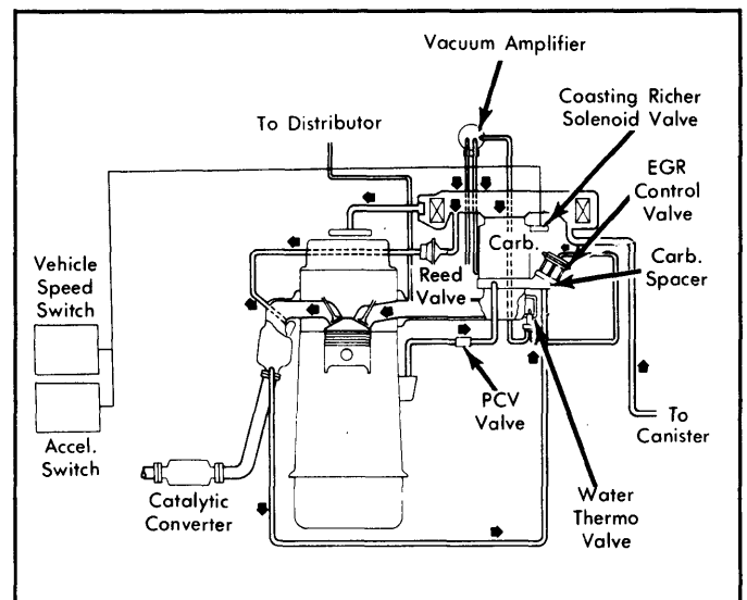
Fig. 10: 1979 2.3L Federal Exhaust Emission System
