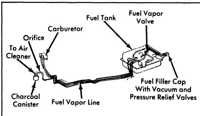
Fig. 7: 1977-78 Fuel Evaporation System
