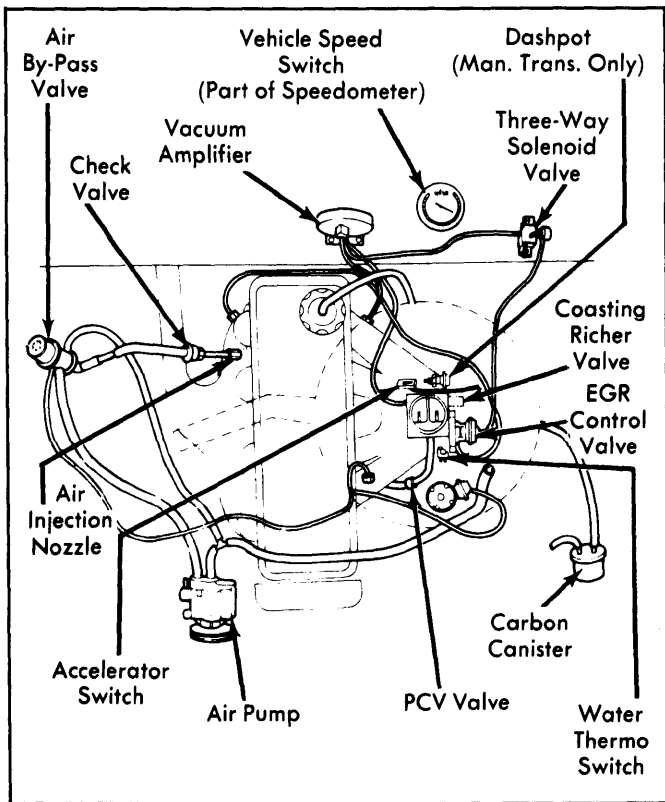
Fig. 4: 1977 2.3L Exhaust Emission System (Except California)
