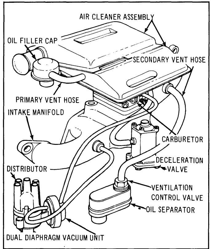
Fig. 14: 1974-76 Positive Crankcase Ventilation System
