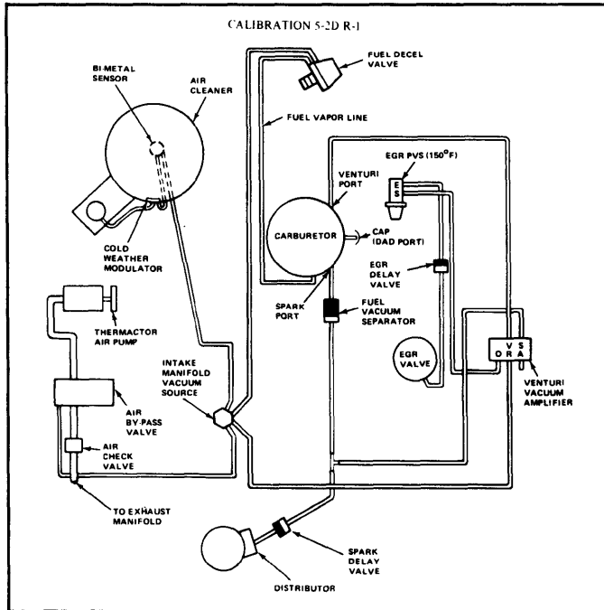
Fig. 7: 1975-78 Vacuum Diagram No. 7
