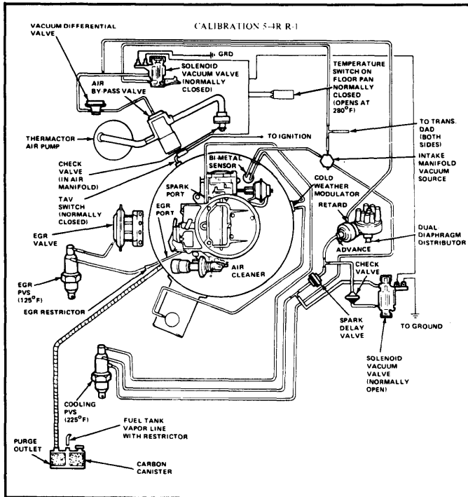
Fig. 11: 1975-78 Vacuum Diagram No. 11
