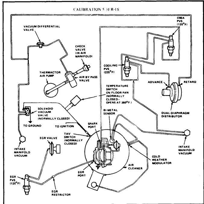
Fig. 9: 1975-78 Vacuum Diagram No. 9
