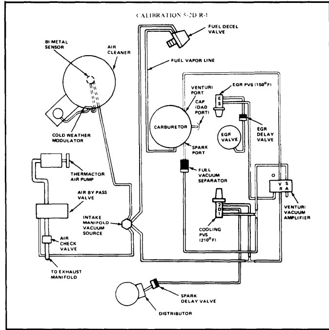
Fig. 8: 1975-78 Vacuum Diagram No. 8
