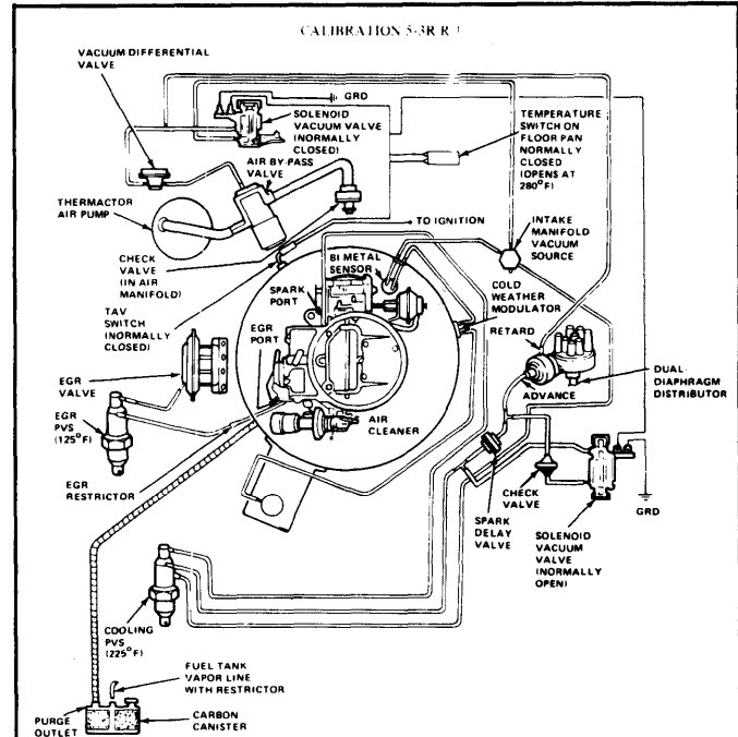
Fig. 10: 1975-78 Vacuum Diagram No. 10
