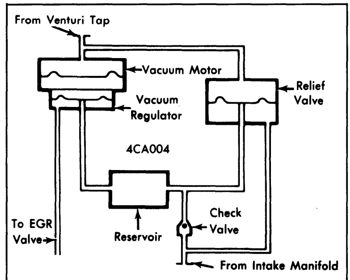
Fig. 13: 1974 EGR/Vacuum Amplifier System
