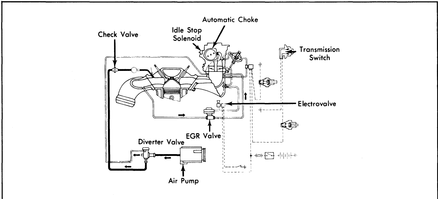
Fig. 11: 1978 124 Spider Exhaust Emission System (Federal)
