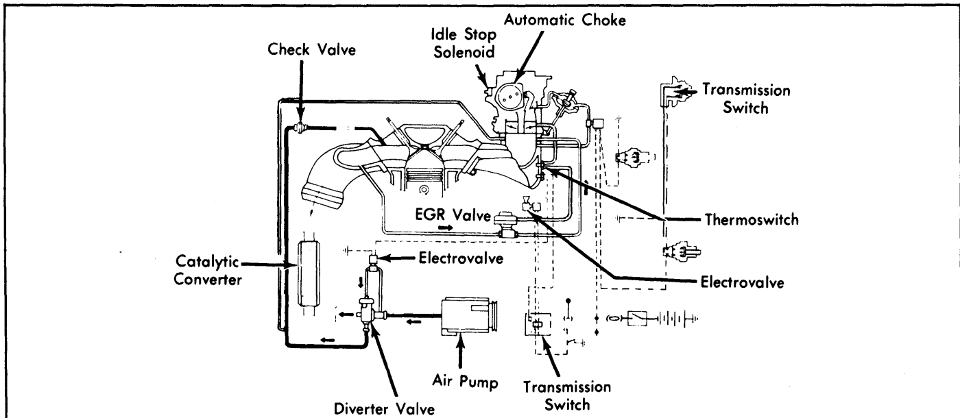
Fig. 10: 1978 124 Spider Exhaust Emission System (California)
