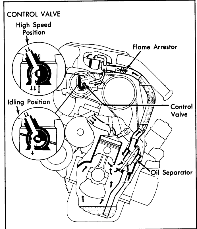
Fig. 3: 1974-79 X1/9 & 128 Positive Crankcase Ventilation System
