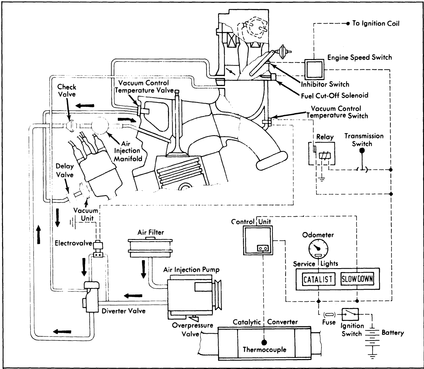
Fig. 7: 1975 128 & X1/9 Exhaust Emission System (California)
