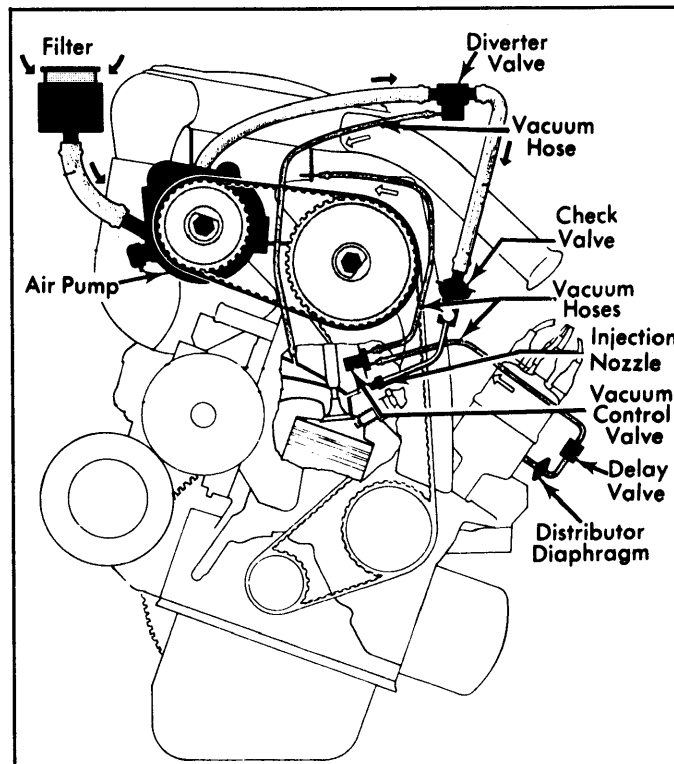
Fig. 2: 1974 X1/9 & 128 Exhaust Emission System
