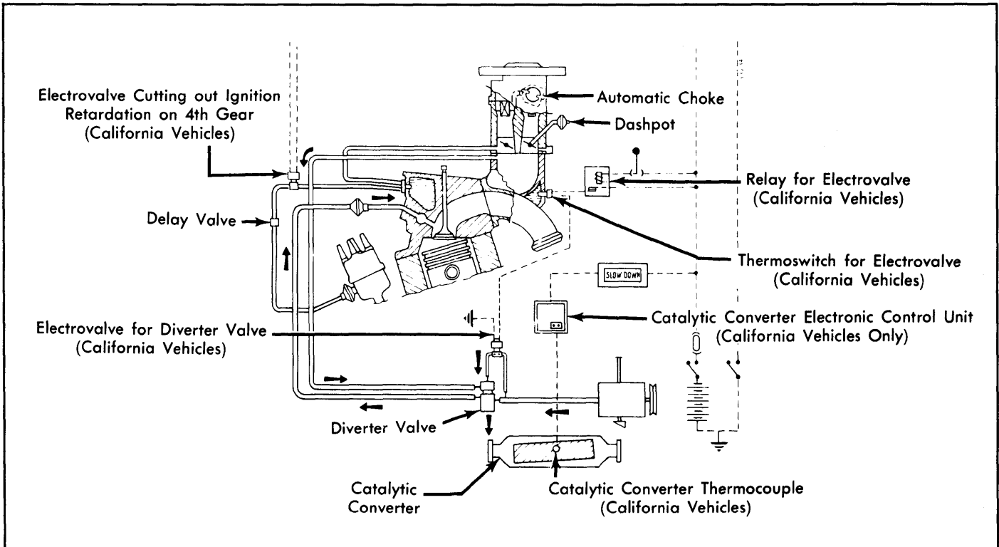
Fig. 13: 1978 X1/9 Exhaust Emission System
