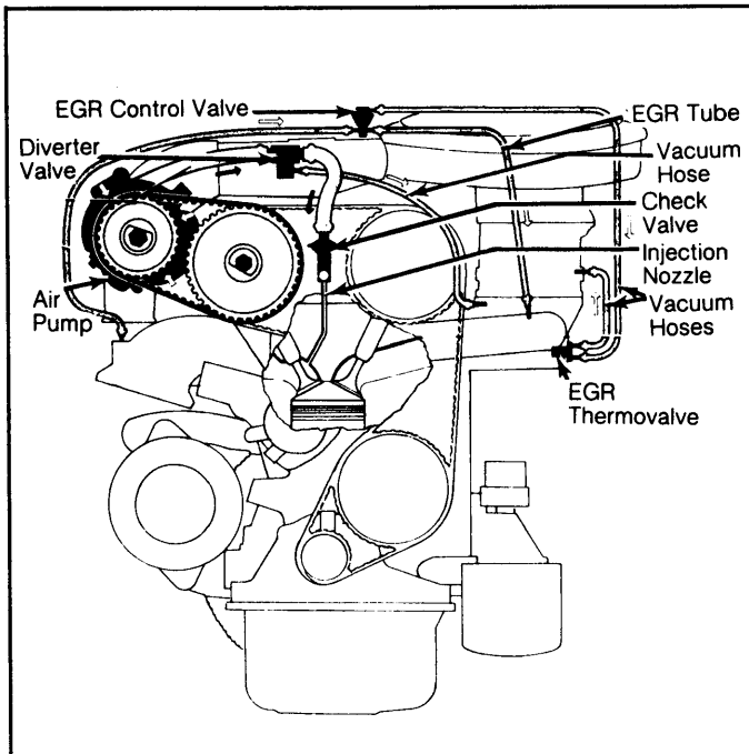
Fig. 1: 1974 124 Exhaust Emission System
