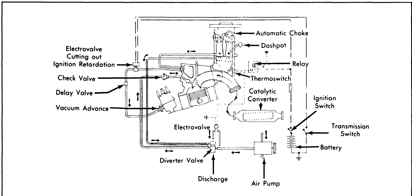
Fig. 12: 1978 128 Exhaust Emission System (California)
