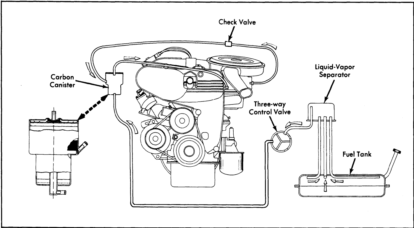
Fig. 9: 1977 124 Fuel Evaporation System
