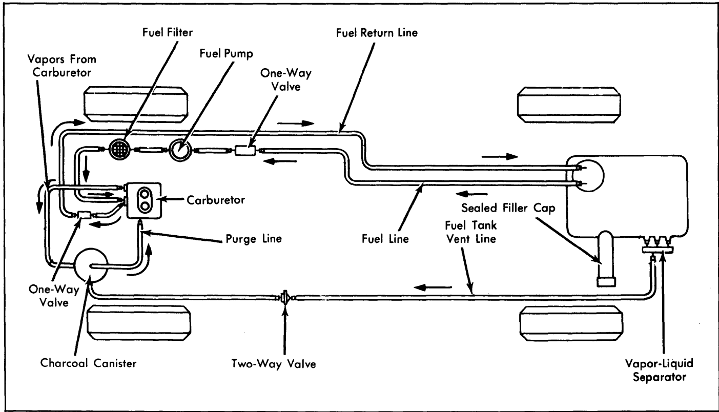
Fig. 14: 1978 X1/9 Fuel Evaporation System
