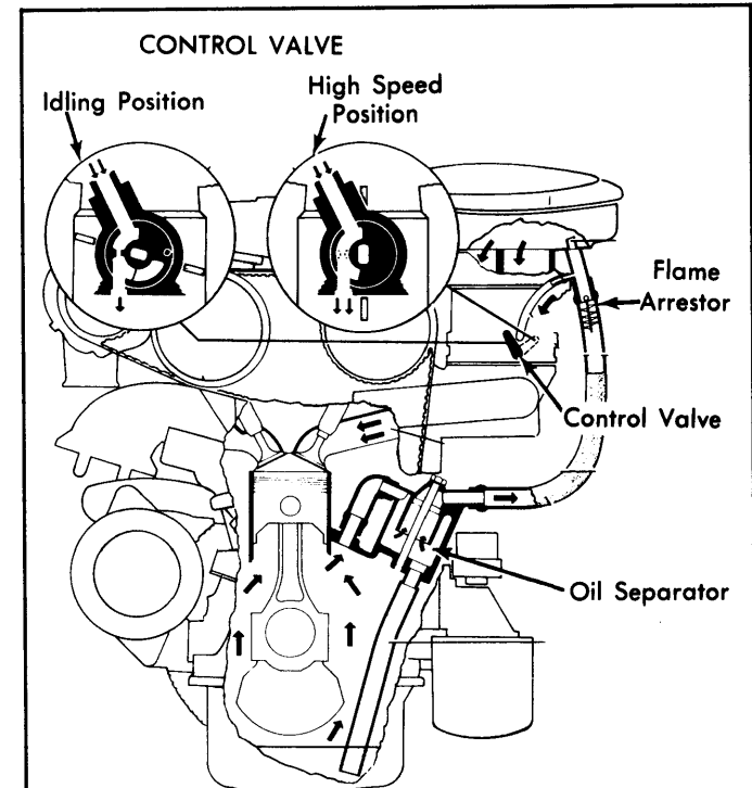
Fig. 4: 1974-75 124 Positive Crankcase Ventilation System
