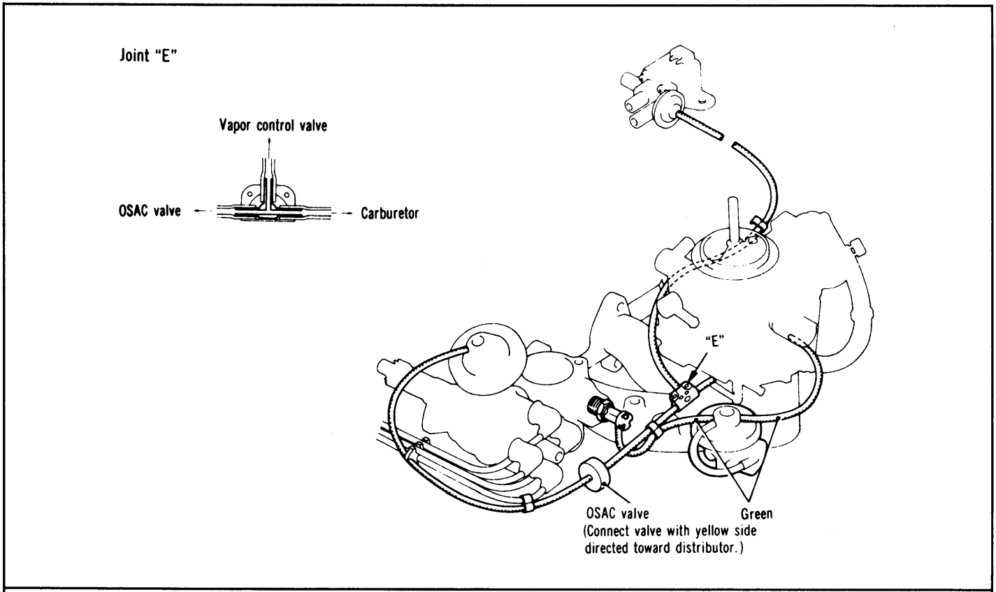
Fig. 18: 1977 Arrow & Colt (2000cc Engine) Exhaust Emission System (Federal)
