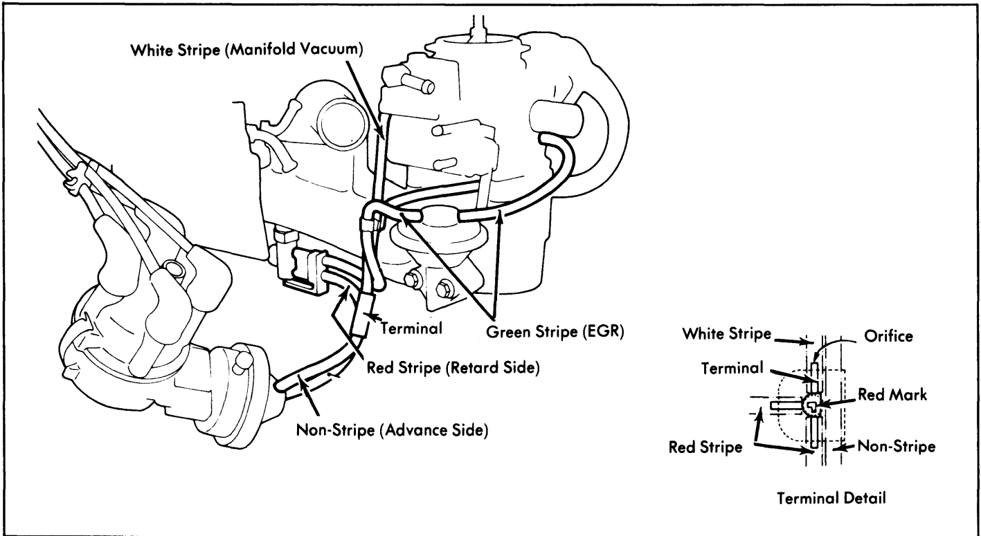
Fig. 5: 1976 Arrow & Colt (1600cc Engine) Exhaust Emission System
