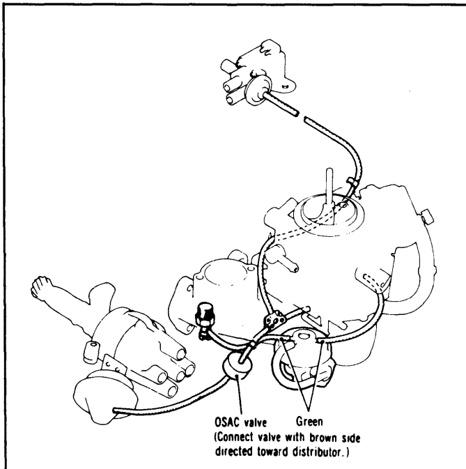
Fig. 16: 1977 Arrow & Colt (1600cc Engine) Exhaust Emission System (Federal Man. Trans.)
