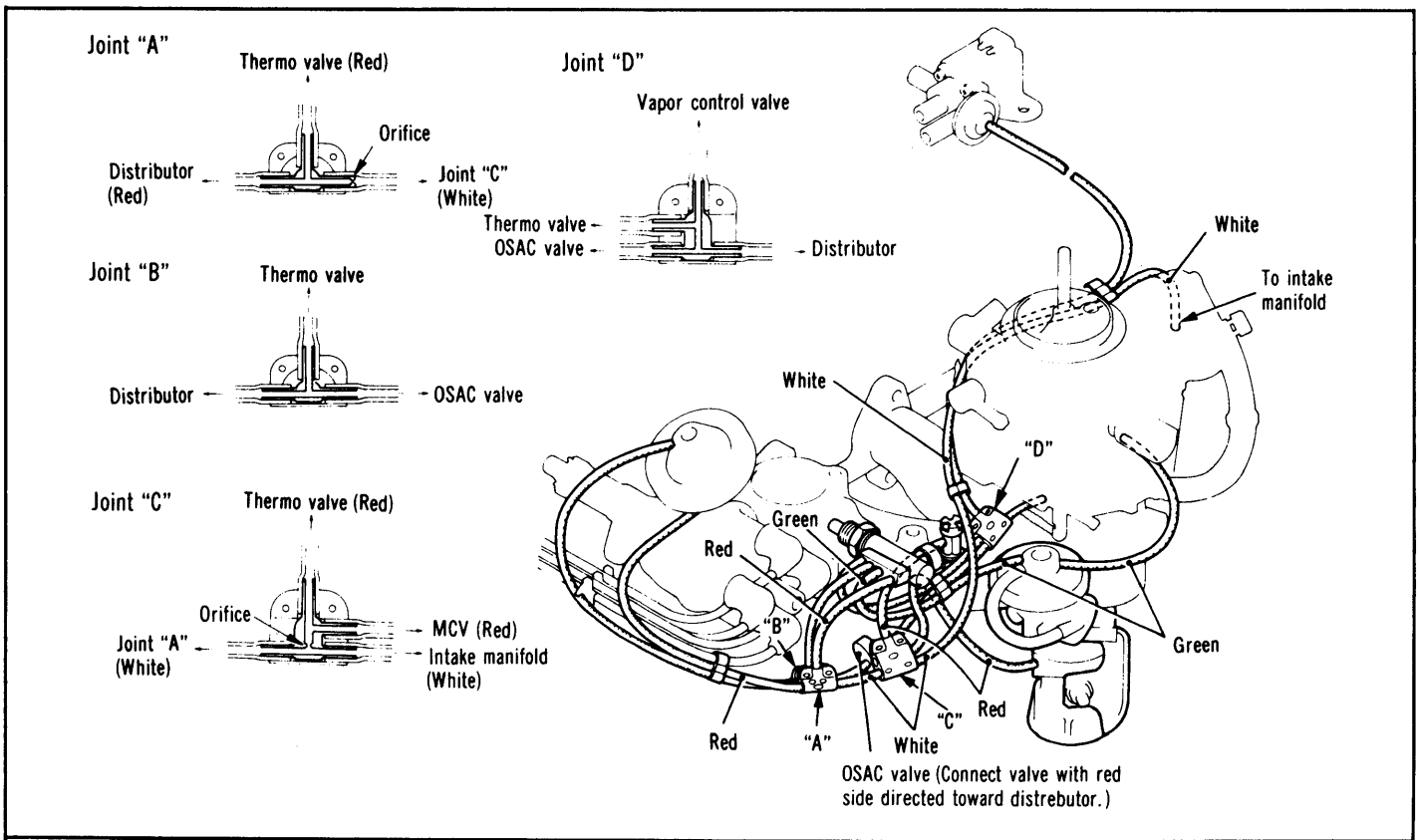
Fig. 19: 1977 Arrow & Colt (2000cc Engine) Exhaust Emission System (California Man. Trans.)
