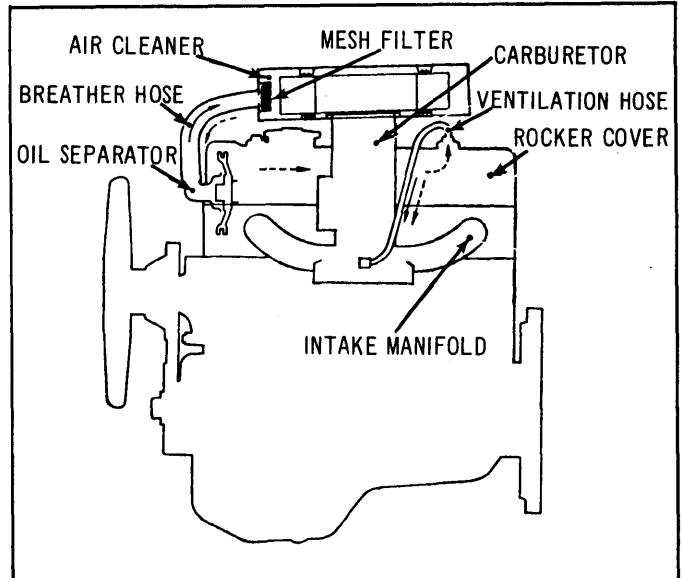
Fig. 3: 1974-75 Colt Positive Crankcase Ventilation System
