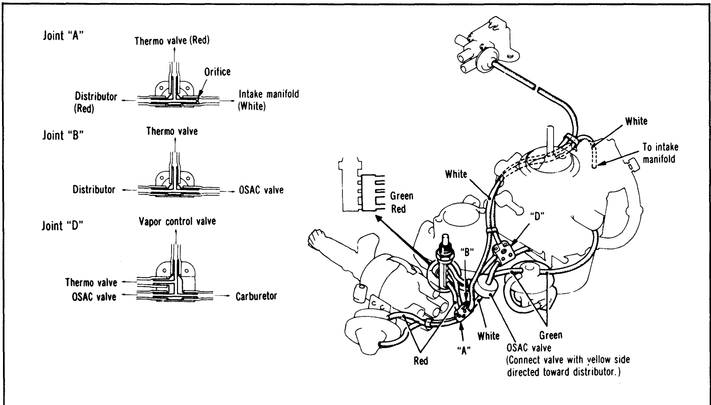
Fig. 15: 1977 Arrow & Colt (1600cc Engine) Exhaust Emission System (California & High Altitude Auto. Trans.)
