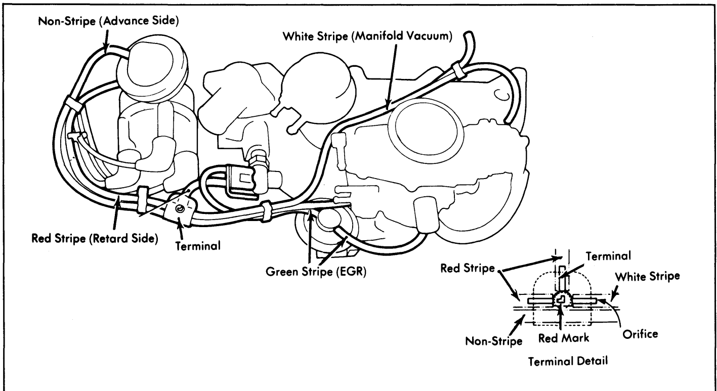
Fig. 6: 1976 Arrow (2000cc Engine) Exhaust Emission System
