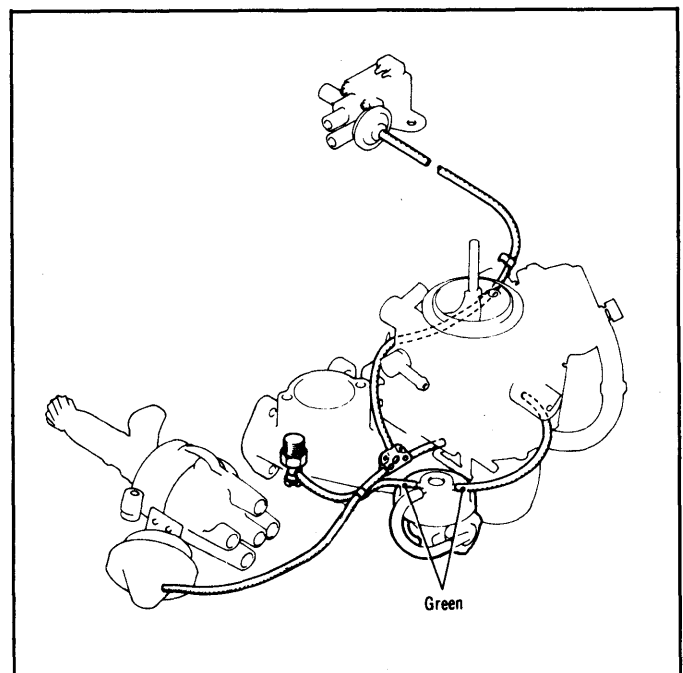
Fig. 17: 1977 Arrow & Colt (1600cc Engine) Exhaust Emission System (Federal Auto. Trans.)
