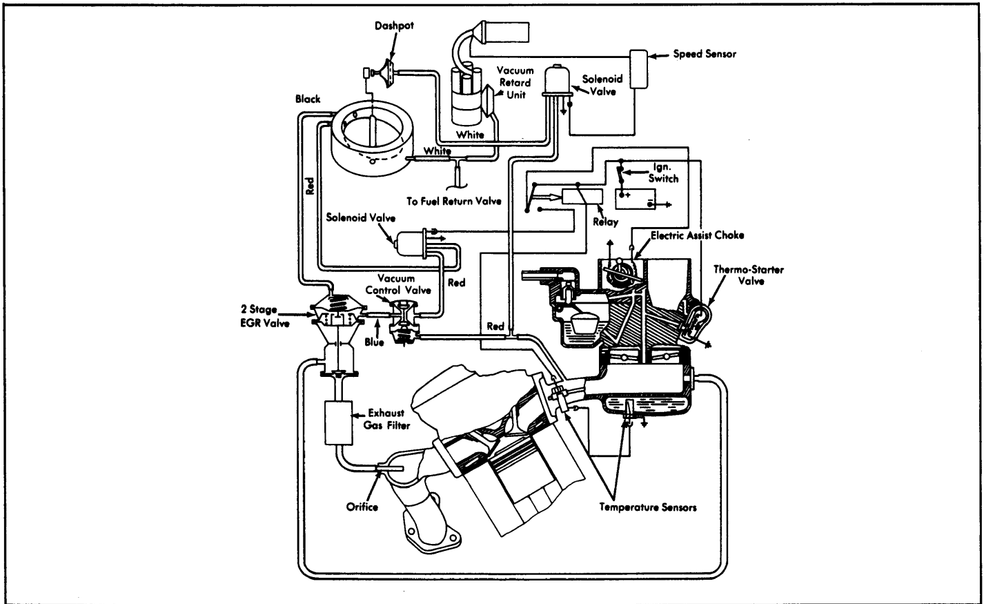
Fig. 1: 1974 2002 Exhaust Emission System
