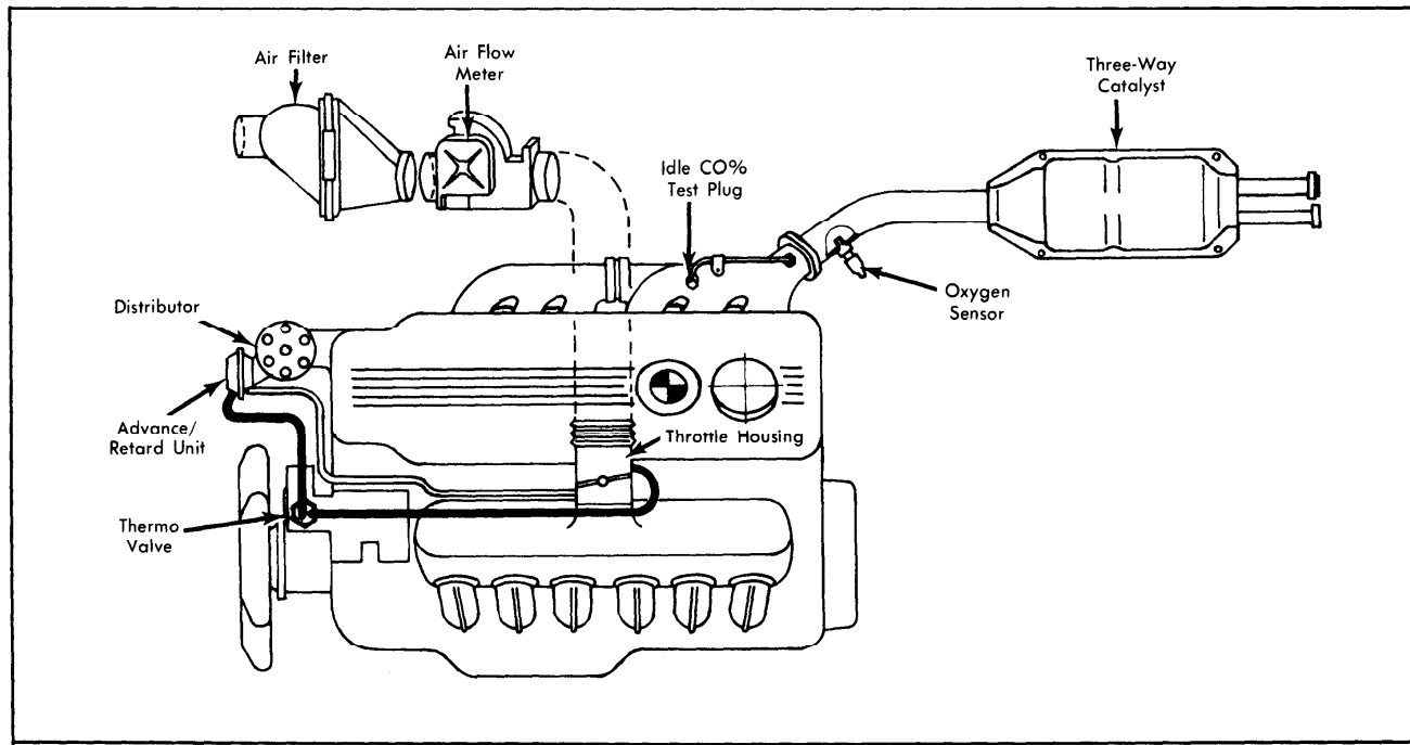
Fig. 22: 1979 528i Exhaust Emission System
