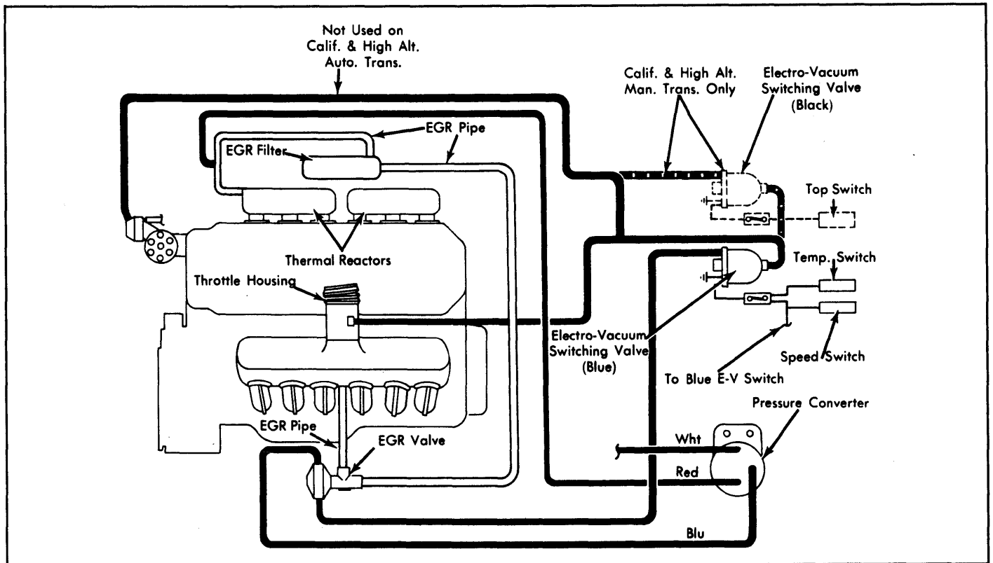
Fig. 19: 1978 733i Exhaust Gas Recirculation System
