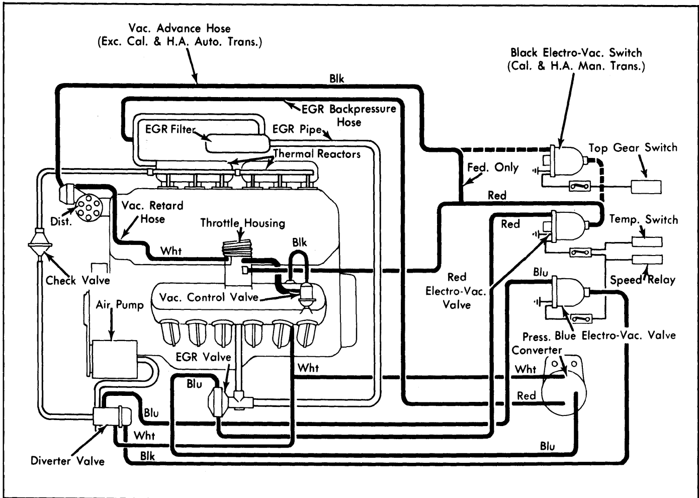
Fig. 17: 1978 733i Exhaust Emission System
