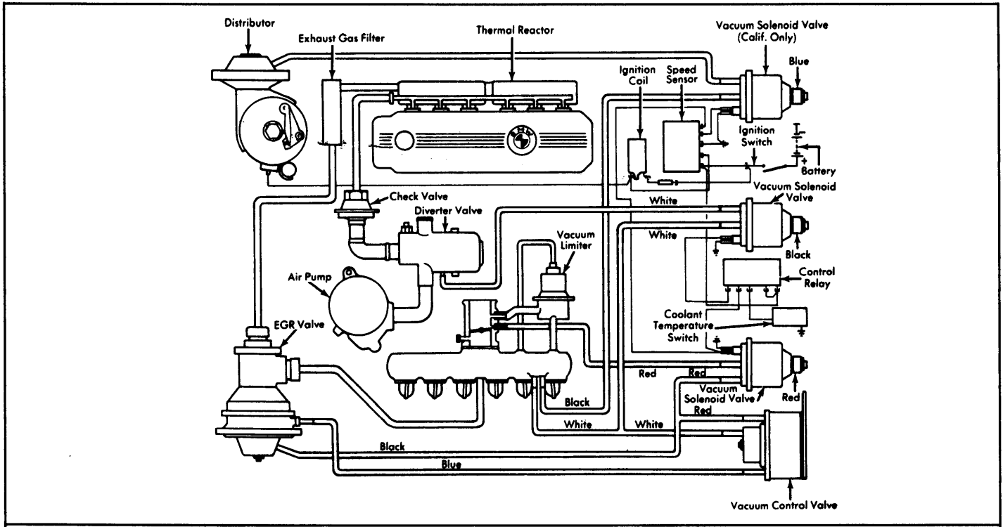
Fig. 5: 1975 530i & 3.0Si Exhaust Emission System
