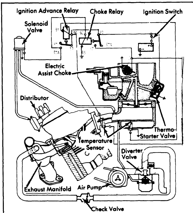
Fig. 10: 1976 2002 Exhaust Emission System (Federal)
