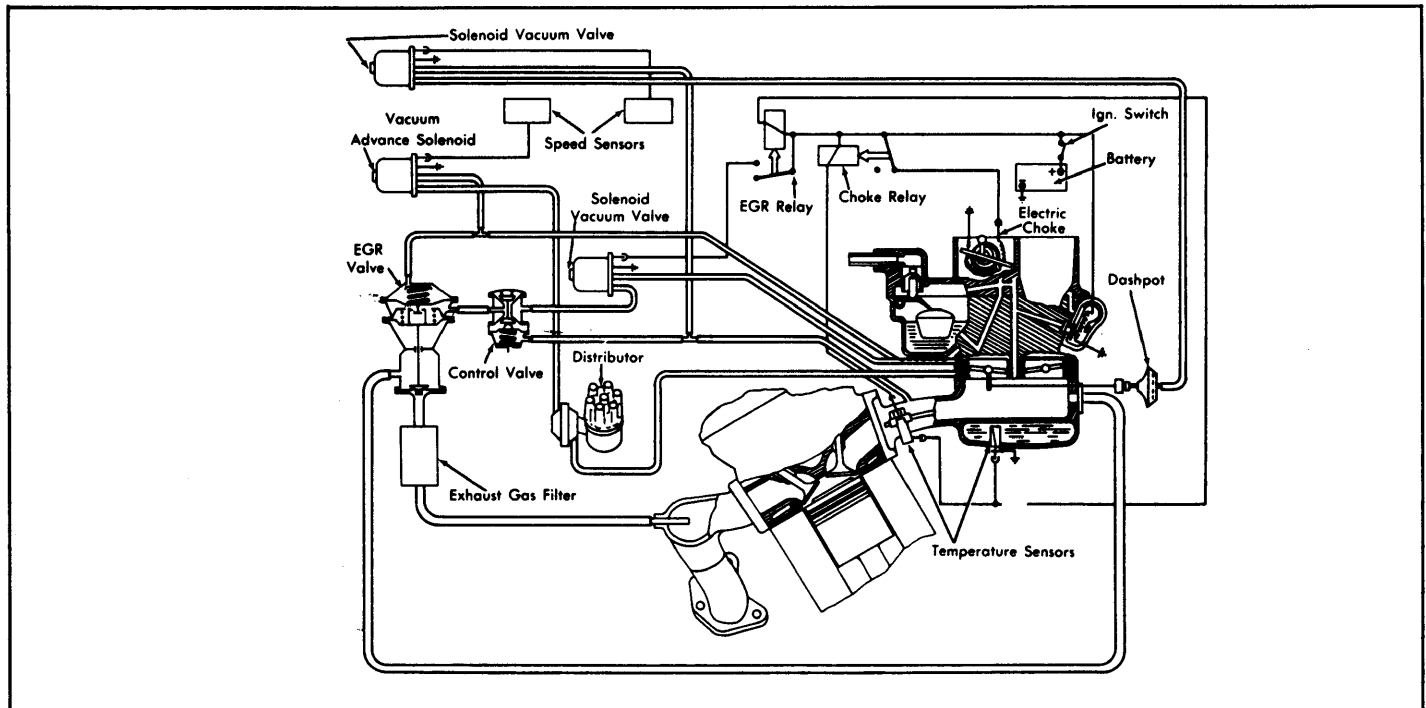
Fig. 2: 1974 Bavaria, 3.0CS & Sedan Exhaust Emission System
