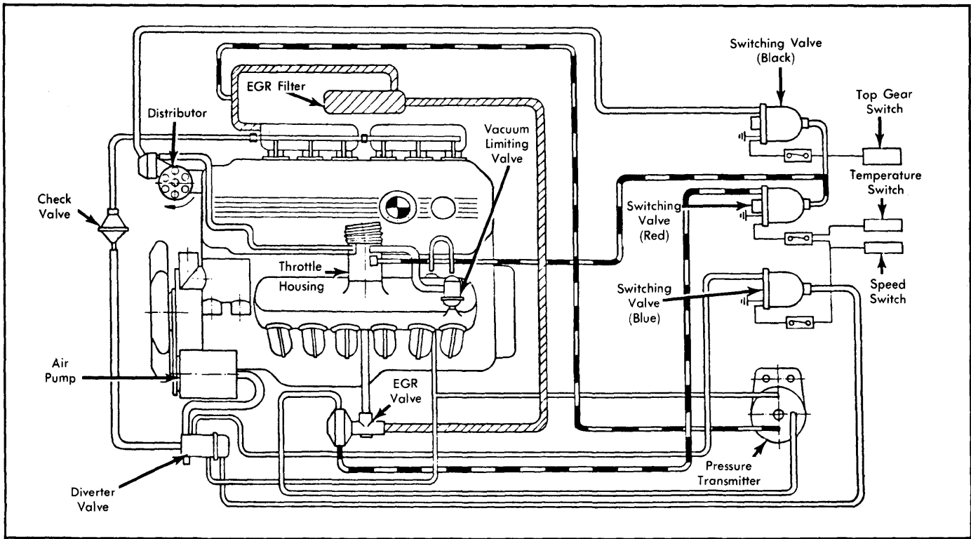
Fig. 25: 1979 633CSI & 733i Exhaust Emission System (California & High Alt. With Man. Trans.)
