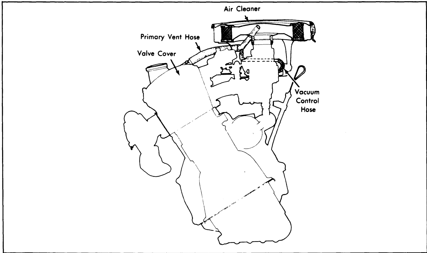
Fig. 4: 1974-76 Positive Crankcase Ventilation System
