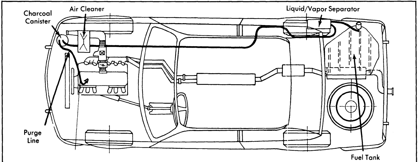
Fig. 14: 1977-78 530i Fuel Evaporation System (633CSI Similar)
