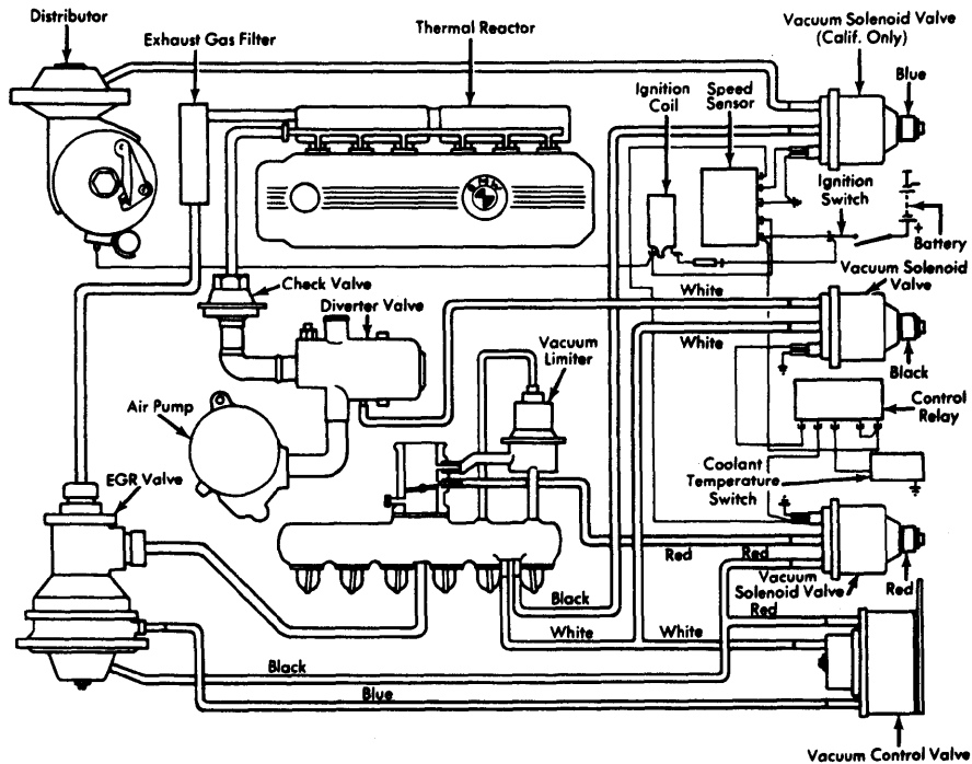
Fig. 8: 1976 530i & 3.0Si Exhaust Emission System
