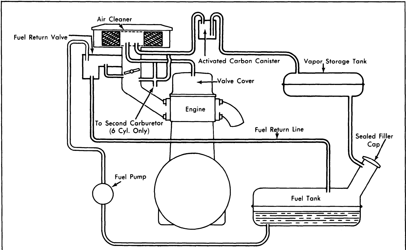
Fig. 3: 1974-76 2002 Fuel Evaporation System
