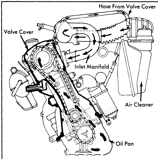
Fig. 15: 1977-78 320i Positive Crankcase Ventilation System
