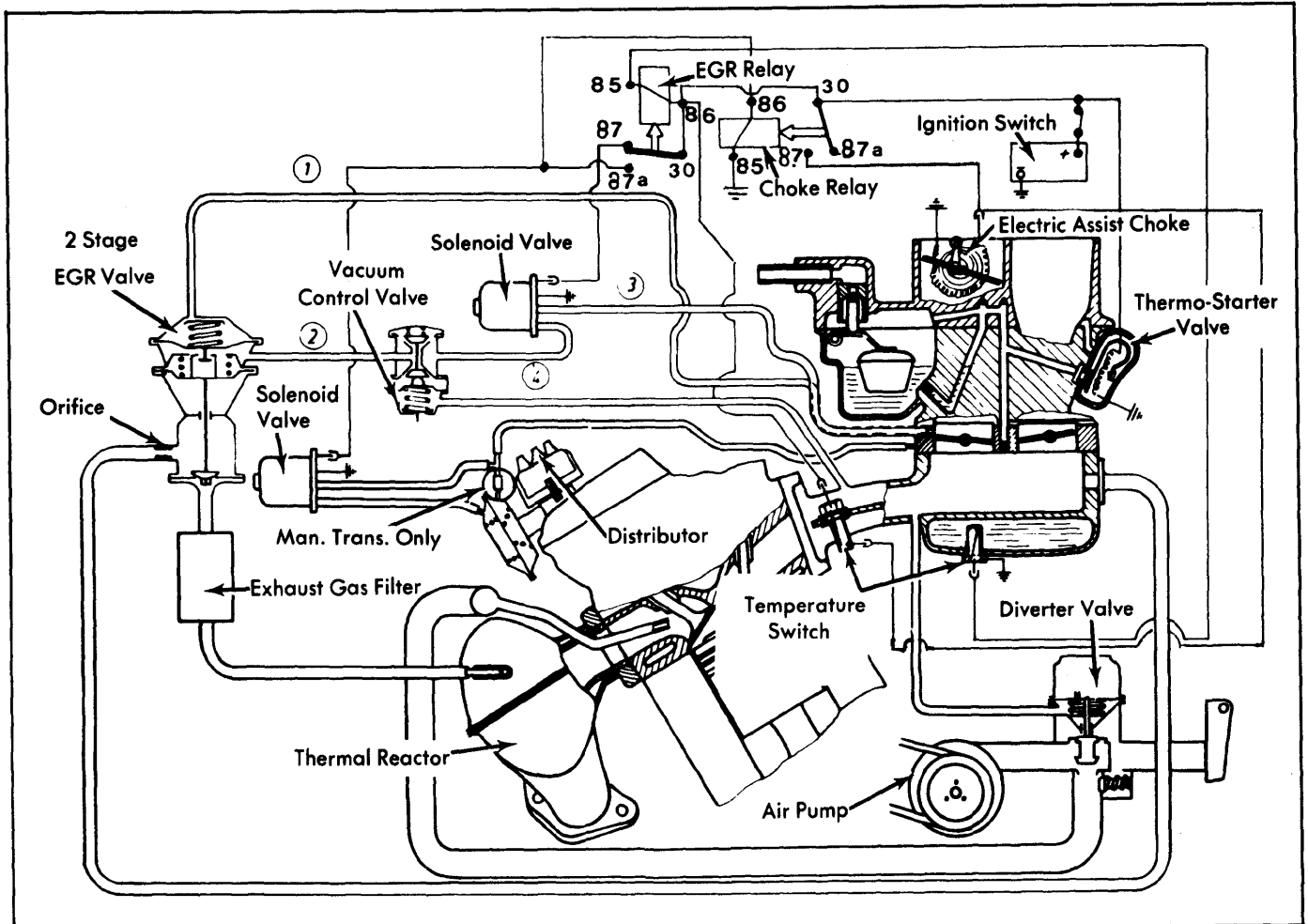
Fig. 9: 1976 2002 Exhaust Emission System (California)
