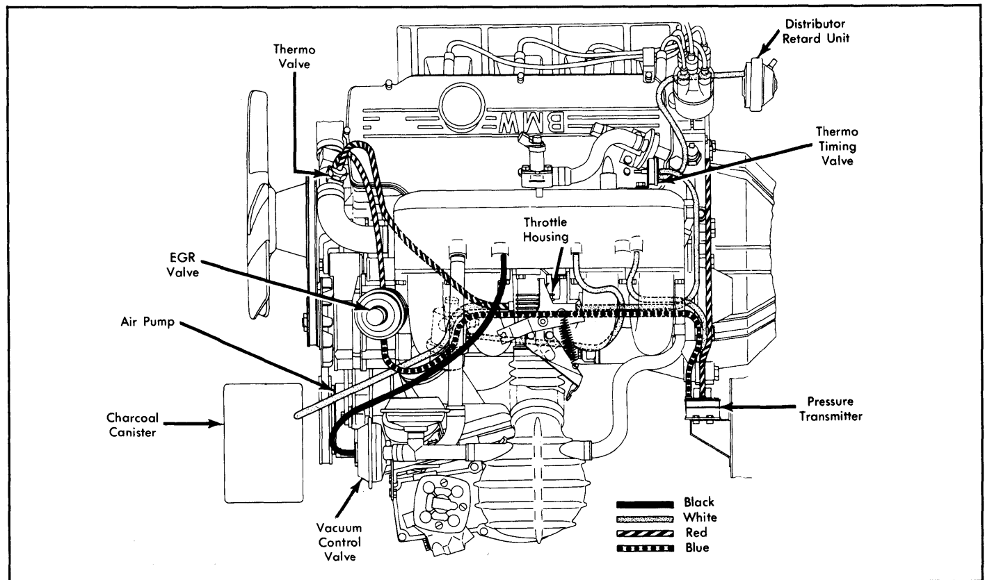
Fig. 20: 1979 320i Exhaust Emission System (Auto. Trans.)
