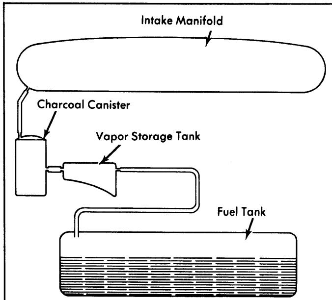
Fig. 6: 1975-76 530i & 3.0Si Fuel Evaporation System
