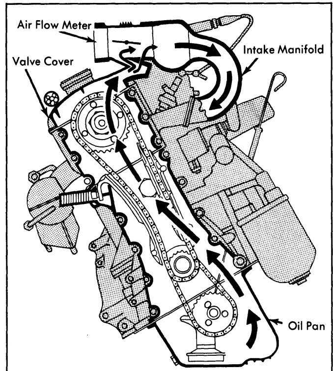
Fig. 16: 1977-78 530i Positive Crankcase Ventilation System
