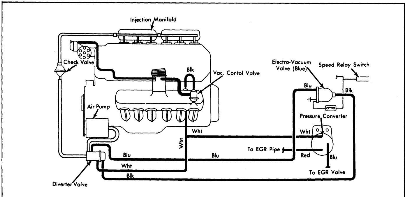
Fig. 18: 1978 733i Air Injection System
