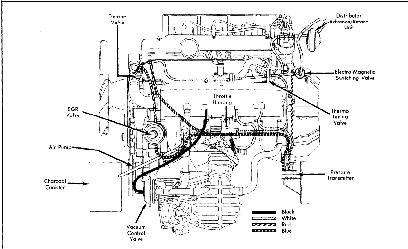
Fig. 21: 1979 320i Exhaust Emission System (Man. Trans.)
