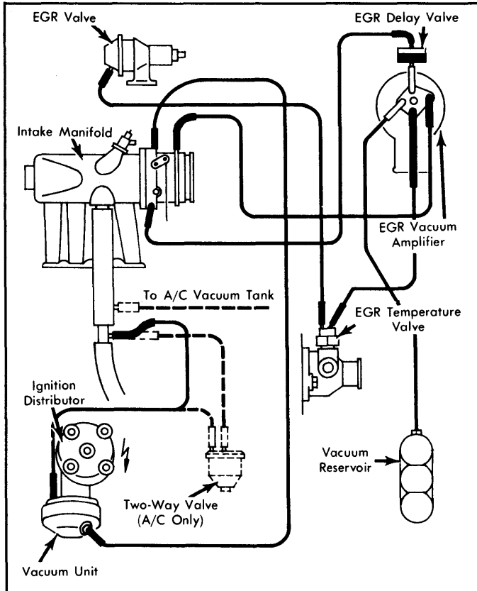
Fig. 14: 1979 Fox Exhaust Emission System (Auto. Trans. Models)
