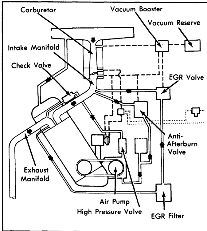
Fig. 1: 1974 100LS Exhaust Emission System
