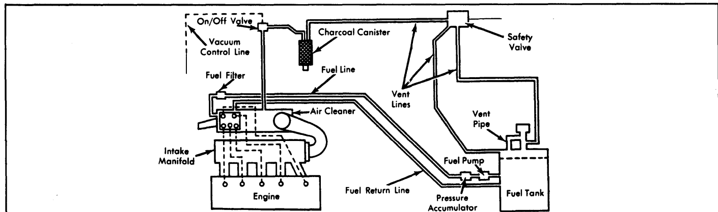
Fig. 12: 1978 5000 Fuel Evaporation System
