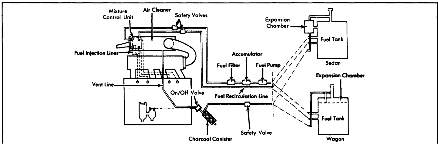
Fig. 11: 1978 Fox Fuel Evaporation System
