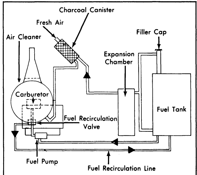
Fig. 3: 1974-77 100LS Fuel Evaporation System
