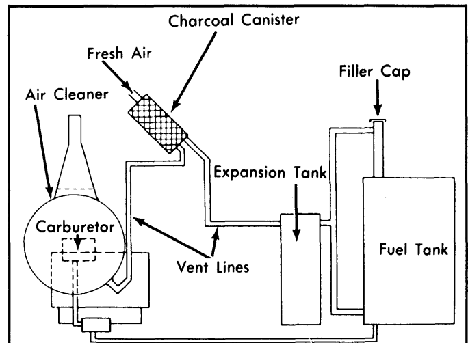
Fig. 4: 1974-75 Fox Fuel Evaporation System
