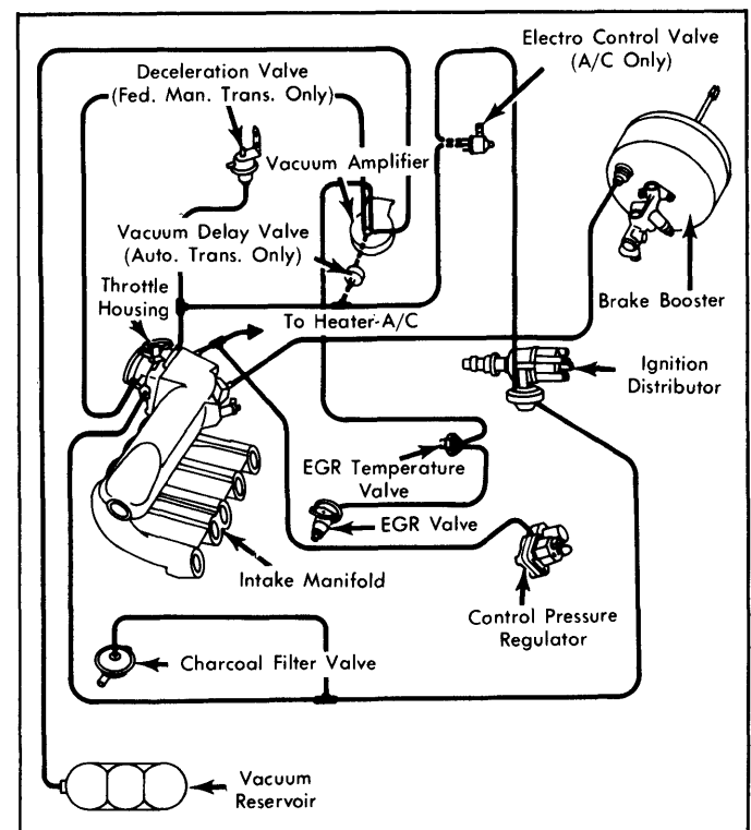
Fig. 17: 1979 5000 Exhaust Emission System
