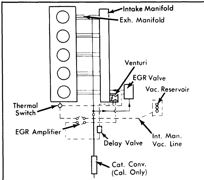
Fig. 10: 1978 5000 Exhaust Emission System
