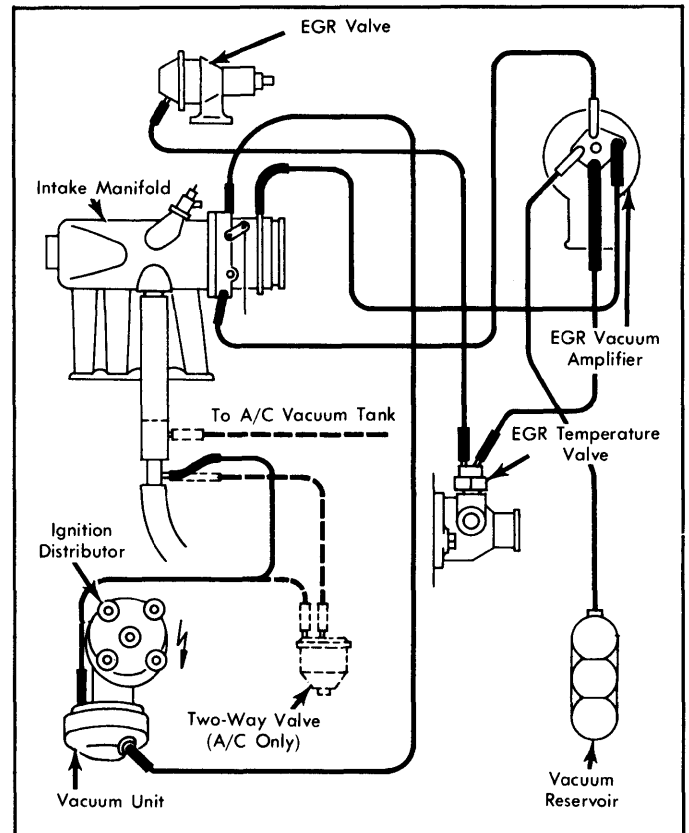
Fig. 16: 1979 Fox Exhaust Emission System (California Models With Man. Trans.)
