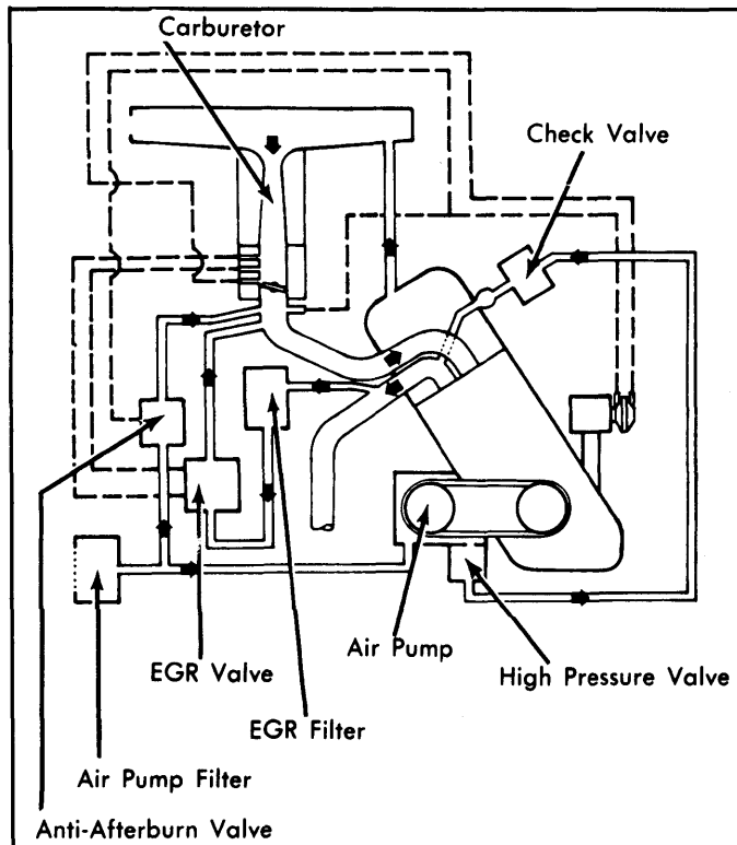
Fig. 2: 1974 Fox Exhaust Emission System
