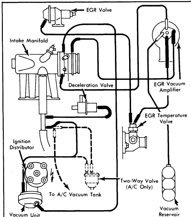
Fig. 15: 1979 Fox Exhaust Emission System (Federal Models With Man. Trans.)
