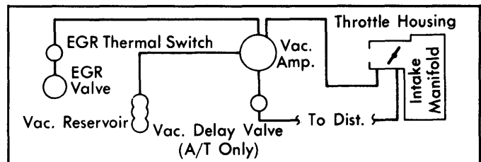
Fig. 13: 1978 5000 Exhaust Gas Recirculation System
