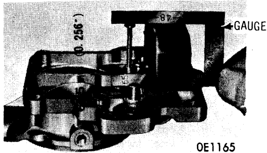
MEASURING FLOAT LEVEL (RAISED)
