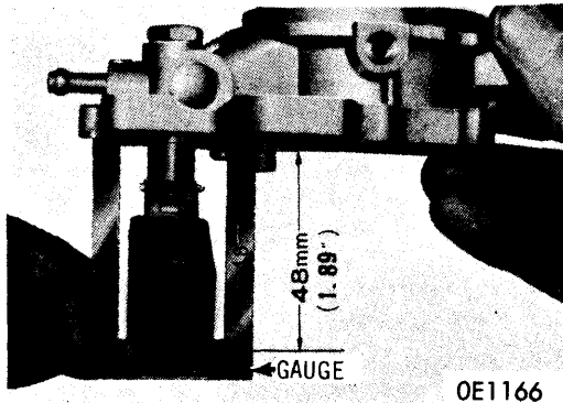
MEASURING FLOAT DROP (LOWERED)
