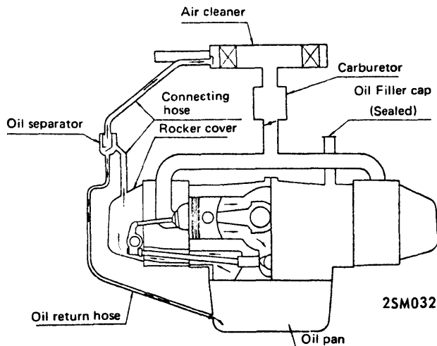
1100 MODEL CRANKCASE VENTILATION SYSTEM
