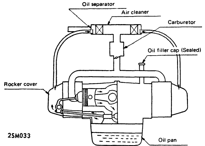
1300G & 1400 CRANKCASE VENTILATION SYSTEM
