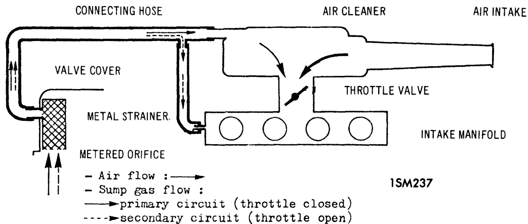
PEUGEOT 304 CRANKCASE VENTILATION SYSTEM
