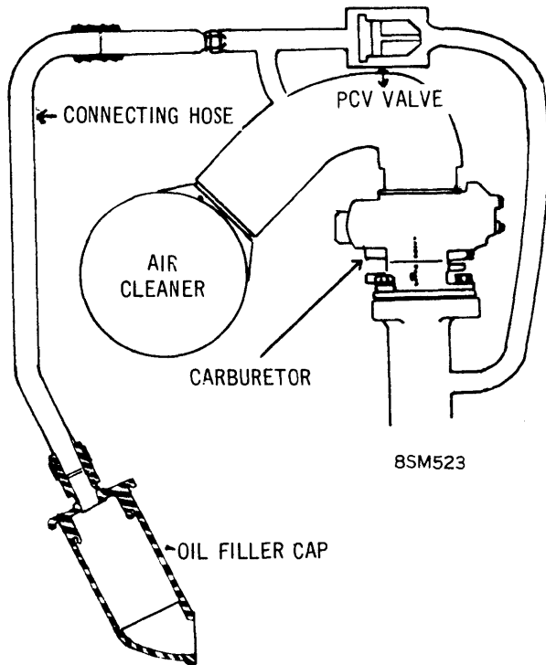
PEUGEOT 404 CRANKCASE VENTILATION SYSTEM
