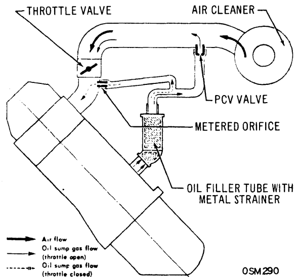
PEUGEOT 504 CRANKCASE VENTILATION SYSTEM
