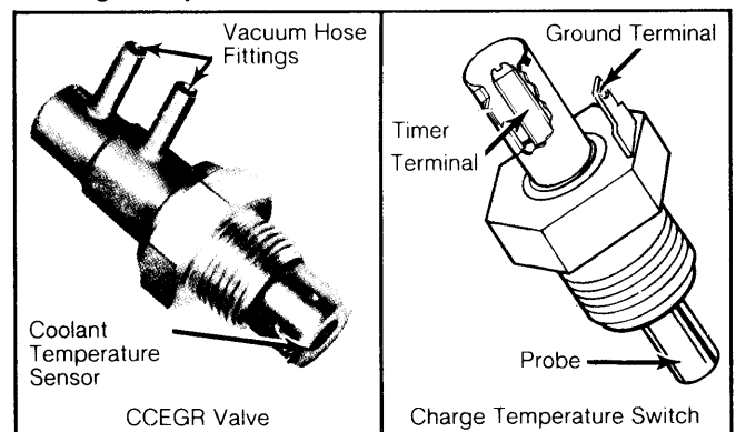
Fig. 2: Typical CCEGR Valve & Charge Temperature Switch
