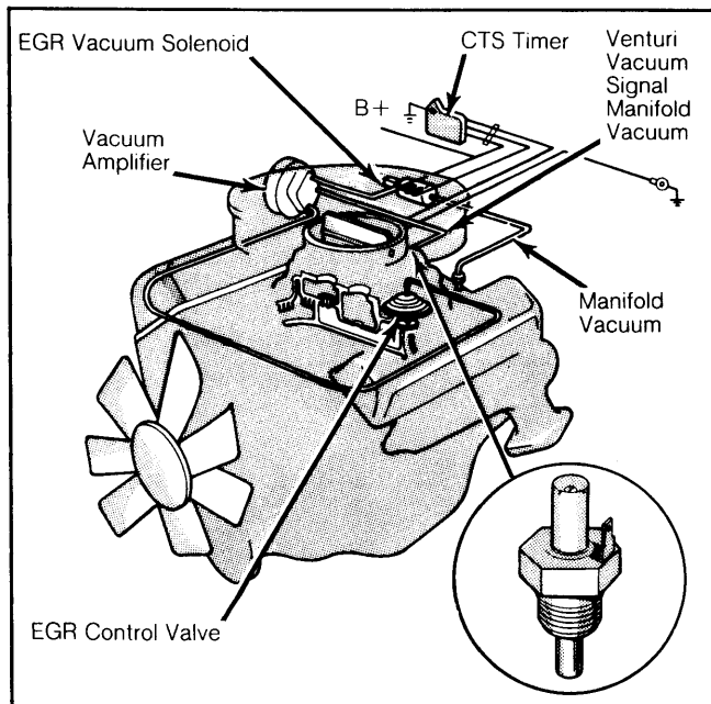
Fig. 1: Chrysler Corp. Exhaust Gas Recirculation System
