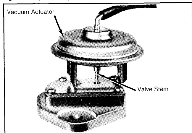
Fig. 3: Chrysler Corp. Vacuum-Actuated EGR Valve
