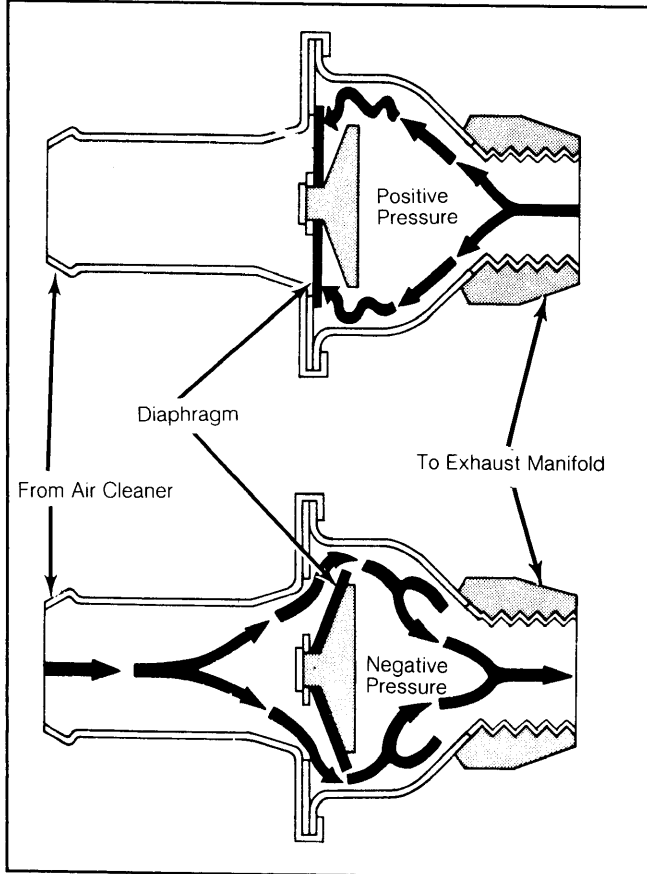
Fig. 1: Chrysler Corp. Aspirator Valve Air Flow
