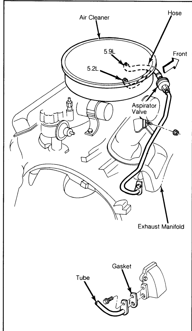
Fig. 2: Chrysler Corp. Aspirator Air System Assembly (V8 Shown - 6-Cylinder Similar)
