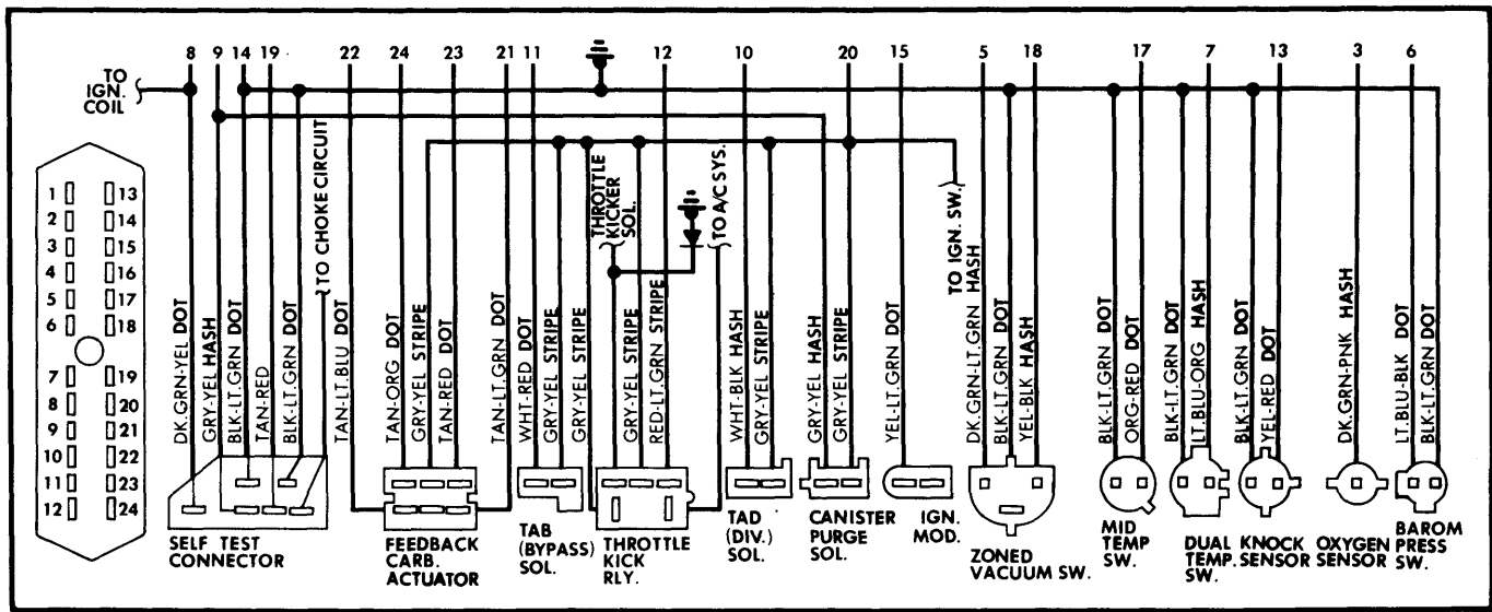
Fig. 5 V6 MCU System Wiring Diagram
