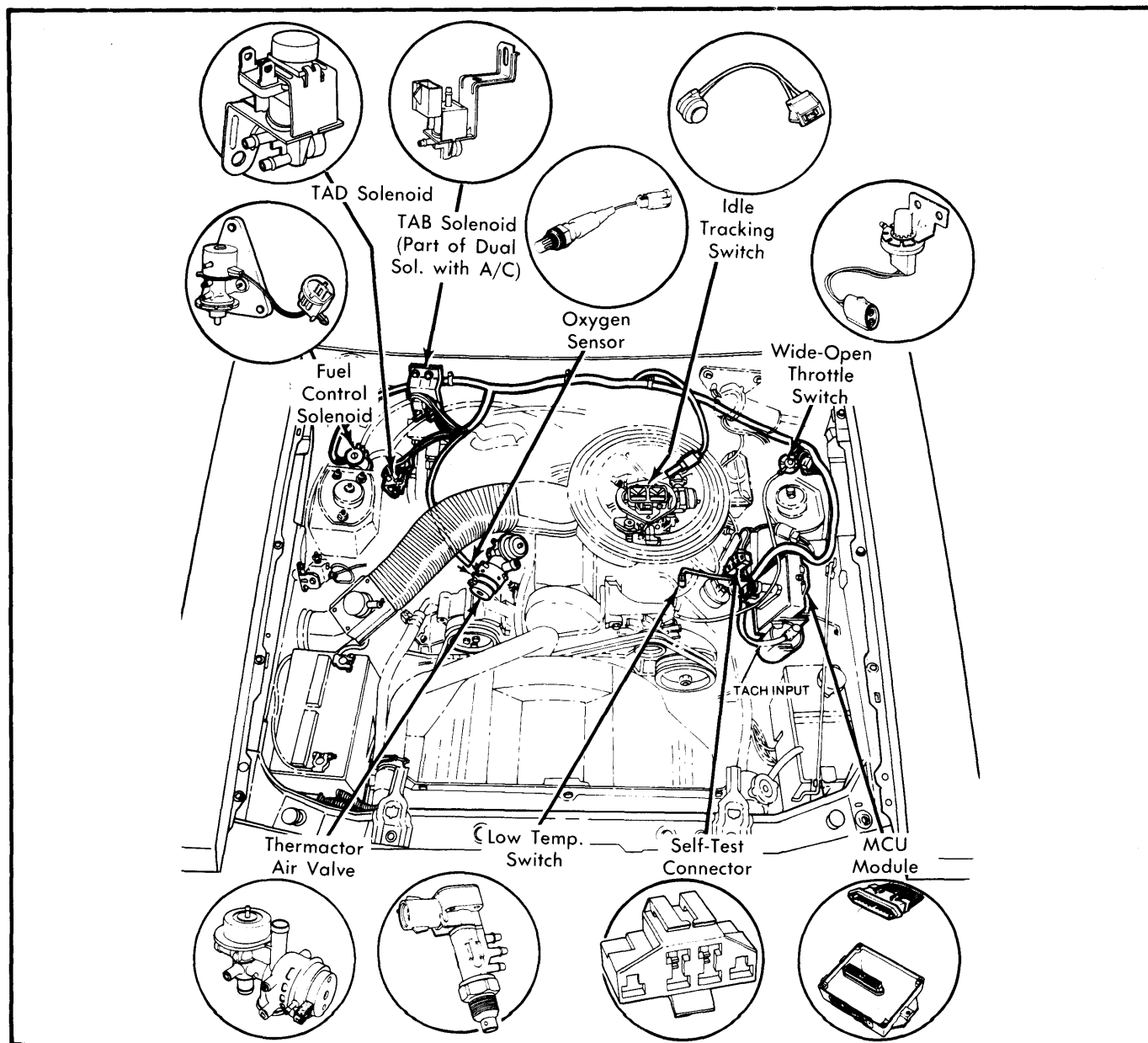
Fig. 1 4-Cylinder MCU System Layout
