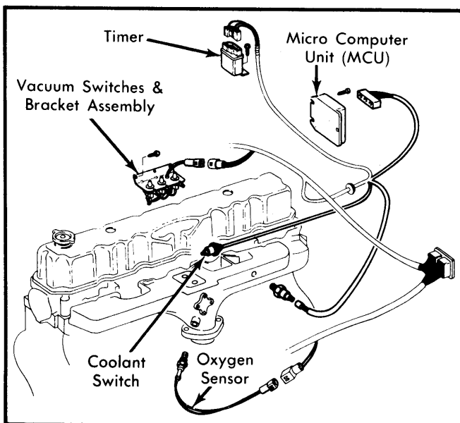
Fig. 1 American Motors 6-Cyl. CEC System
