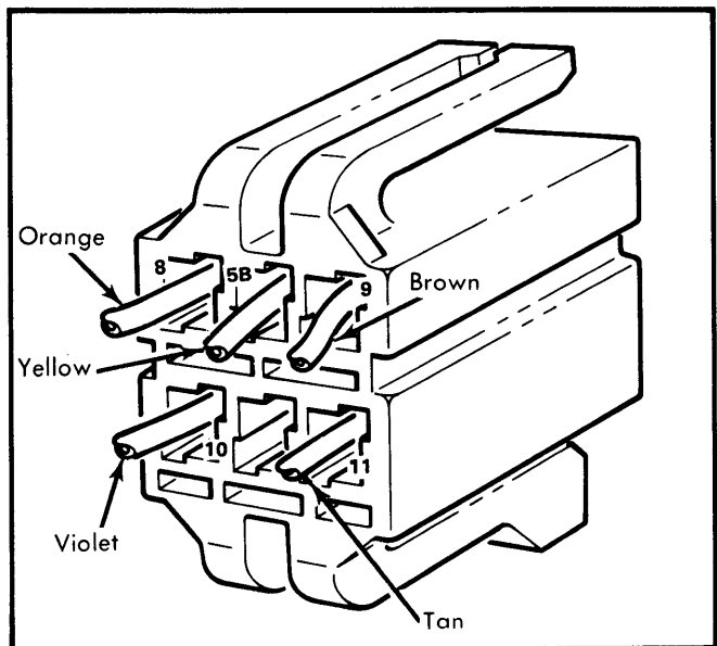
Fig. 4 Stepper Motor Connector Terminal Identification
