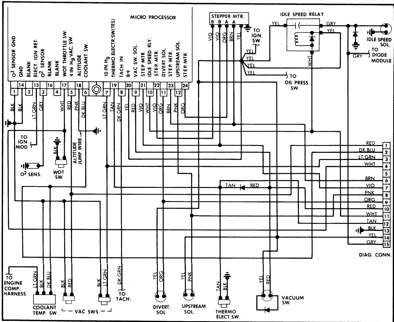
Fig. 3 American Motors 6-Cyl. CEC System Wiring Diagram
