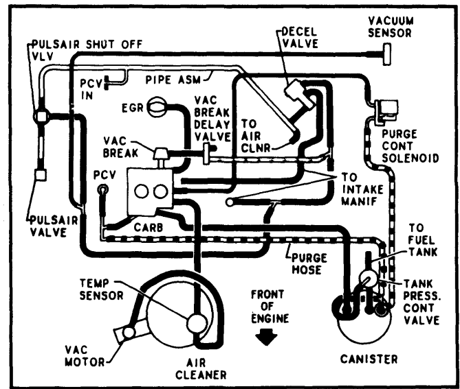
Fig. 2 1.6L (98") 4 Cyl. 2-Bbl. VIN C Calif. Auto. & Man. Trans.
