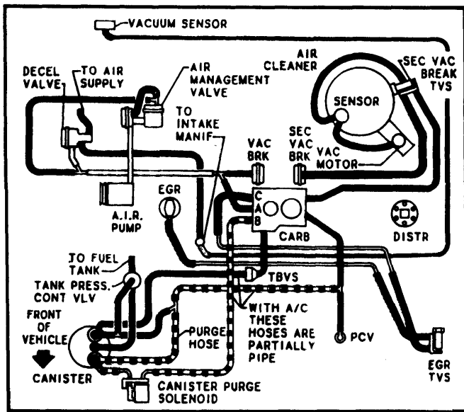
Fig. 9 2.8L (173") V6 2-Bbl. VIN X Federal, Calif. Man. Trans.
