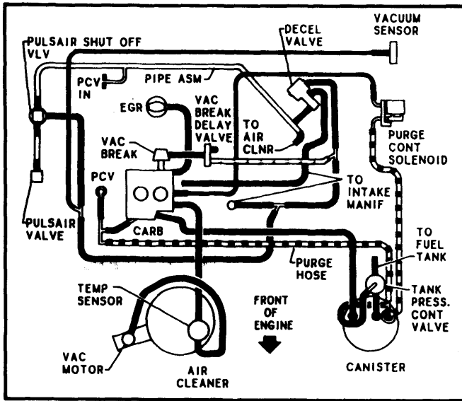
Fig. 1 1.6L (98") 4 Cyl. 2-Bbl. VIN C Federal Auto. & Man. Trans.
