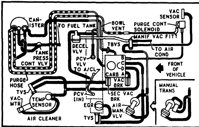
Fig. 3 1.8L (112") 4 Cyl. 2-Bbl. VIN G Federal Auto. & Man. Trans.
