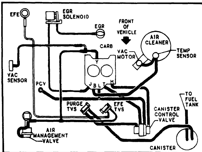
Fig. 11 3.8L (229") V6 2-Bbl. Federal Auto. Trans.
