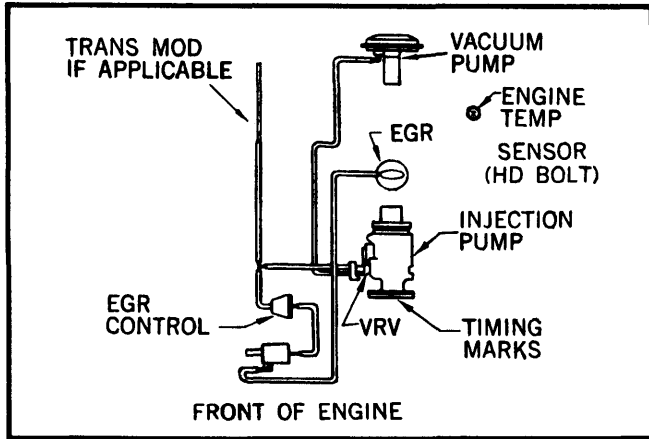
Fig. 19 5.7L (350") V8 Diesel VIN N Federal Auto. Trans.
