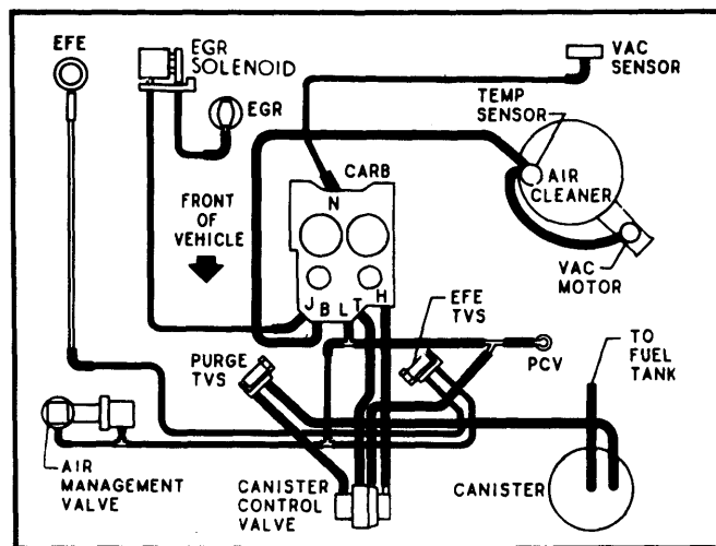
Fig. 17 5.0L (305'') V8 4-Bbl. VIN H Federal Man. Trans.
