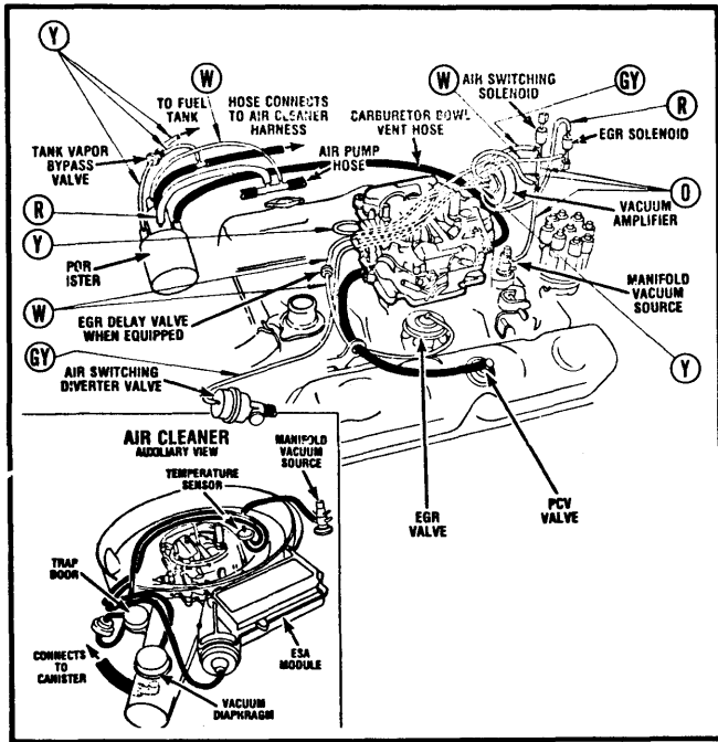
Fig. 5 1981 5.2L (318") V8 4-Bbl.; Federal & Calif. (Cordoba, Diplomat, Mirada, New Yorker)
