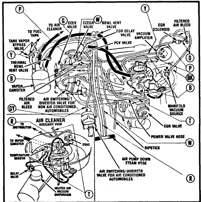
Fig. 2 1981 3.7L (225") 6-Cyl. Federal (Cordoba, Diplomat, Mirada, New Yorker)
