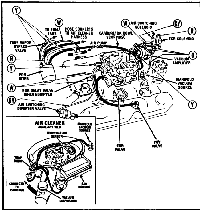
Fig. 7 1982 5.2L (318") V8 4-Bl.; Federal & Calif.(Cordoba, Diplomat, Mirada, New Yorker)
