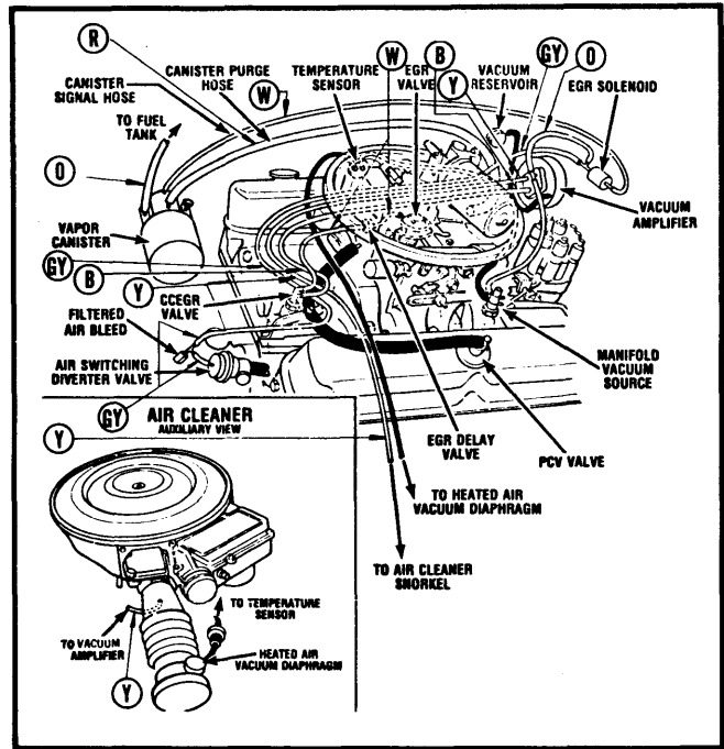
Fig. 8 1982 5.2L (318") V8 EFI; Federal & Calif. (Imperial)
