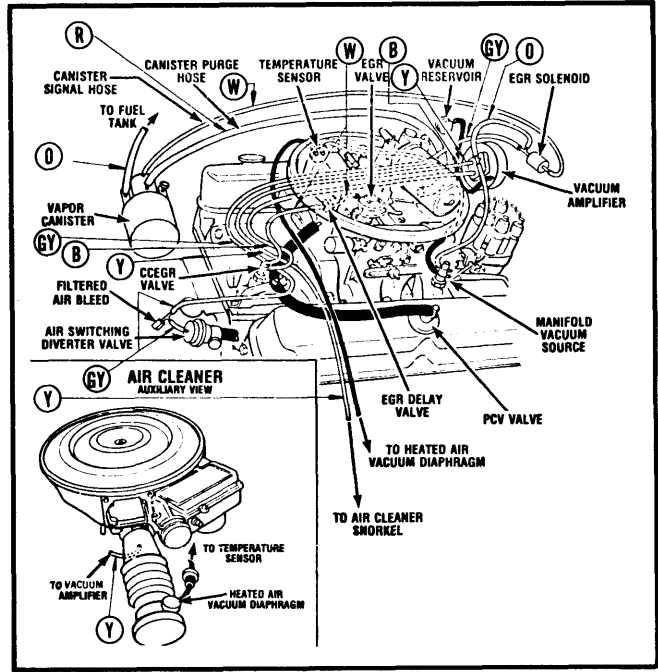
Fig. 6 1981 5.2L (318") V8 EFI; Federal & Calif. (Imperial)
