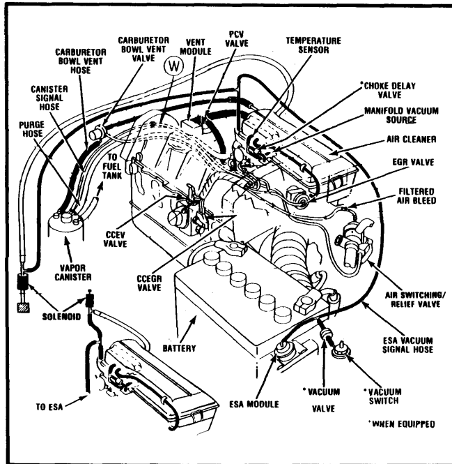
Fig. 1 1981 2.2L (135") 4-Cyl. (Horizon & Omni W/A/C)
