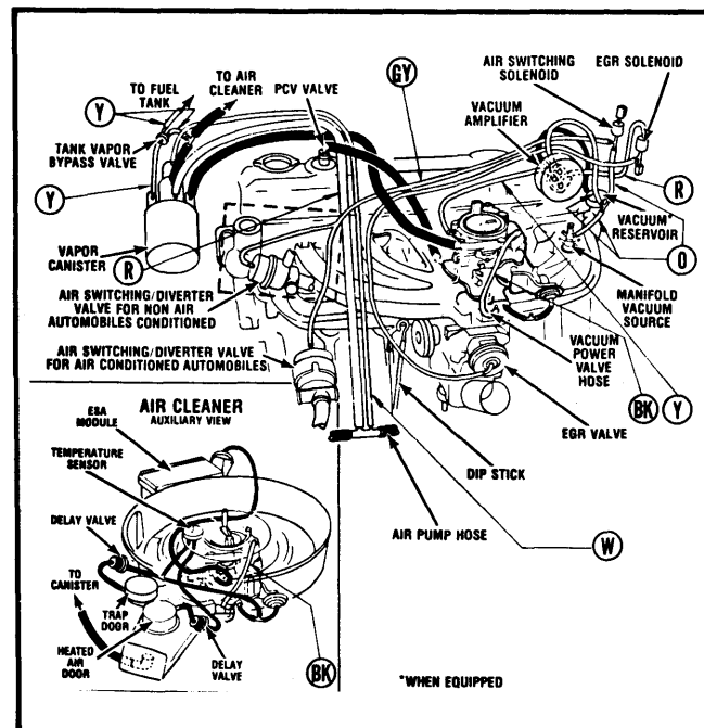
Fig. 3 1981 3.7L (225") 6-Cyl. Calif. (Cordoba, Diplomat, Mirada, New Yorker)
