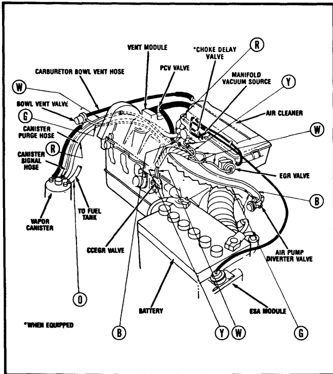
Fig. 3 1982 2.2L (135") 4-Cyl.; Federal (Omni & Rampage)
