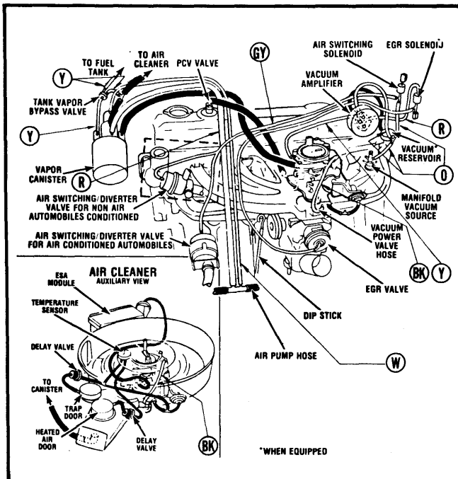
Fig. 5 1982 3.7L (225") 6-Cyl.; Calif. (Cordoba, Diplomat, Mirada, New Yorker)
