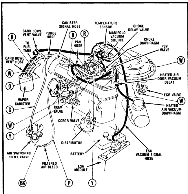
Fig. 1 1982 1.7L (105") 4-Cyl. (Horizon, Omni & Rampage)
