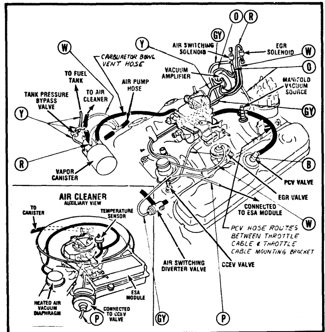
Fig. 6 1982 5.2L (318") V8 2-Bbl.; Federal (Cordoba, Diplomat, Mirada, New Yorker)
