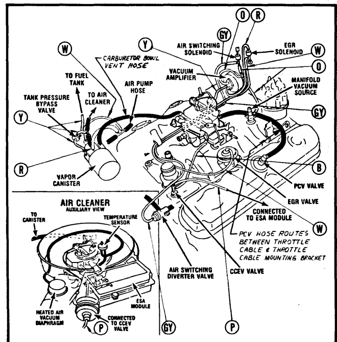
Fig. 4 1981 5.2L (318") V8 2-Bbl.; Federal (Cordoba, Diplomat, Mirada, New Yorker)
