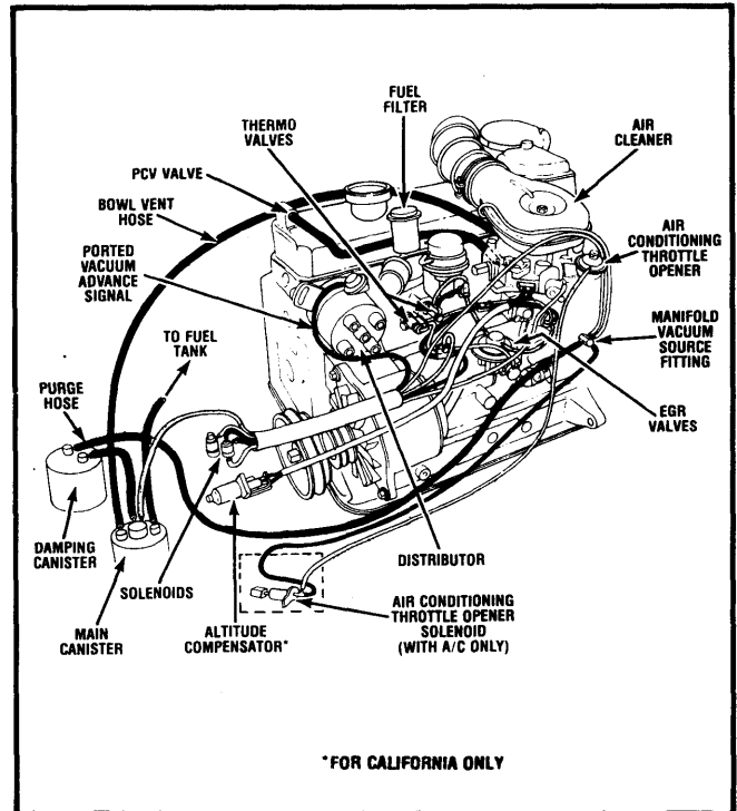
Fig. 4 1982 2.6L (156") 4-Cyl.; Calif.
