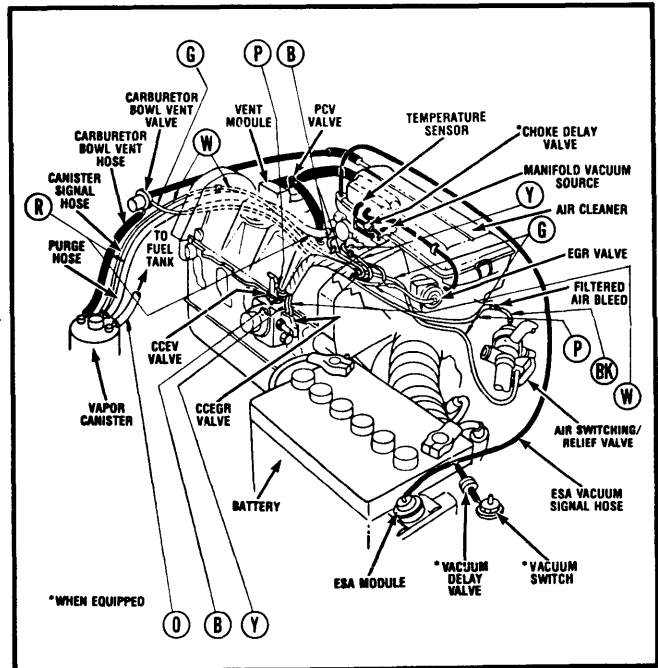
Fig. 2 1982 2.2L (135") 4-Cyl. (Aries, Horizon, LeBaron, Omni, Rampage, Reliant & 400)
