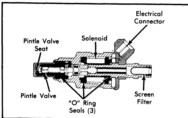
Fig. 4 Cutaway View of Injector Valve
