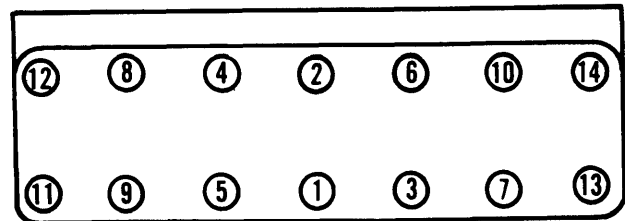
12V71
