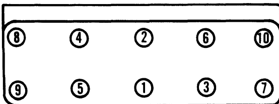
8V71 & 8V92
