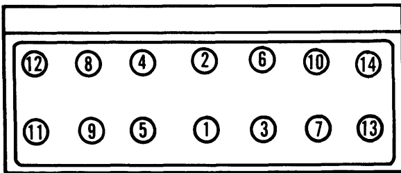
8V71 & 8V92
