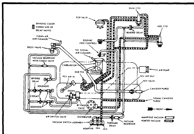
Fig. 11 4.2L 6-Cyl. Calif. All Models Manual Transmission, Heavy Duty Cooling
