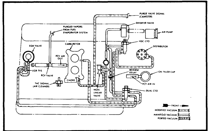
Fig. 20 5.0L V8 Federal "CJ" & Scrambler Automatic Transmission, Heavy Duty Cooling
