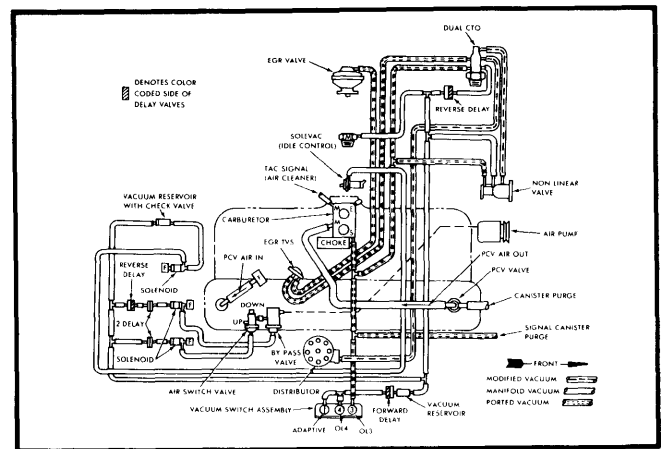
Fig. 12 4.2L 6-Cyl. Calif. All Models Automatic Transmission, Standard Cooling
