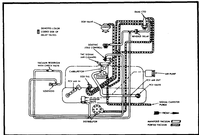
Fig. 16 4.2L 6-Cyl. High Altitude All Models Automatic Transmission
