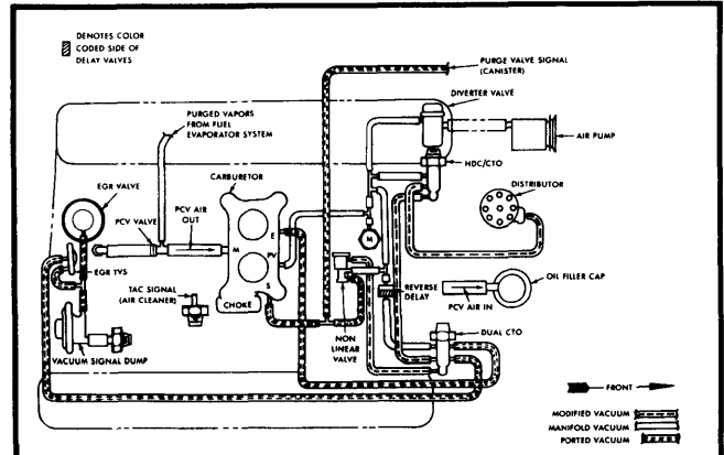
Fig. 24 6.0L Federal Cherokee, Wagoneer & Truck Manual & Automatic Transmission, Heavy Duty Cooling
