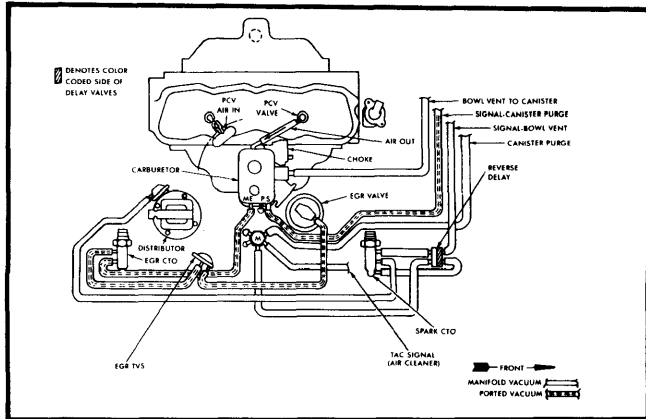
Fig. 3 2.5L 4-Cyl. Federal "CJ" & Scrambler Automatic Transmission, Heavy Duty Cooling
