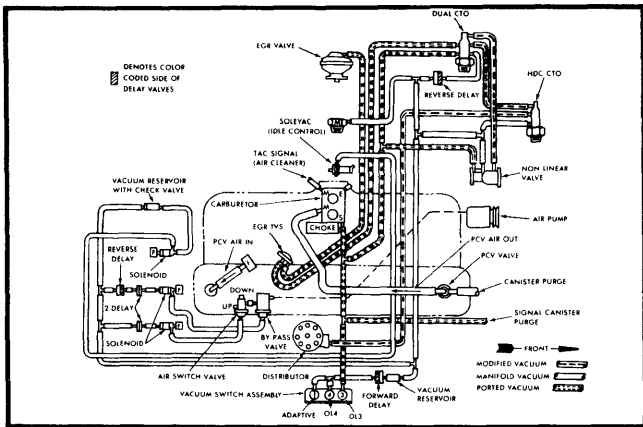
Fig. 13 4.2L 6-Cyl. Calif. All Models Automatic Transmission, Heavy Duty Cooling
