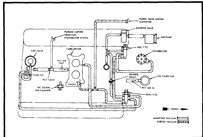
Fig. 18 5.0L V8 Federal "CJ" & Scrambler Manual Transmission, Heavy Duty Cooling
