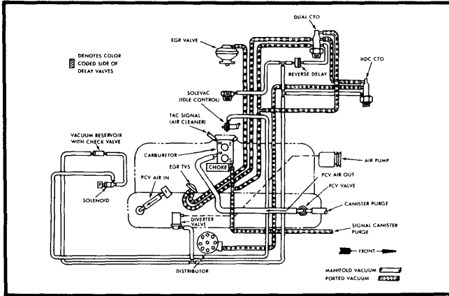
Fig. 7 4.2L 6-Cyl. Federal All Models Manual Transmission, Heavy Duty Cooling
