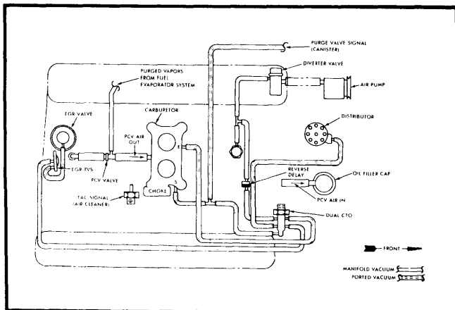
Fig. 17 5.0L V8 Federal "CJ" & Scrambler Manual Transmission, Standard Cooling
