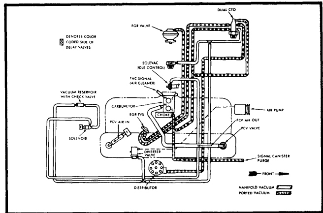
Fig. 14 4.2L 6-Cyl. High Altitude All Models Manual Transmission, Standard Cooling
