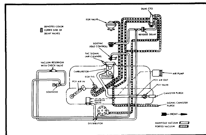
Fig. 6 4.2L 6-Cyl. Federal All Models Manual Transmission, Standard Cooling
