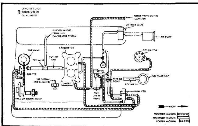
Fig. 23 6.0L V8 Federal Cherokee, Wagoneer & Truck Manual & Automatic Transmission, Standard Cooling
