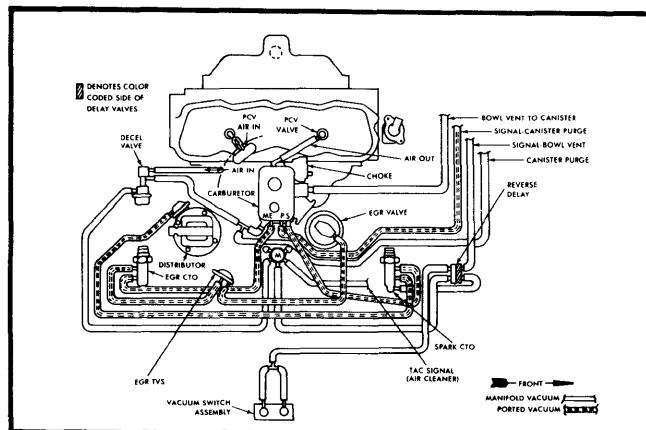
Fig. 5 2.5L 4-Cyl. Calif. CJ-7 Automatic Transmission, Standard & Heavy Duty Cooling
