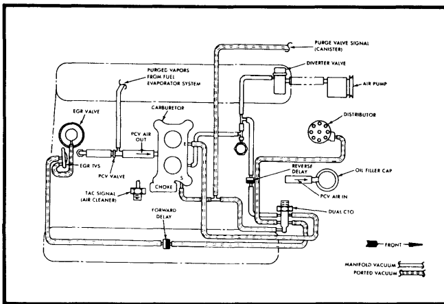
Fig. 21 5.0L V8 High Altitude "CJ" & Scrambler Manual Transmission, Standard Cooling
