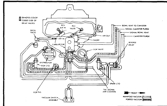
Fig. 4 2.5L 4-Cyl. Calif. "CJ" & Scrambler Manual Transmission, Standard & Heavy Duty Cooling
