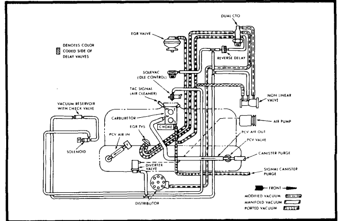
Fig. 8 4.2L 6-Cyl. Federal All Models Automatic Transmission, Standard Cooling
