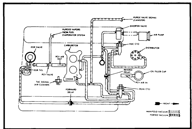
Fig. 22 5.0L V8 High Altitude "CJ" & Scrambler Manual Transmission, Heavy Duty Cooling
