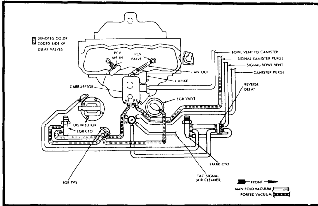
Fig. 1 2.5L 4-Cyl. Federal "CJ" & Scrambler Manual Transmission, Standard & Heavy Duty Cooling
