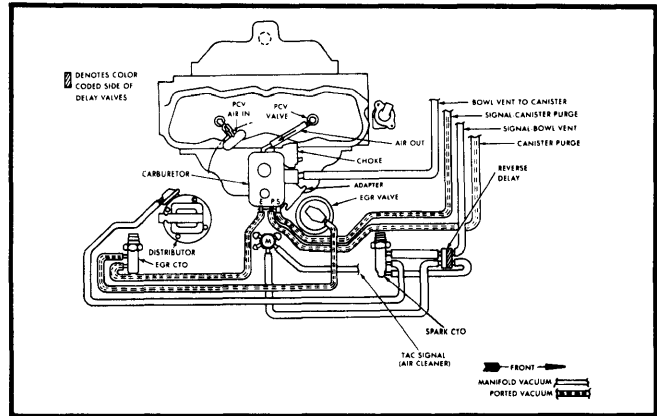
Fig. 2 2.5L 4-Cyl. Federal "CJ" & Scrambler Automatic Transmission, Standard Cooling
