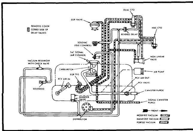
Fig. 9 4.2L 6-Cyl. Federal All Models Automatic Transmission, Heavy Duty Cooling
