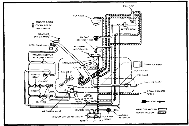
Fig. 10 4.2L 6-Cyl. Calif. All Models Manual Transmission, Standard Cooling
