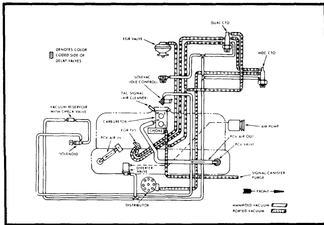
Fig. 15 4.2L 6-Cyl. High Altitude All Models Manual Transmission, Heavy Duty Cooling
