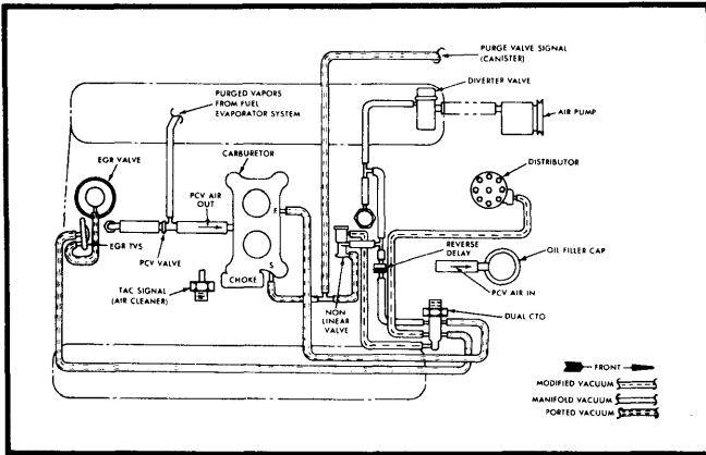
Fig. 19 5.0L V8 Federal "CJ" & Scrambler Automatic Transmission, Standard Cooling
