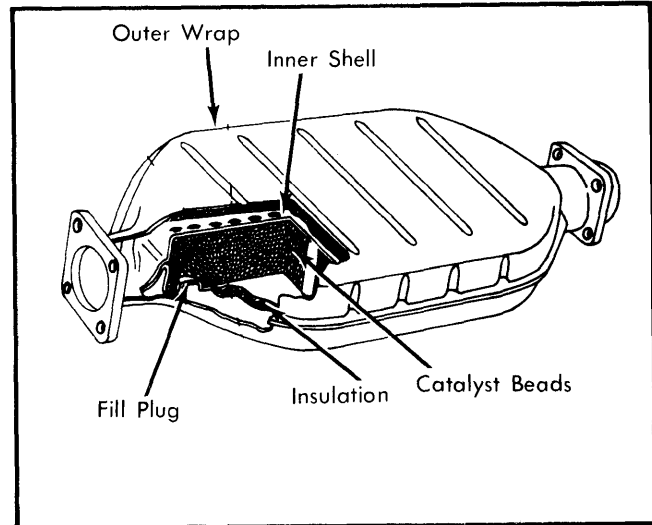
Fig. 2 Cutaway View of Bead-Type Catalytic Converter General Motors and Jeep
