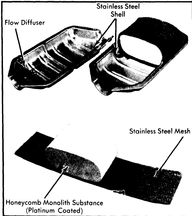
Fig. 1 Cutaway View of Monolithic Catalytic Converter Chrysler Corp. Shown, Ford is Similar
