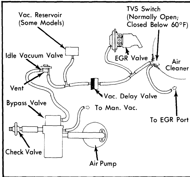
Fig. 6 Schematics of Ford Air Injection System with Idle Vacuum Valve
