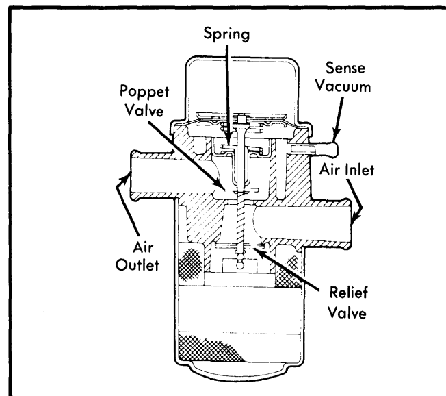
Fig. 3 Typical Diverter Valve Ford & Jeep (Bypass Valve)
