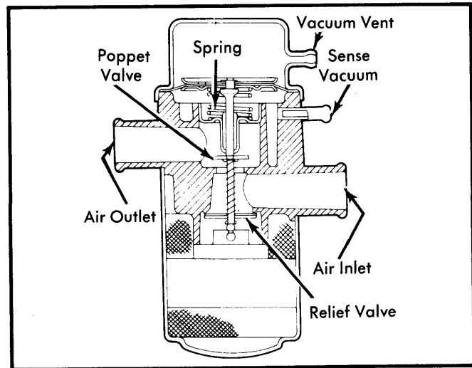
Fig. 4 Ford & Jeep Timed & Vented Bypass Valve
