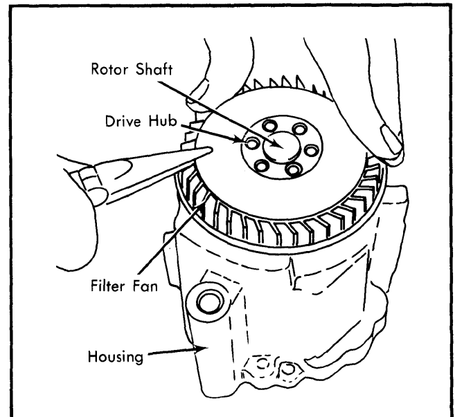
Fig. 7 Removing Centrifugal Fan Filter from Air Injection Pump with Pulley Removed
