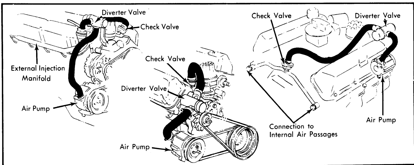
Fig. 5 Typical Air Injection System Installation Configurations
