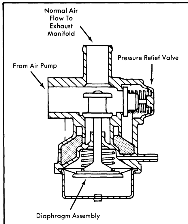
Fig. 2 Typical Diverter Valve Chevrolet, GMC & Chrysler Corp.
