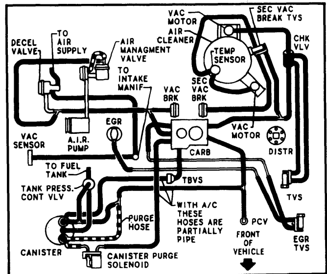
Fig. 6 2.8L (173") V6 Federal Auto. Trans.
