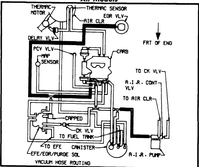
Fig. 9 3.8L (231") V6 Federal Man. Trans.
