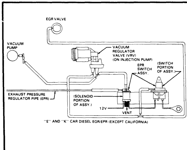
Fig. 27 5.7L (350") Diesel V8 Federal Front Wheel Drive
