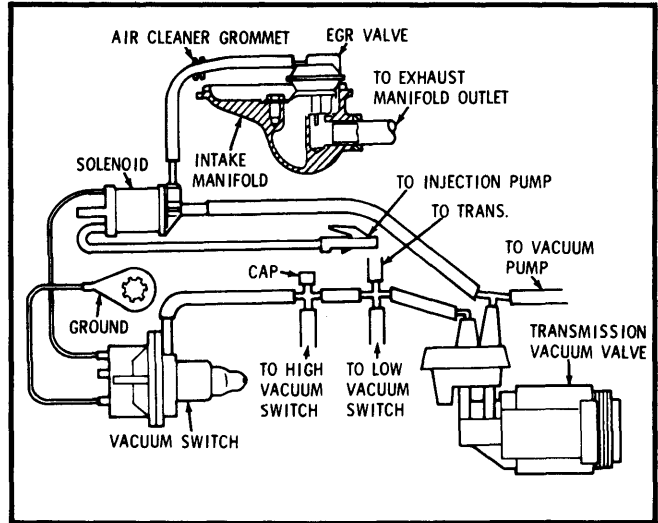
Fig. 29 5.7L (350") Diesel V8 Calif. Rear Wheel Drive (Wagon)
