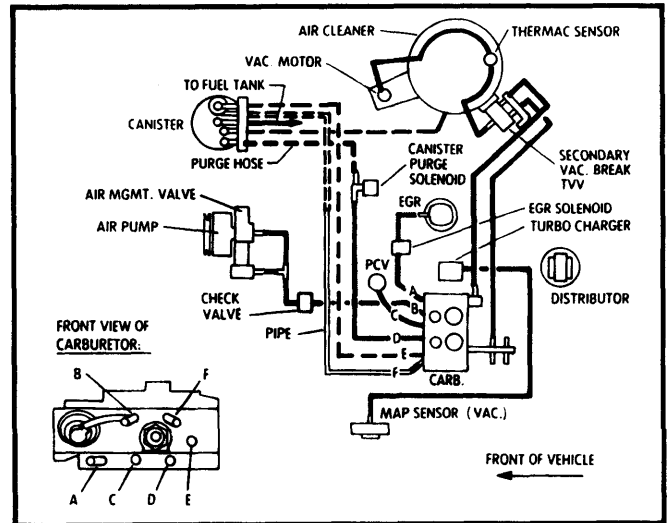
Fig. 22 4.9L (301") Turbo V8 All Models
