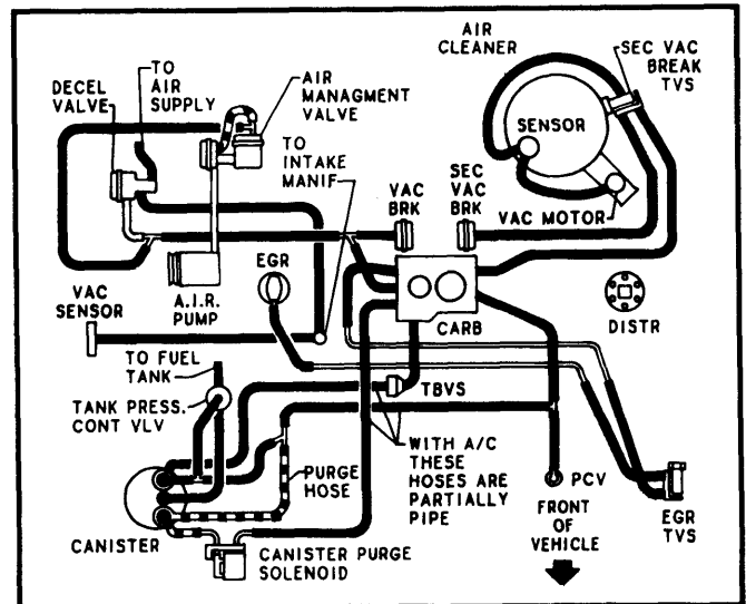
Fig. 5 2.8L (173") V6 Federal Man. Trans.
