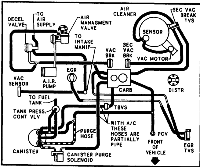
Fig. 7 2.8L (173") V6 Calif. Man. Trans.
