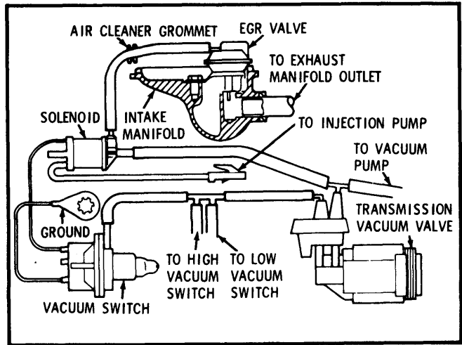
Fig. 28 5.7L (350") Diesel V8 Calif. Rear Wheel Drive (Exc. Wagon)
