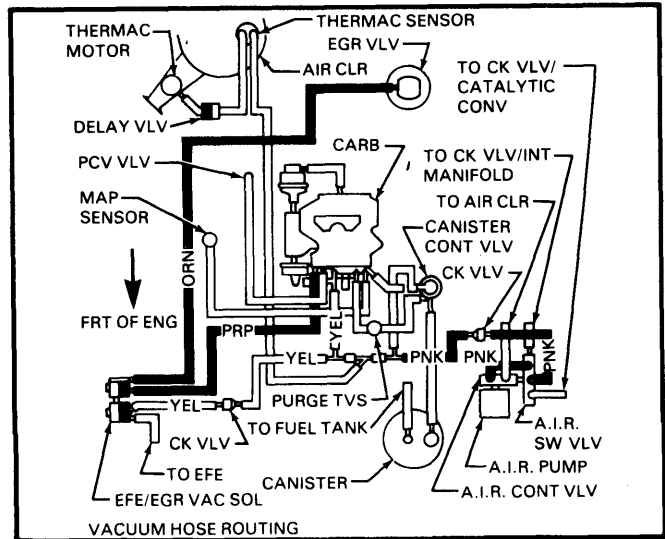
Fig. 17 4.1L (252") V6 Federal Auto. Trans.
