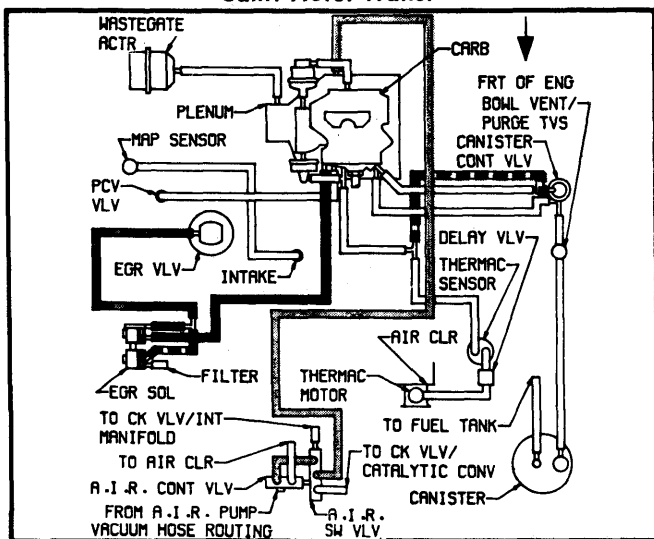
Fig. 15 3.8L (231") Turbo V6 Federal Auto. Trans.
