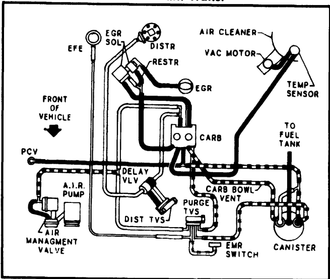
Fig. 8 3.8L (229") V6 All Models
