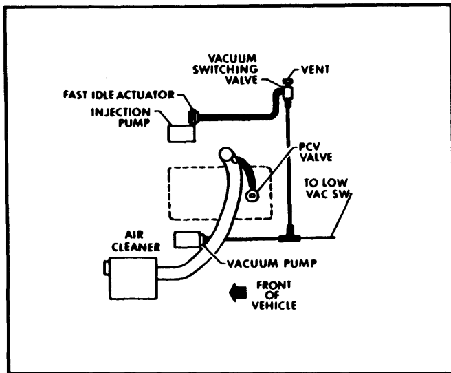
Fig. 2 1.8L (111") 4-Cyl. Diesel All Models
