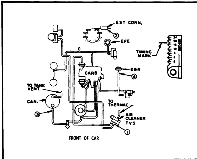
Fig. 19 4.3L (260") V8 All Models
