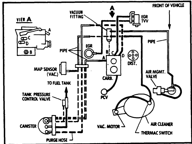
Fig. 4 2.5L (151") 4-Cyl. All Models
