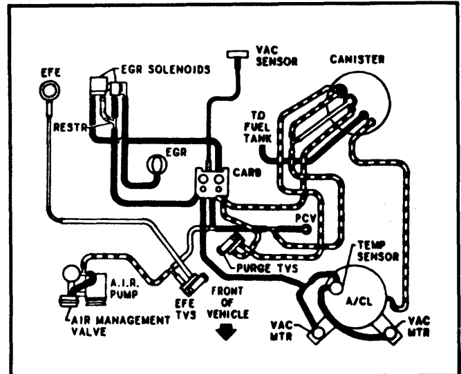
Fig. 24 5.7L (350") V8 Federal
