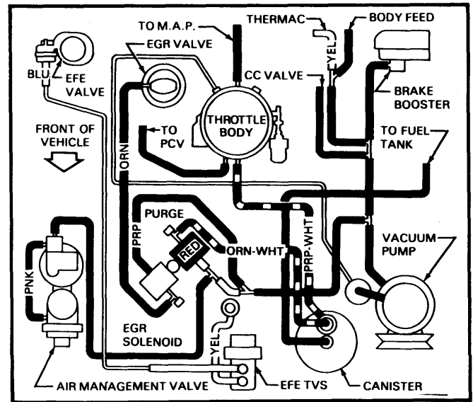
Fig. 32 6.0L (368") V8-6-4 All Front Wheel Drive Models
