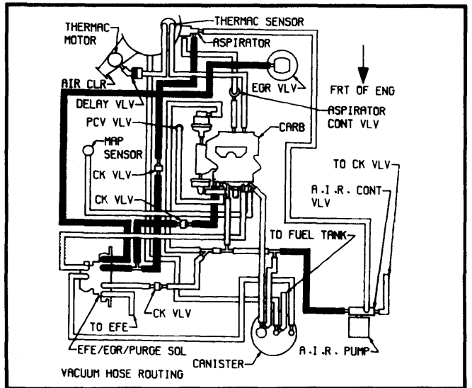
Fig. 11 3.8L (231") V6 Federal Auto. Trans.
