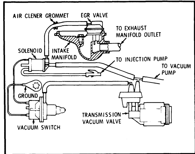
Fig. 30 5.7L (350") Diesel V8 Calif. Front Wheel Drive
