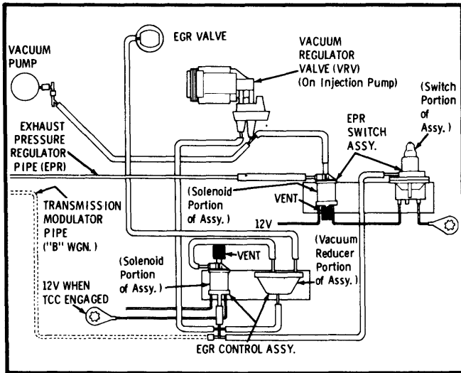
Fig. 26 5.7L (350") Diesel V8 Federal Rear Wheel Drive
