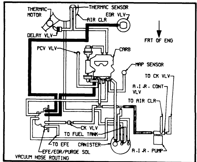
Fig. 10 3.8L (231") V6 Federal Auto. Trans.
