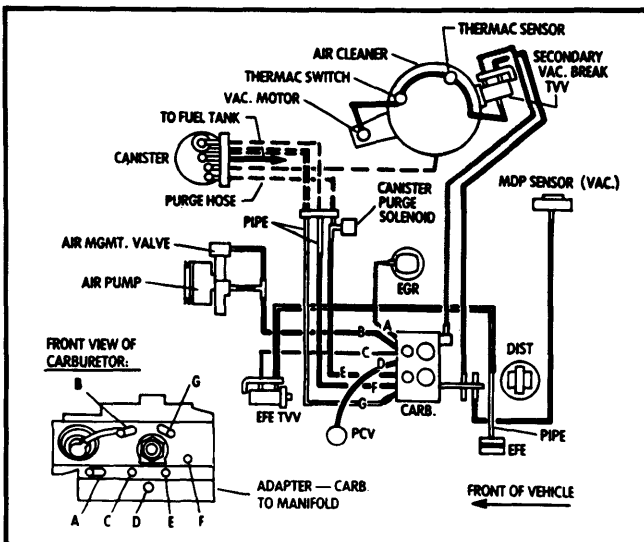
Fig. 21 4.9L (301") V8 All Models
