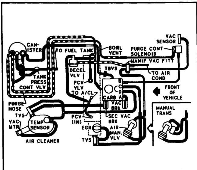
Fig. 3 1.8L (113") 4-Cyl. Gasoline All Models
