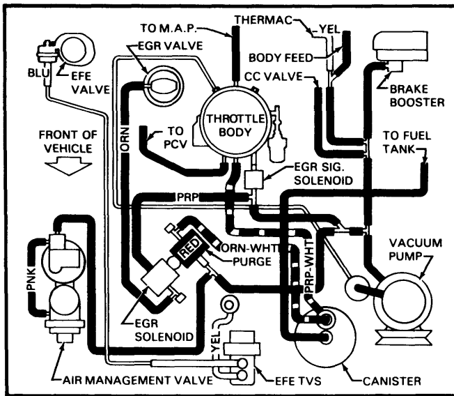
Fig. 31 6.0L (368") V8-6-4 All Rear Wheel Drive Models
