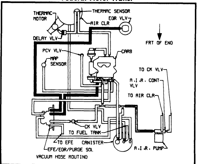
Fig. 12 3.8L (231") V6 Federal Auto. Trans.
