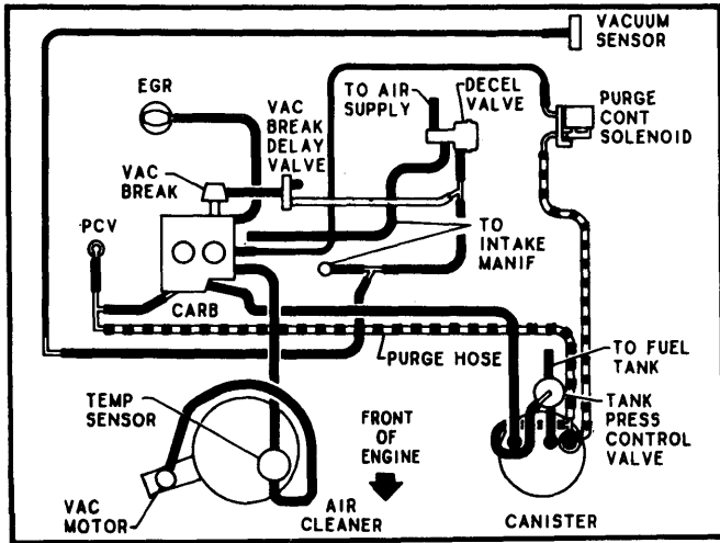
Fig. 1 1.6L (98") 4-Cyl. All Models
