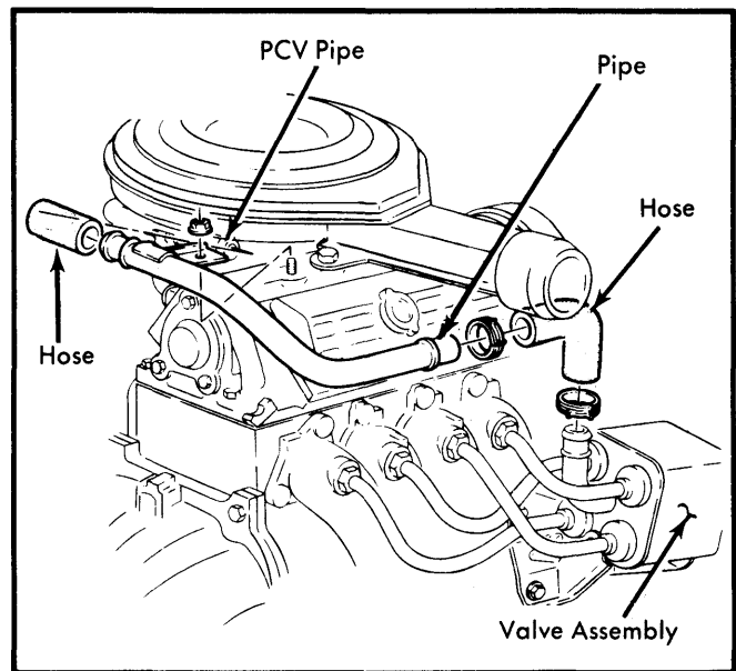
Fig. 2 Showing Typical Installation of PAIR Valve Pipe and Hose (Chevette Shown; Others Similar)
