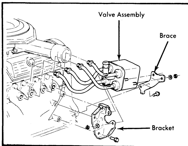
Fig. 1 Pulse Air Valve Mounting Location Shown (Chevette Illustrated; Others Similar)
