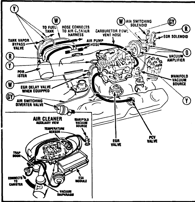
Fig. 5 1981 5.2L (318") V8 4-Bl.; Federal & Calif. (Cordoba, Diplomat, Mirada, New Yorker)
