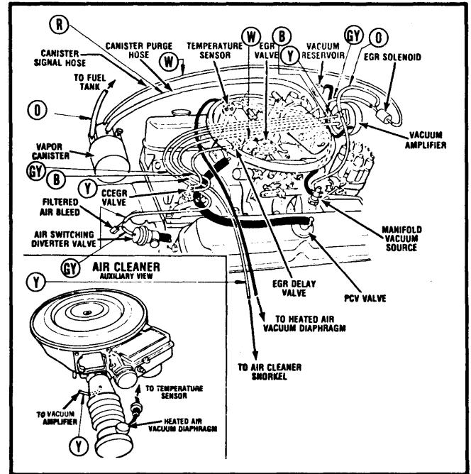
Fig. 6 1981 5.2L (318") V8 EFI; Federal & Calif. (Imperial)
