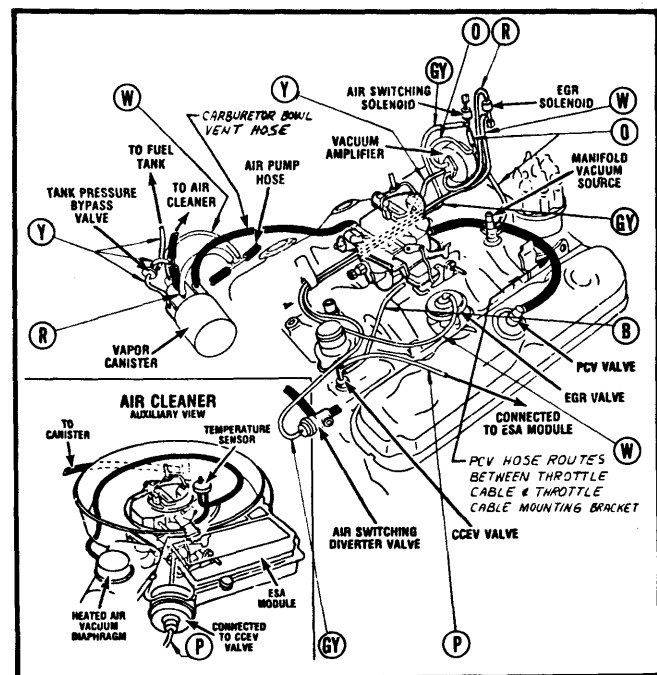
Fig. 4 1981 5.2L (318") V8 2-Bbl.; Federal (Cordoba, Diplomat, Mirada, New Yorker)
