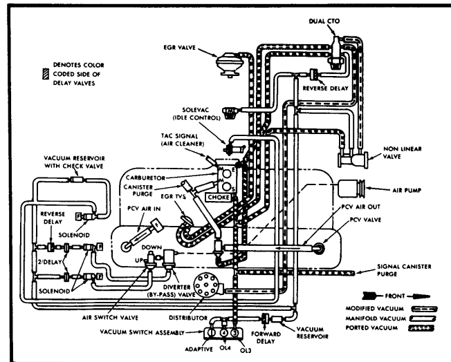
Fig. 9 258" 6 Cyl. Nationwide – Spirit and Concord (All Models)
