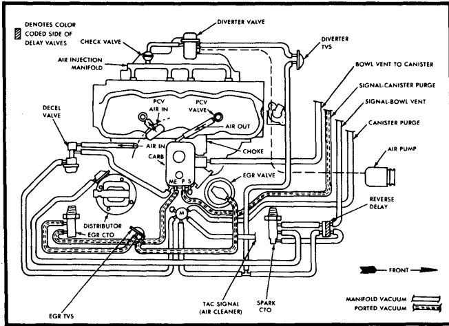
Fig. 1 151" 4 Cyl. Federal – Concord and Spirit (All Except Auto. Trans. with A/C)
