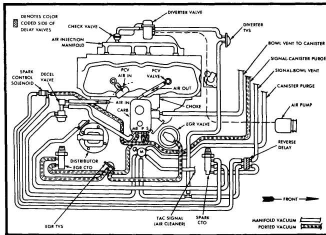
Fig. 2 151" 4 Cyl. Federal – Concord and Spirit (Auto. Trans. with A/C)
