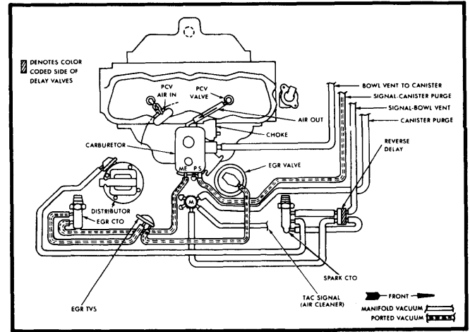
Fig. 5 151" 4 Cyl. Federal – Eagle (Without A/C)
