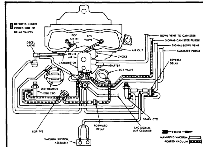
Fig. 3 151" 4 Cyl. Calif. – Concord and Spirit (Man. Trans.)
