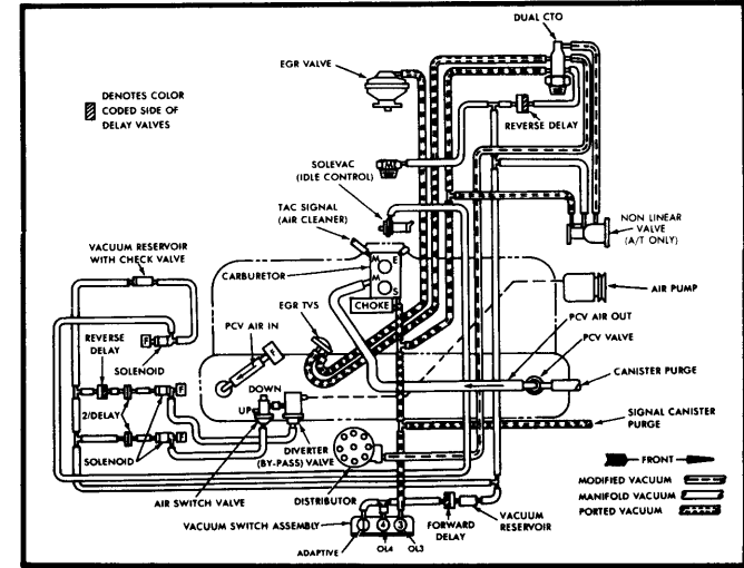
Fig. 11 258" 6 Cyl. Calif. – Eagle (All Models)
