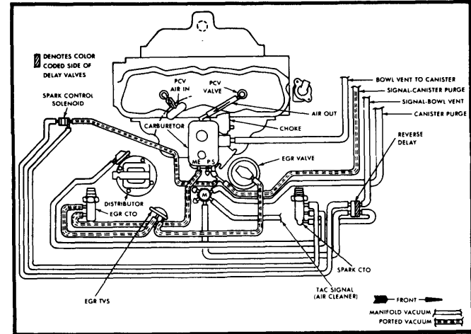
Fig. 6 151" 4 Cyl. Federal – Eagle (With A/C)
