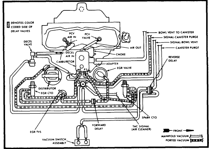
Fig. 4 151" 4 Cyl. Calif. – Concord and Spirit (Auto. Trans.)
