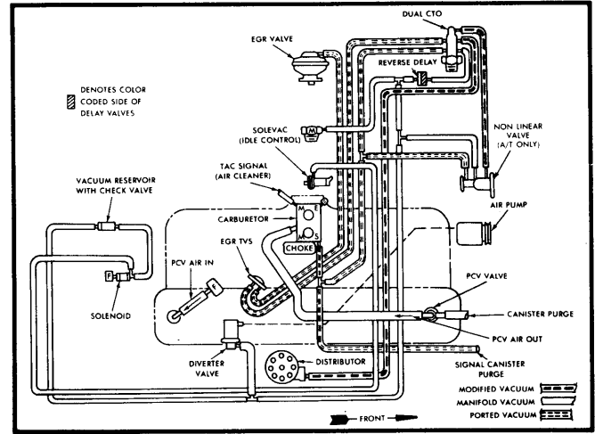
Fig. 10 258" 6 Cyl. Federal – Eagle (All Models)
