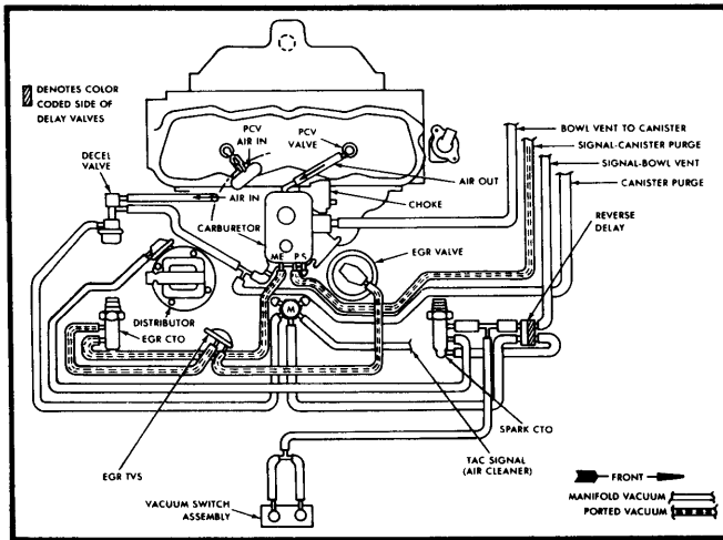
Fig. 7 151" 4 Cyl. Calif. – Eagle (Man. Trans.)
