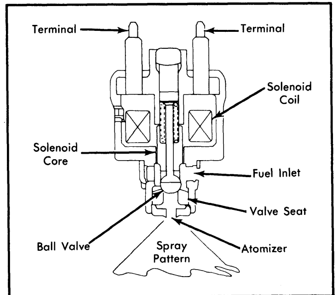
Fig. 2 Sectional View of Injector Valve
