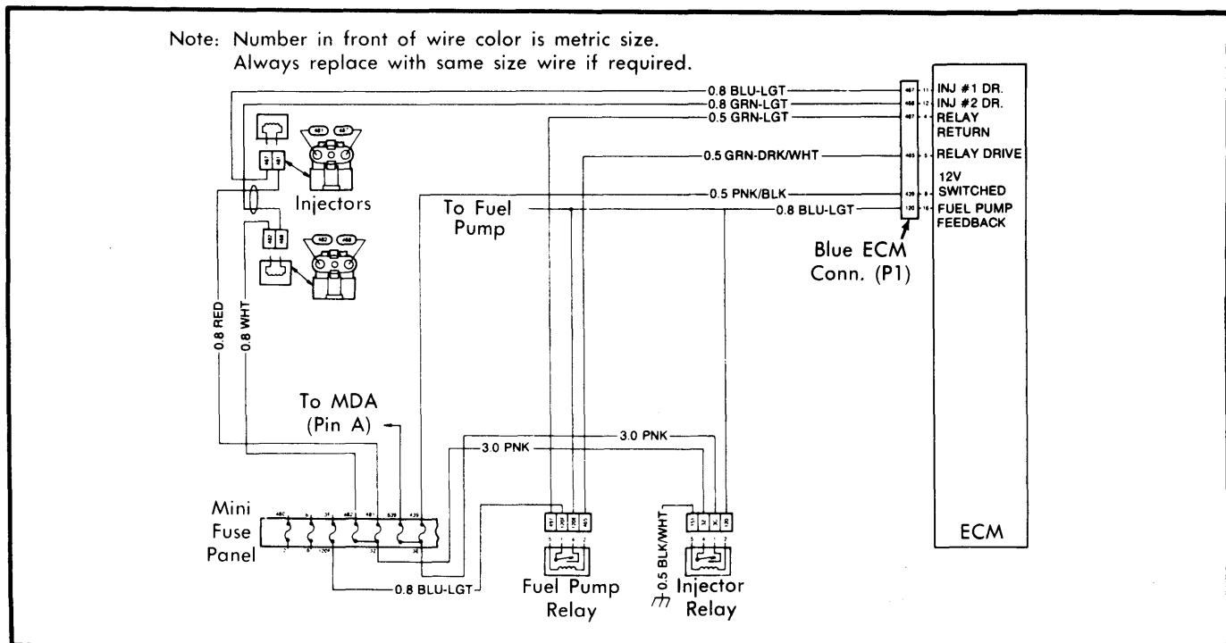
Fig. 6 DFI Fuel Pump and Injector Circuit
