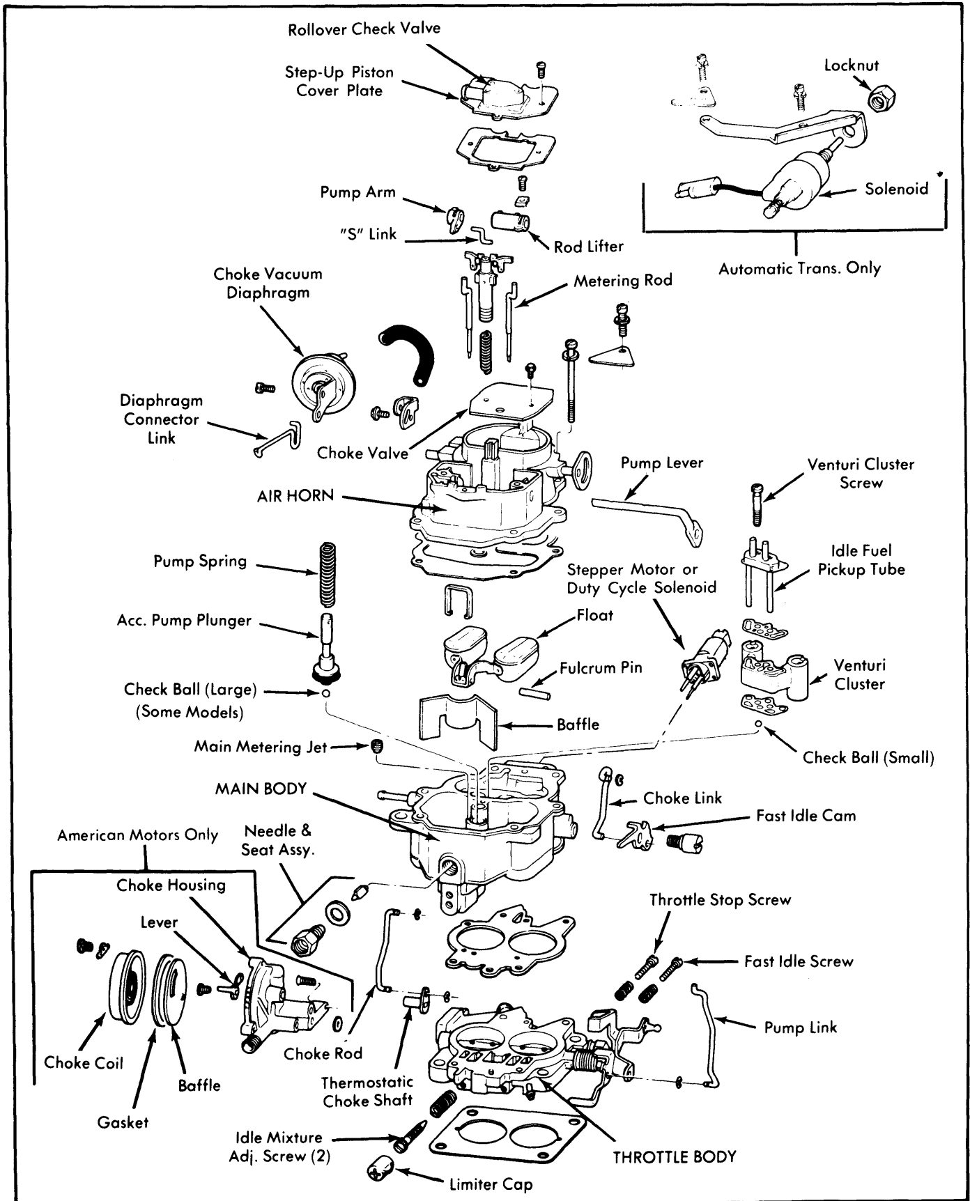
Fig. 10 Exploded View of Carter Model BBD 2-Barrel Carburetor
