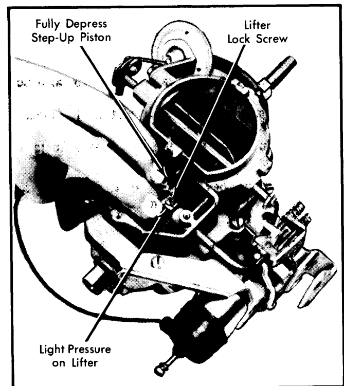
Fig. 5 Adjusting Step-Up Piston
