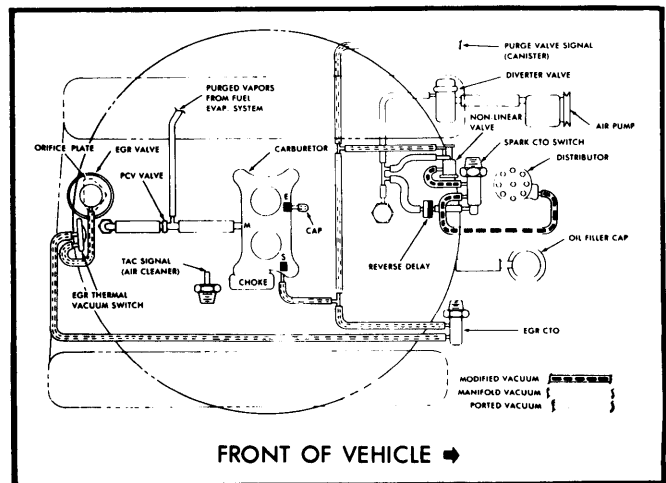
Fig. 12 304" V8 Federal Auto. Trans. with Standard Cooling – CJ-7 Models
