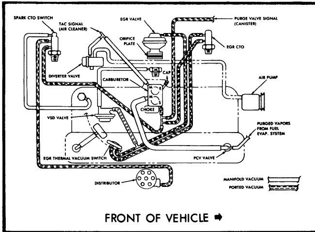
Fig. 7 258" 6 Cyl. Fed. & Calif. Man. Trans. with Standard Cooling – All Except CJ Models
