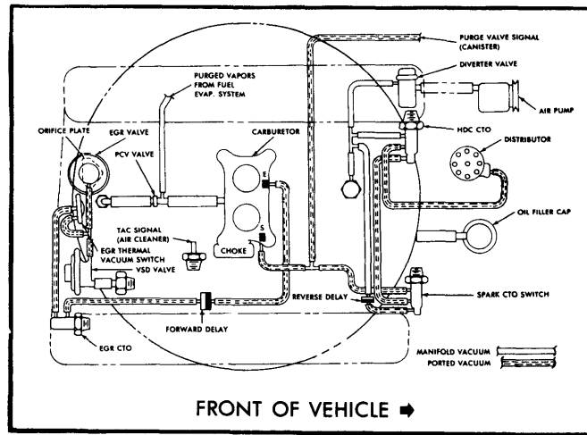
Fig. 21 360" V8 Fed. & Calif. Auto. Trans. with Heavy Duty Cooling - All Except CJ Models
