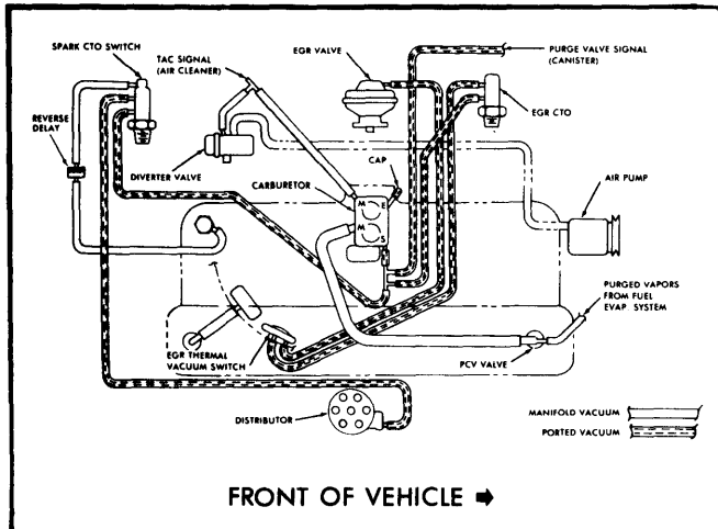
Fig. 3 258" 6 Cyl. Fed. & Calif. Man. Trans. with Standard Cooling – CJ Models
