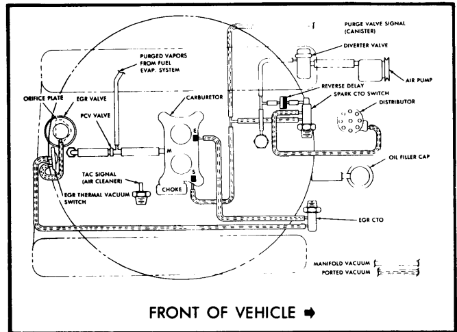
Fig. 10 304" V8 Fed. & High Alt. Man. Trans. with Standard Cooling – CJ Models
