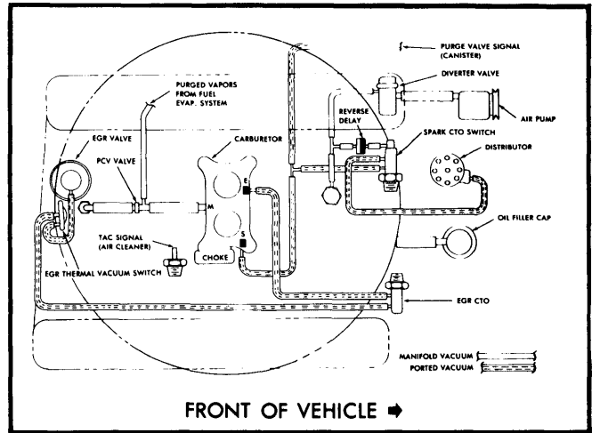
Fig. 20 360" V8 Fed. & Calif. Auto. Trans. with Standard Cooling - All Exc. CJ & J-20 Models
