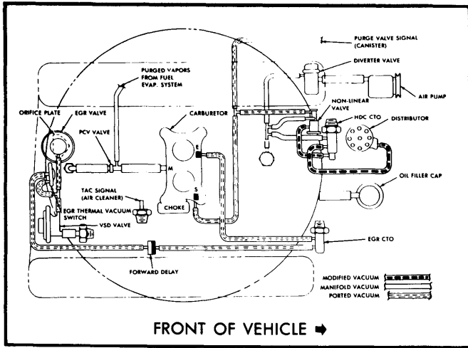
Fig. 19 360" V8 Federal Man. Trans. with Heavy Duty Cooling - J-20 Models
