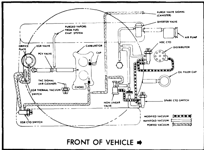
Fig. 13 304" V8 Federal Auto. Trans. with Heavy Duty Cooling - CJ-7 Models
