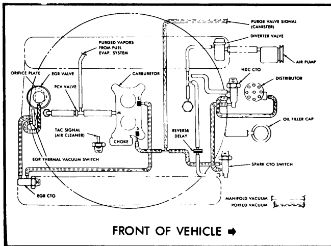
Fig. 11 304" V8 Fed. & High Alt. Man. Trans. with Heavy Duty Cooling – CJ Models
