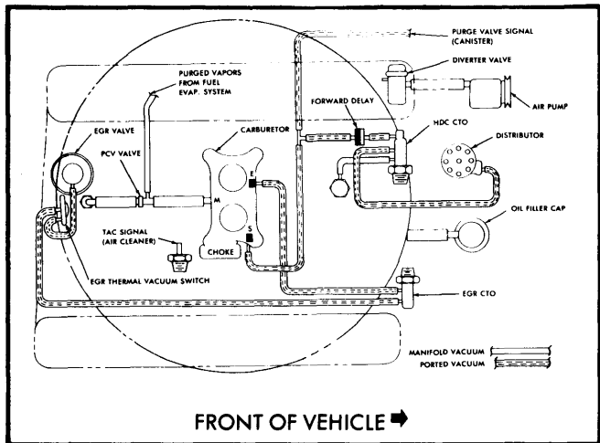
Fig. 14 304" V8 Calif. Man. Trans. with Heavy Duty Cooling - CJ-7 Models
