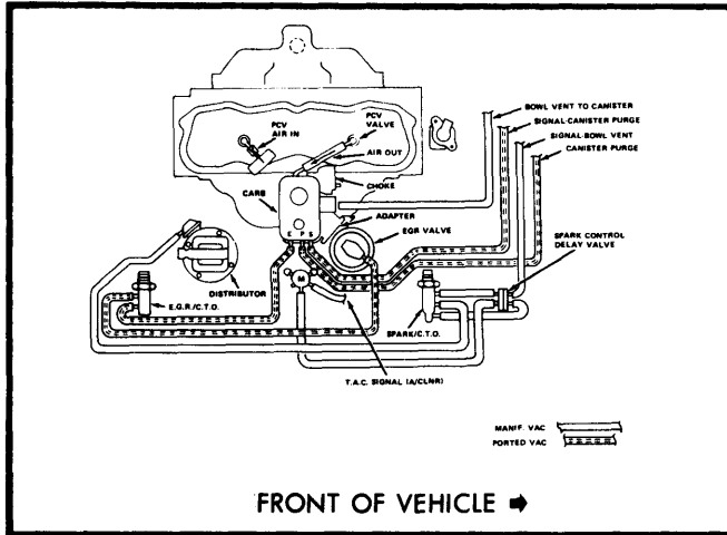
Fig. 1 151" 4 Cyl. Federal CJ Models
