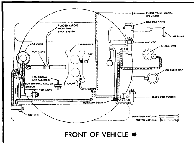
Fig. 15 304" V8 Calif. Auto. Trans. with Heavy Duty Cooling - CJ-7 Models
