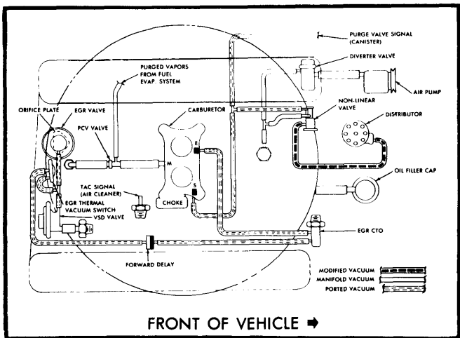
Fig. 18 360" V8 Federal Man. Trans. with Standard Cooling - J-20 Models
