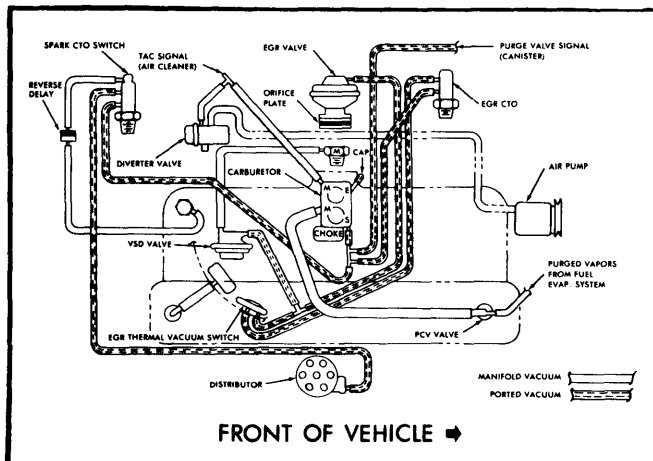
Fig. 3 258" 6 Cyl. Fed. & Calif. Man. Trans. with Standard Cooling – CJ Models
