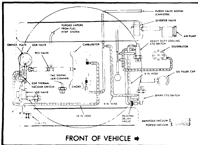
Fig. 17 360" V8 Federal Man. Trans. with Heavy Duty Cooling - Cherokee & J-10 Models
