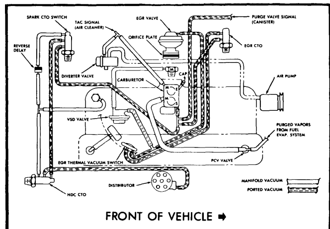
Fig. 6 258" 6 Cyl. Fed. & Calif. Auto. Trans. with Heavy Duty Cooling – CJ-7 Models; and Fed. Man. Trans. with Heavy Duty Cooling – Wagoneer, Cherokee and J-10 Models
