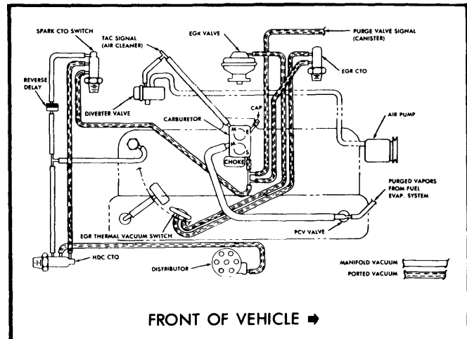
Fig. 4 258" 6 Cyl. Fed. & Calif. Man. Trans. with Standard or Heavy Duty Cooling – CJ Models
