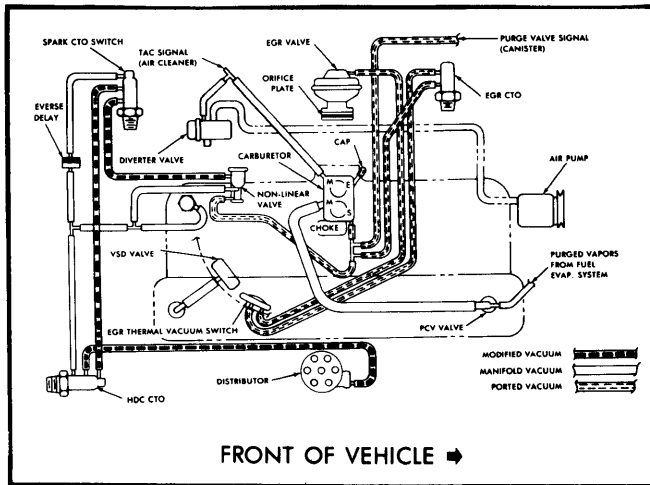
Fig. 9 258" 6 Cyl. Federal Auto. Trans. with Heavy Duty Cooling – All Except CJ Models
