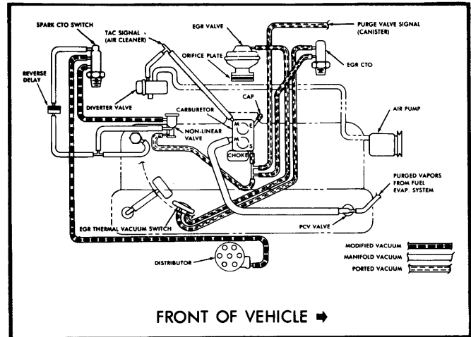
Fig. 8 258" 6 Cyl. Fed. & Calif. Auto. Trans. with Standard Cooling – All Except CJ Models
