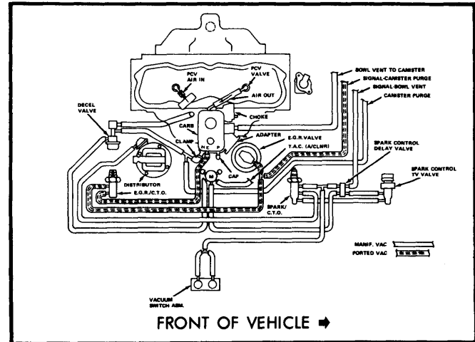
Fig. 2 151" 4 Cyl. California CJ Models
