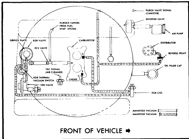
Fig. 16 360" V8 Federal Man. Trans. with Standard Cooling - Cherokee & J-10 Models
