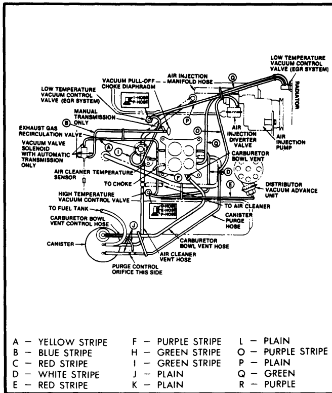
Fig. 9 345" V8 California Emissions With Air Conditioning
