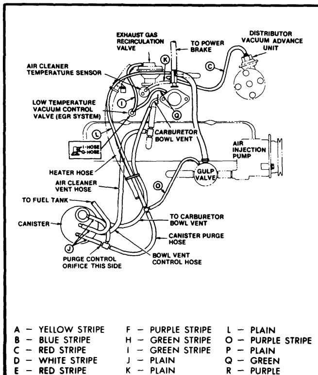
Fig. 2 196" 4 Cyl. California Emissions
