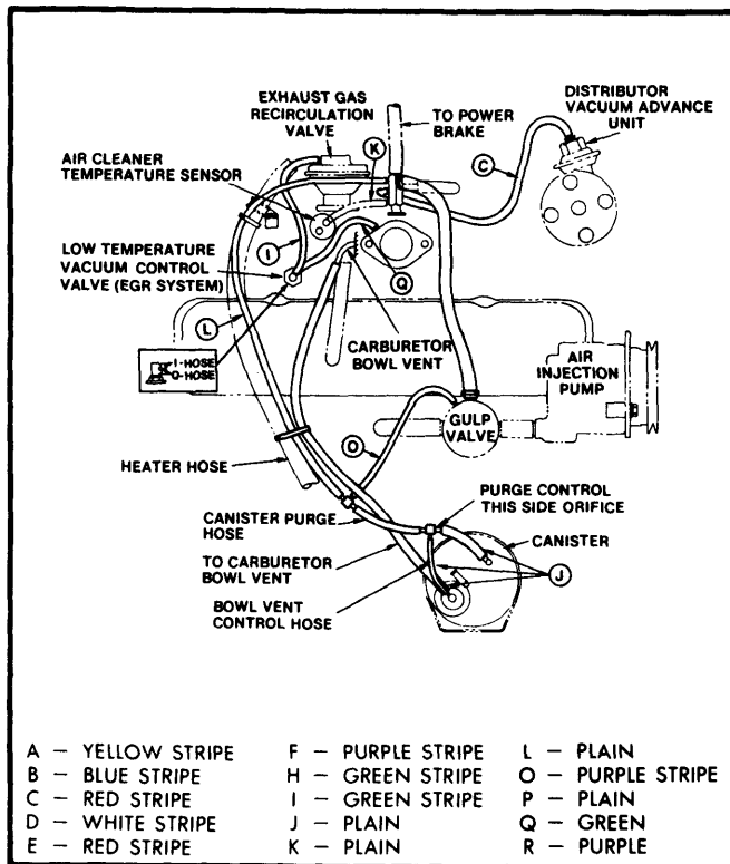
Fig. 1 196" 4 Cyl. Federal Emissions
