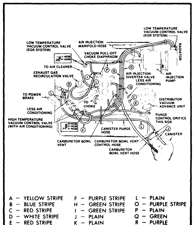
Fig. 4 304" V8 Federal Emissions Automatic Transmission
