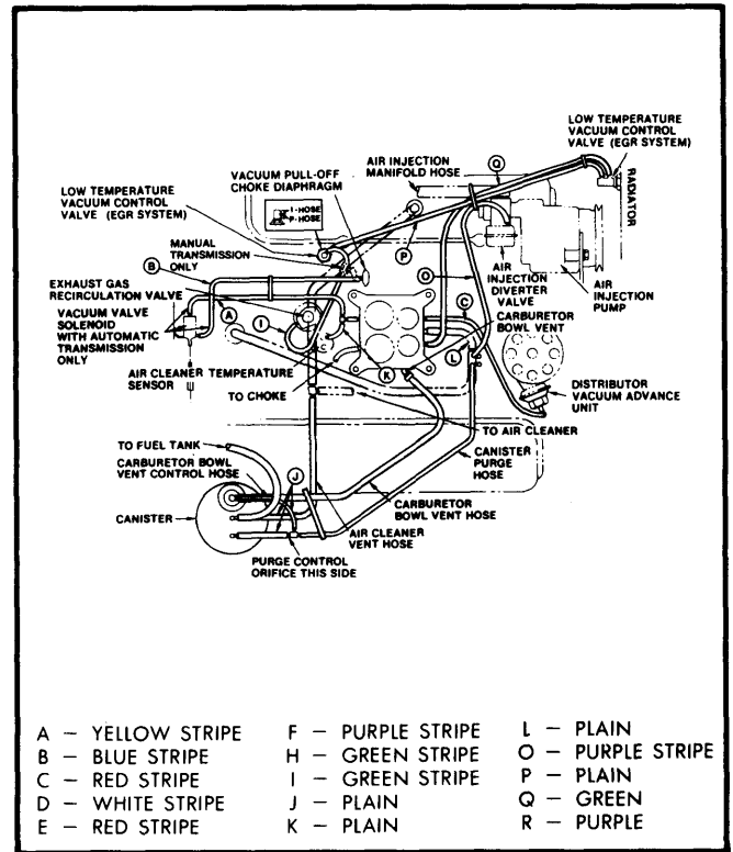
Fig. 10 345" V8 California Emissions Without Air Conditioning
