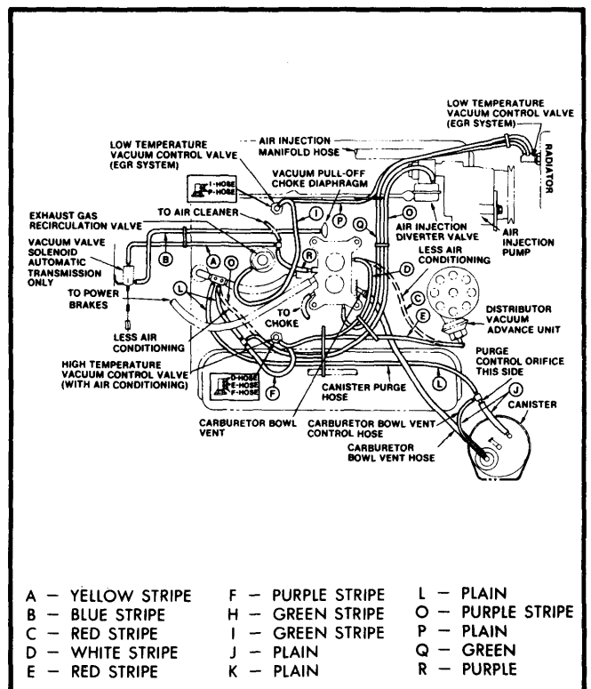
Fig. 3 304" V8 Federal Emissions Manual Transmission
