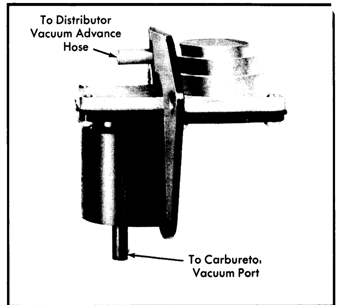
Fig. 2 Close-Up View of OSAC Valve
