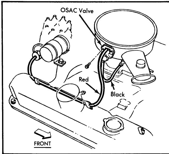
Fig. 1 Typical OSAC Valve Hose Routing (318" & 360" Engines Shown)
