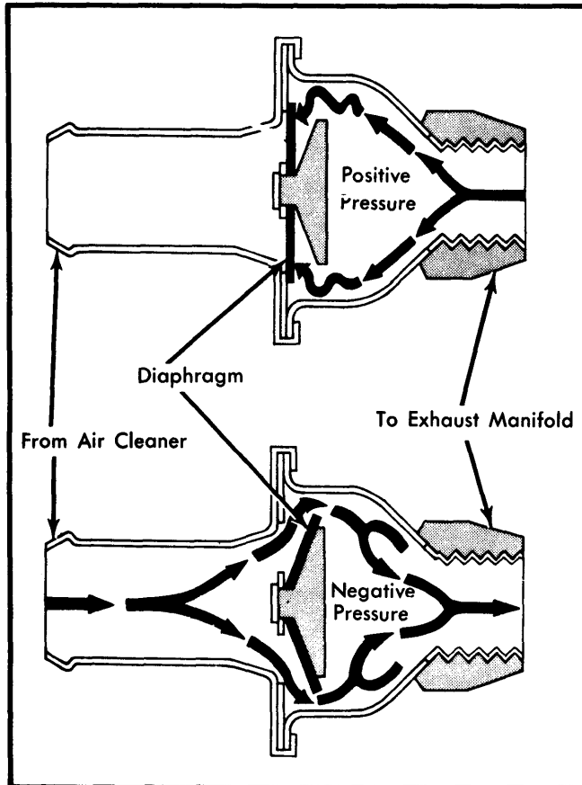
Fig. 1 Aspirator Valve Air Flow
