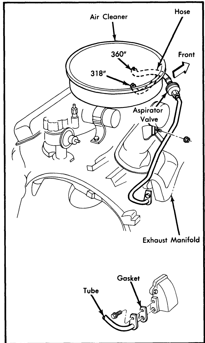
Fig. 2 Aspirator Air System Assembly (V8 Shown - 6 Cylinder Similar)
