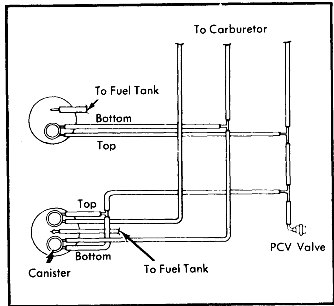
Fig. 1 Vacuum Hose Routing for Two-Canister Evaporative Control System (Models So Equipped)
