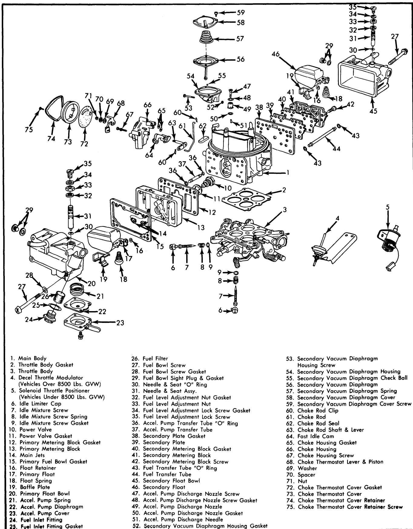
Fig. 7 Exploded View of Holley Model 4180-C 4-Barrel Carburetor
