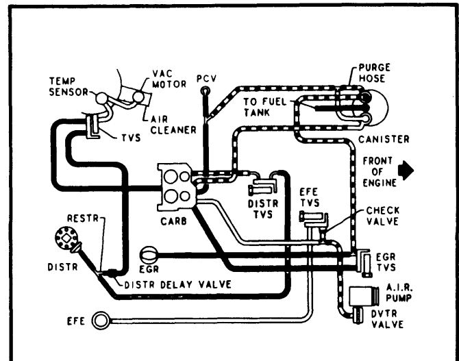
Fig. 48 305" & 350" V8 4-Bbl. Federal Man. Trans.
