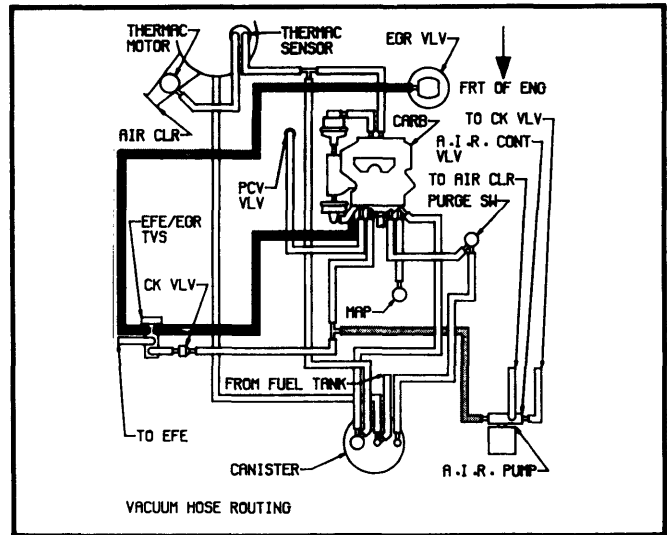
Fig. 28 231" V6 2-Bbl. Calif. Man. Trans.
