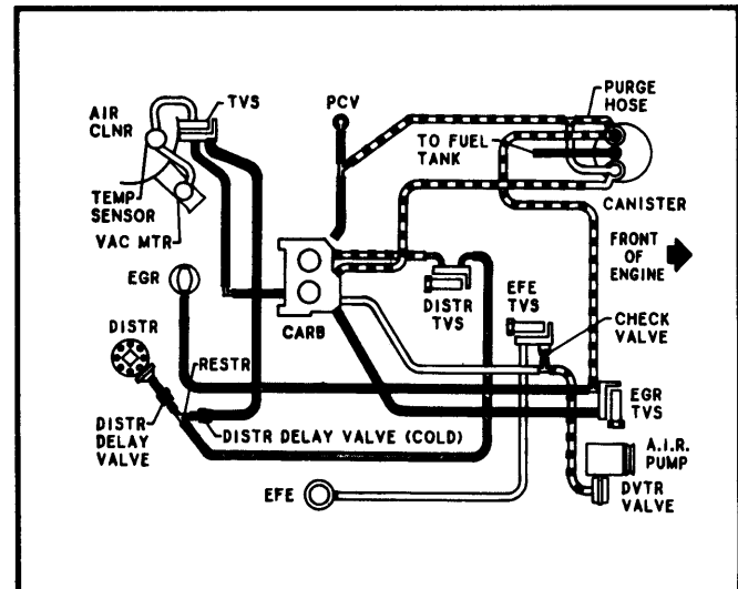
Fig. 41 267" V8 2-Bbl. Federal Auto. Trans.
