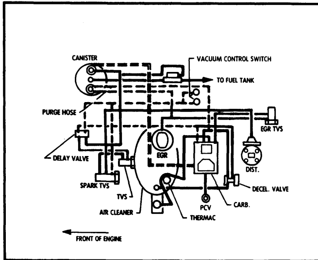
Fig. 7 151" 4 Cyl. 2-Bbl. VIN V Calif. Man. Trans.
