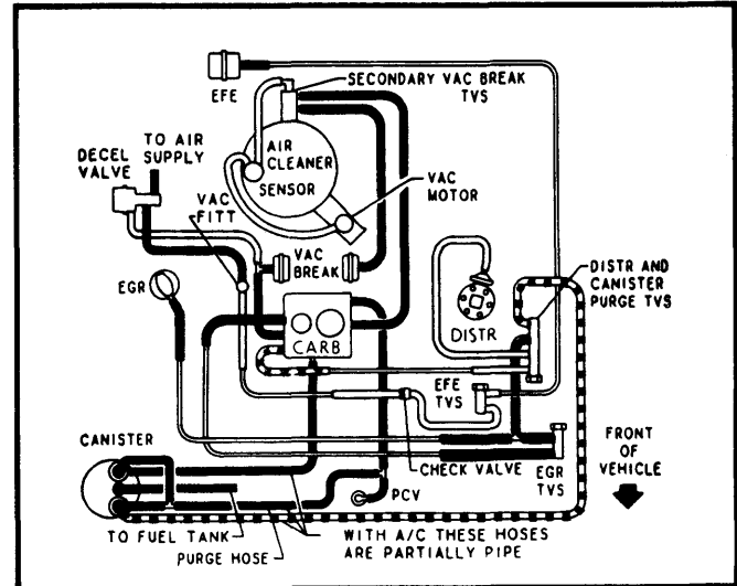
Fig. 17 173" V6 2-Bbl. Federal Auto. Trans.
