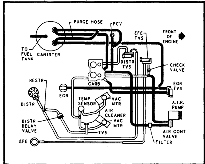
Fig. 53 350" V8 4-Bbl. VIN 6 & 8 Federal Man. Trans.
