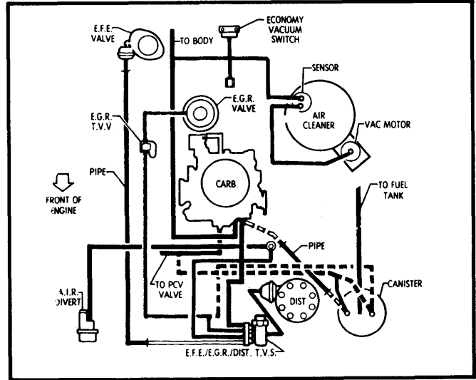
Fig. 64 368" V8 4-Bbl. Federal Auto. Trans.
