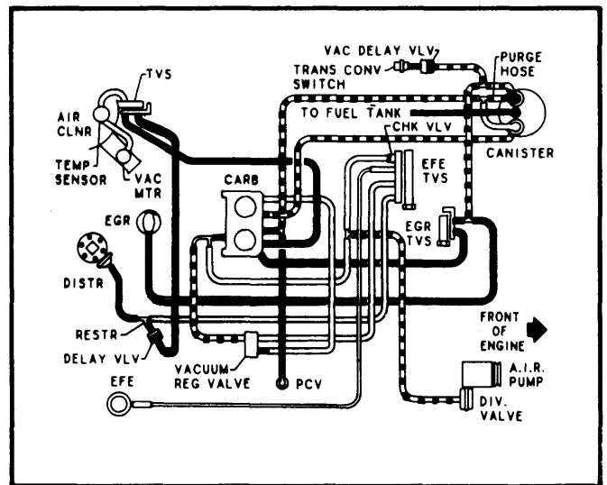
Fig. 22 229" V6 2-Bbl. Federal Auto. Trans.
