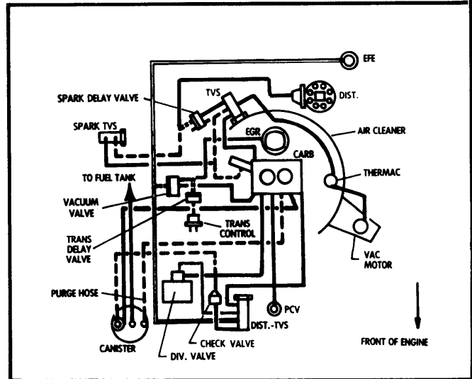
Fig. 40 265" V8 2-Bbl. Federal Auto. Trans.
