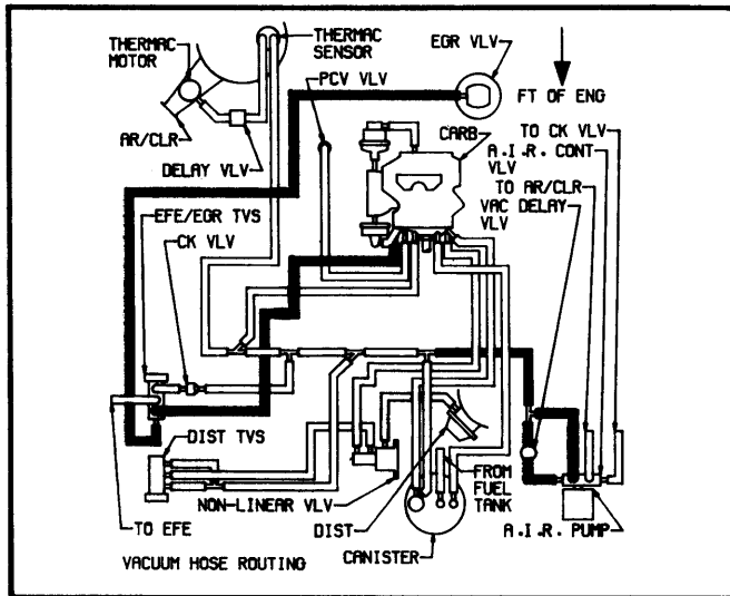
Fig. 37 252" V6 4-Bbl. Federal Auto. Trans.
