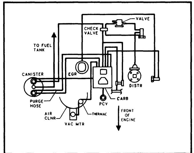
Fig. 10 151" 4 Cyl. 2-Bbl. VIN 5 Federal Man. Trans.
