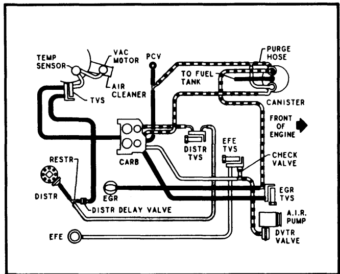
Fig. 52 305" & 350" V8 4-Bbl. (VIN H & L) Federal Auto. Trans.
