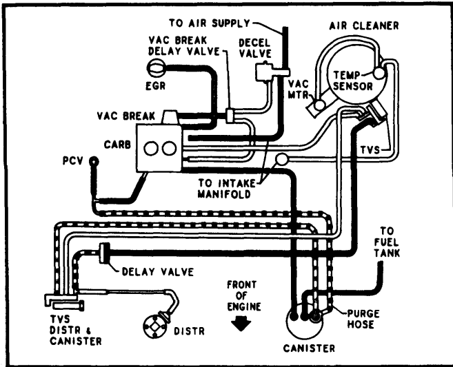
Fig. 2 98" 4 Cyl. 2-Bbl. Federal
