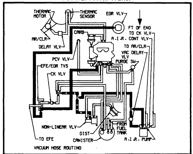
Fig. 23 231" V6 2-Bbl. Federal Man. Trans.
