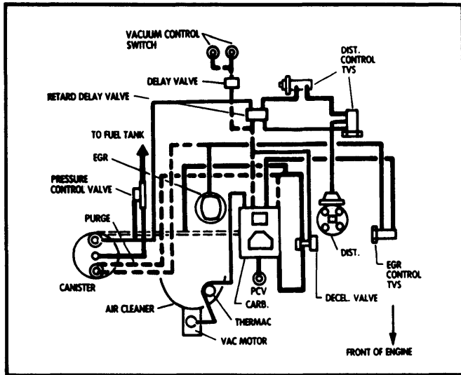
Fig. 13 151" 4 Cyl. 2-Bbl. VIN 5 Calif. Man. Trans.
