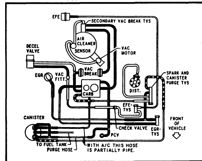
Fig. 18 173" V6 2-Bbl. Federal Auto. Trans.
