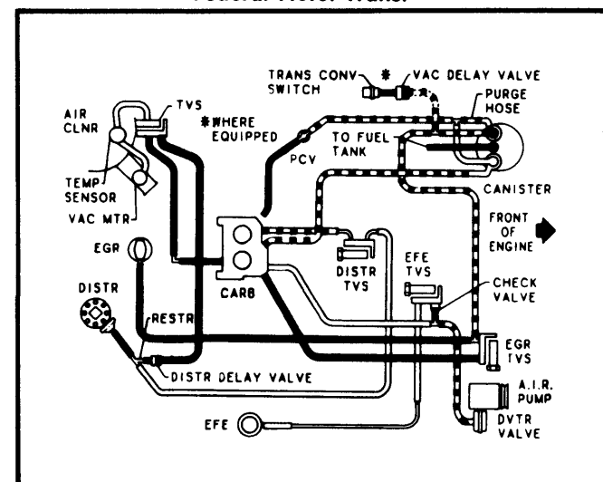
Fig. 42 267" V8 2-Bbl. Federal Auto. Trans.
