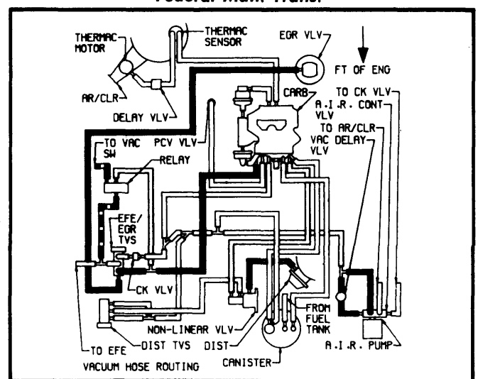
Fig. 24 231" V6 2-Bbl. Federal Auto. Trans.
