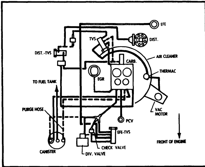
Fig. 43 301" V8 4-Bbl. Federal Auto. Trans.
