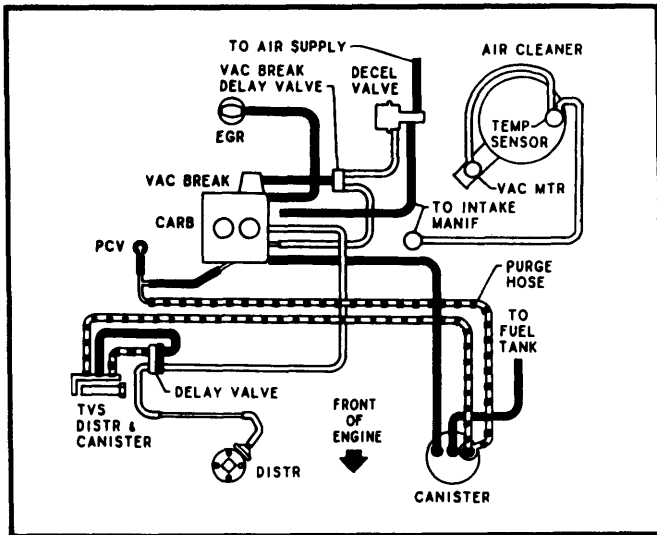
Fig. 1 98" 4 Cyl. 2-Bbl. Federal
