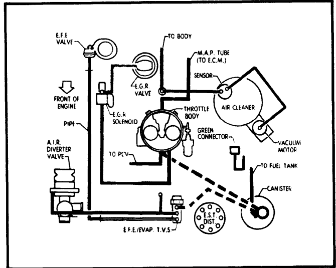
Fig. 63 368" V8 DEFI Federal Auto. Trans.
