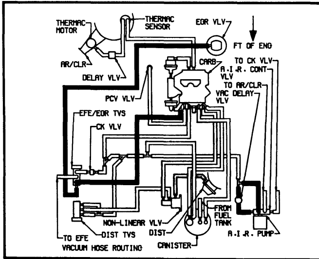
Fig. 26 231" V6 2-Bbl. Federal Auto. Trans.
