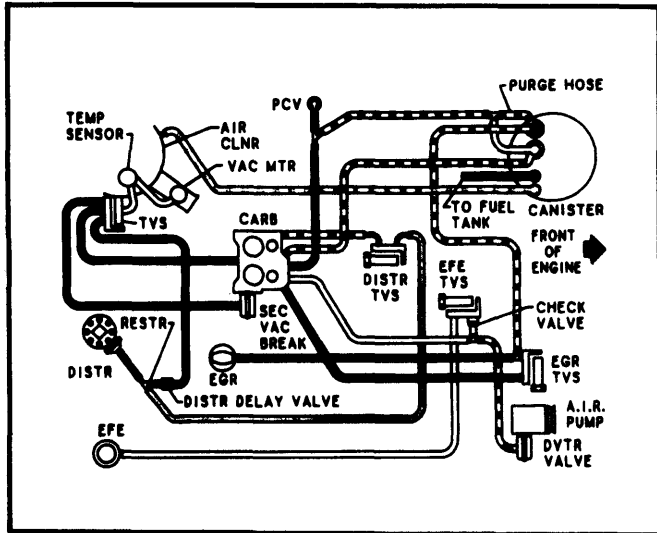
Fig. 50 305" V8 4-Bbl. Calif. Man. Trans.
