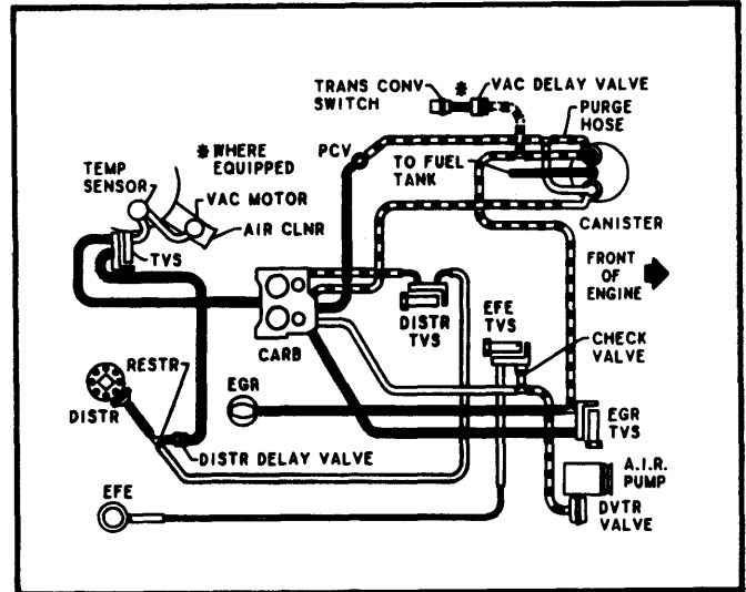
Fig. 46 305" V8 4-Bbl. Federal Auto. Trans.
