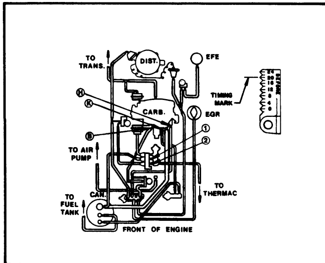
Fig. 38 260" V8 2-Bbl. Federal Auto. Trans.
