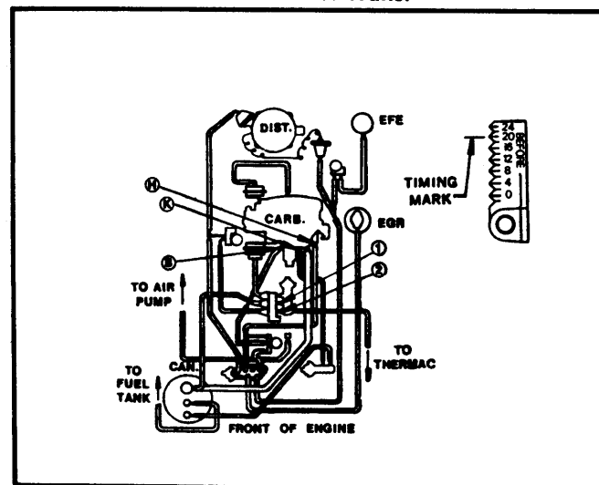
Fig. 39 260" V8 2-Bbl. Federal Auto. Trans.
