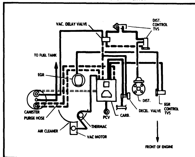
Fig. 9 151" 4 Cyl. 2-Bbl. VIN 5 Federal Man. Trans.
