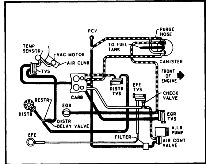
Fig. 47 305" V8 4-Bbl. Federal Man. Trans.
