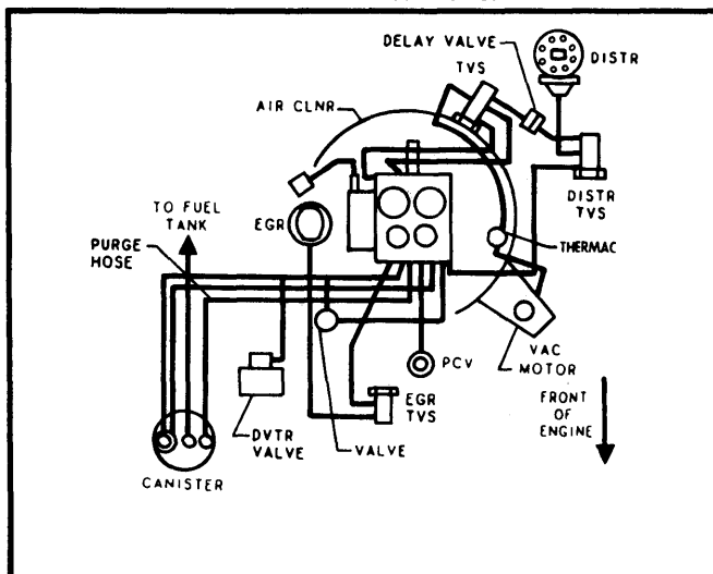
Fig. 45 301" V8 Turbo Federal Auto. Trans.
