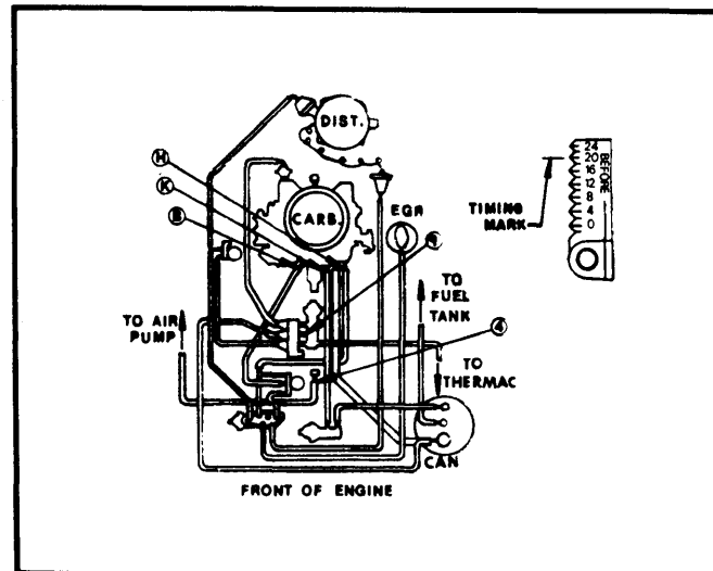
Fig. 51 307" V8 4-Bbl. Federal Auto. Trans.
