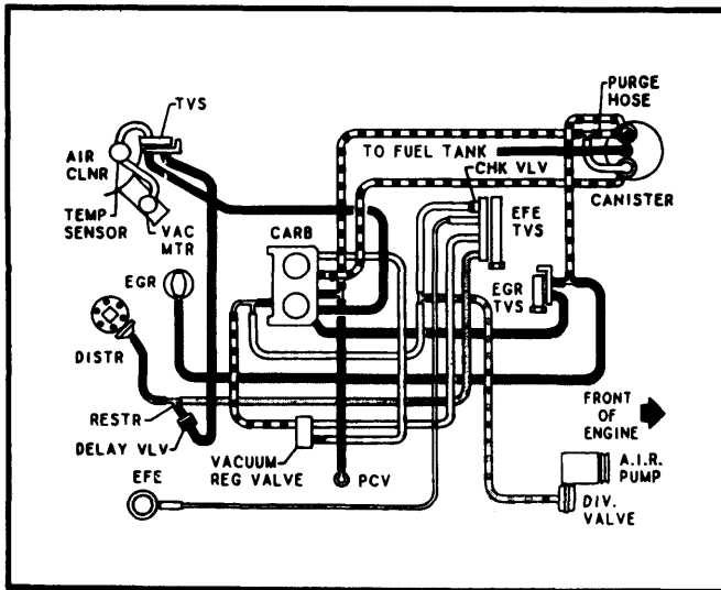
Fig. 20 229" V6 2-Bbl. Federal Man. Trans.
