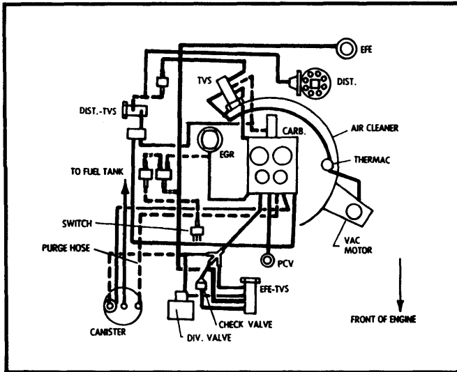
Fig. 44 301" V8 4-Bbl. Federal Auto. Trans.
