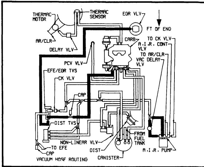
Fig. 25 231" V6 2-Bbl. Federal Auto. Trans.
