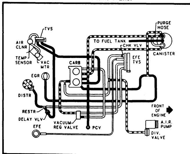
Fig. 21 229" V6 2-Bbl. Federal Auto. Trans.
